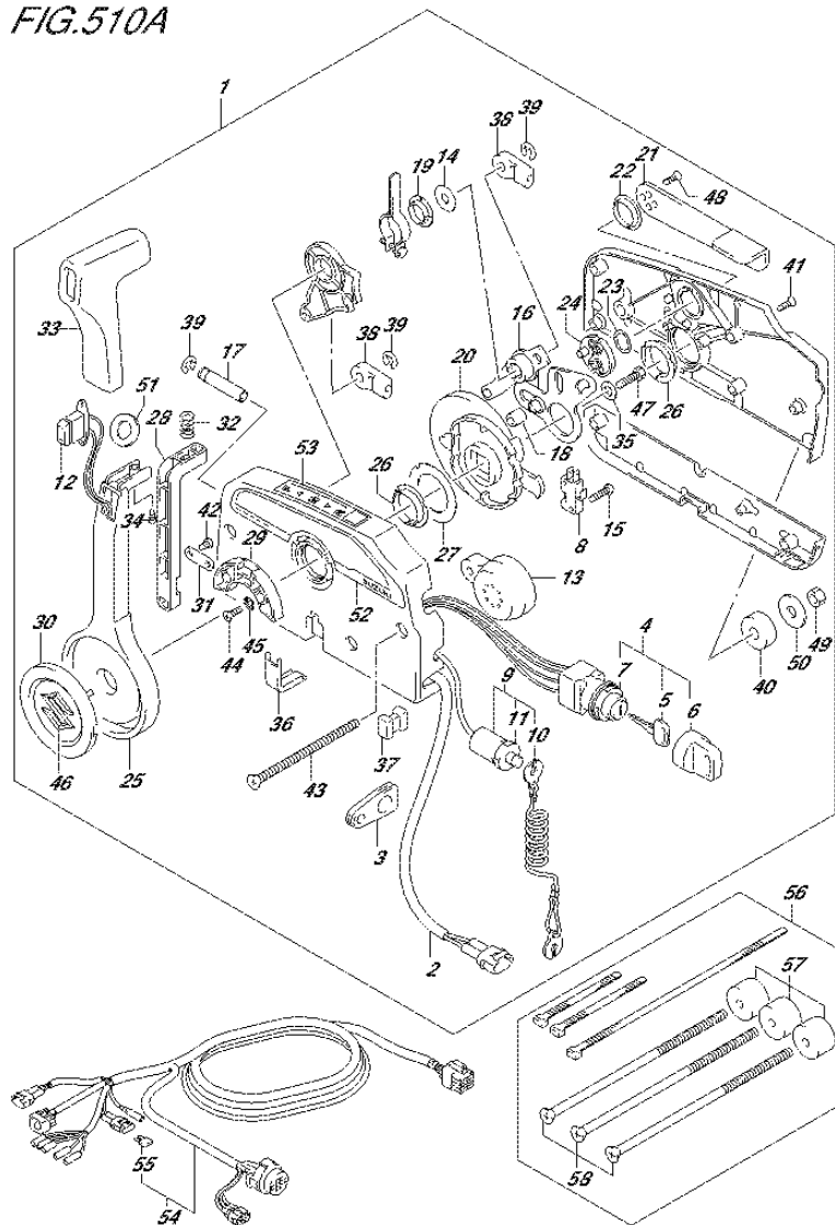
FIG.510A (3-D-6) OPT:REMOTE CONTROL (2) (DF100AT E11)
