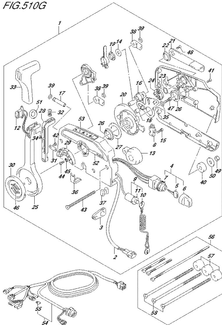
FIG.510G (3-E-10) OPT:REMOTE CONTROL (2) (DF140AT E40)
