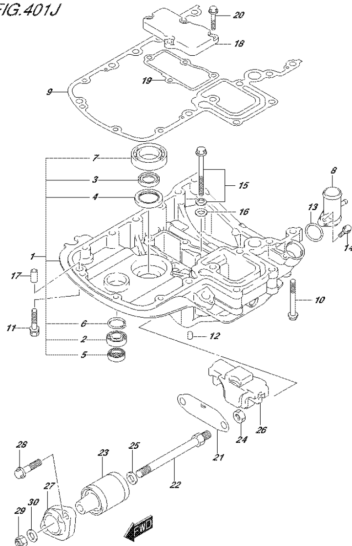
FIG.401J (2-F-14) ENGINE HOLDER (DF140AZ E40)
