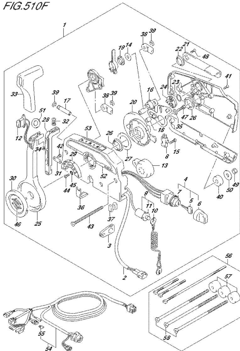
FIG.510F (3-E-9) OPT:REMOTE CONTROL (2) (DF140AT E11)
