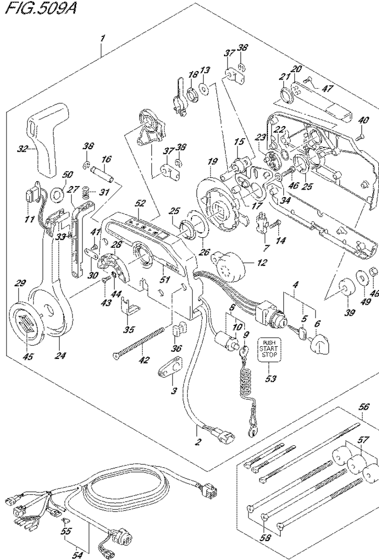
FIG.509A (3-C-6) OPT:REMOTE CONTROL (1) (DF100AT E11)
