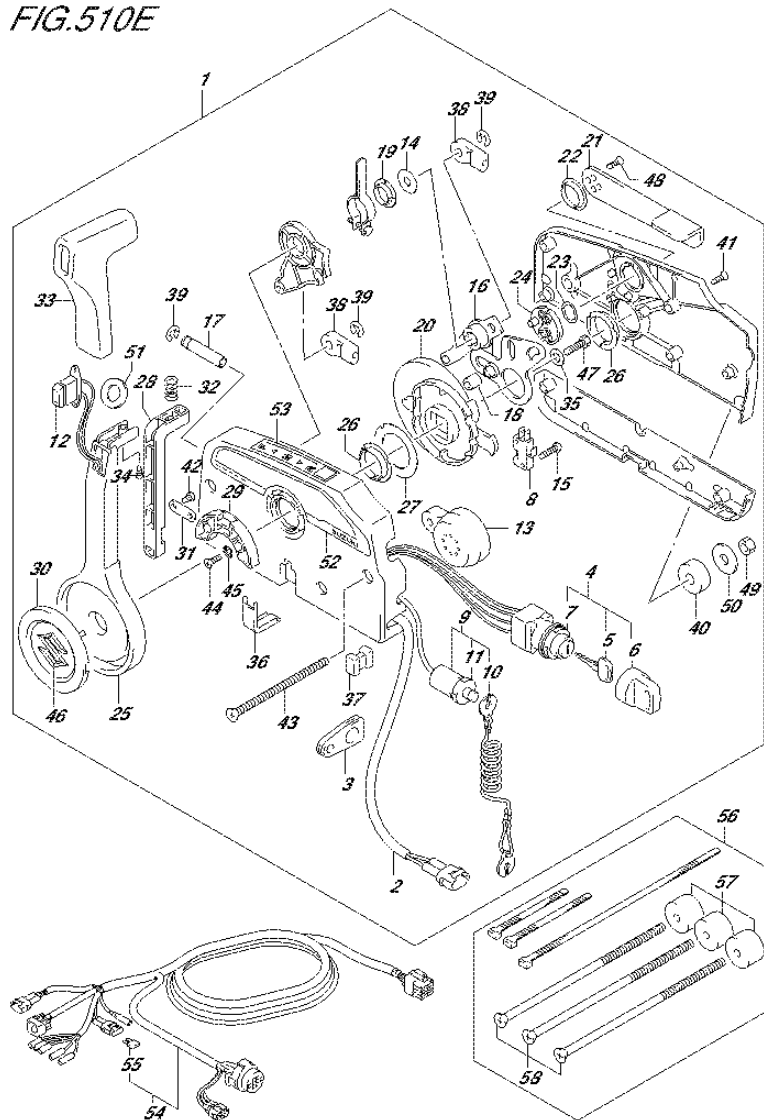
FIG.510E (3-E-6) OPT:REMOTE CONTROL (2) (DF115AZ E40)
