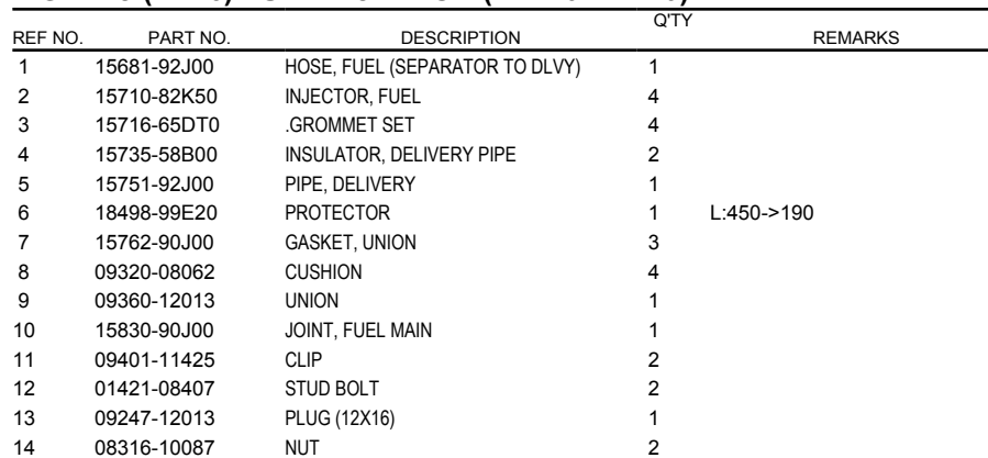
FIG.144J (1-E-6) FUEL INJECTOR (DF140AZ E40)
