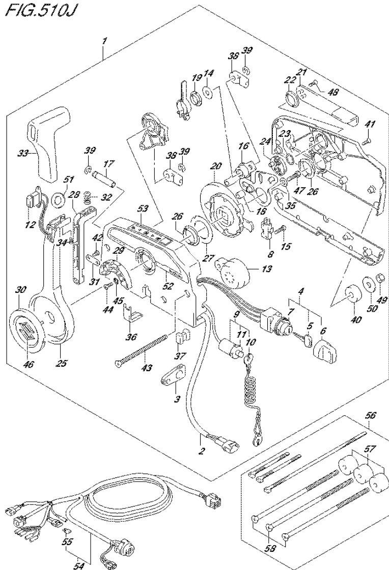
FIG.510J (3-F-2) OPT:REMOTE CONTROL (2) (DF140AZ E40)
