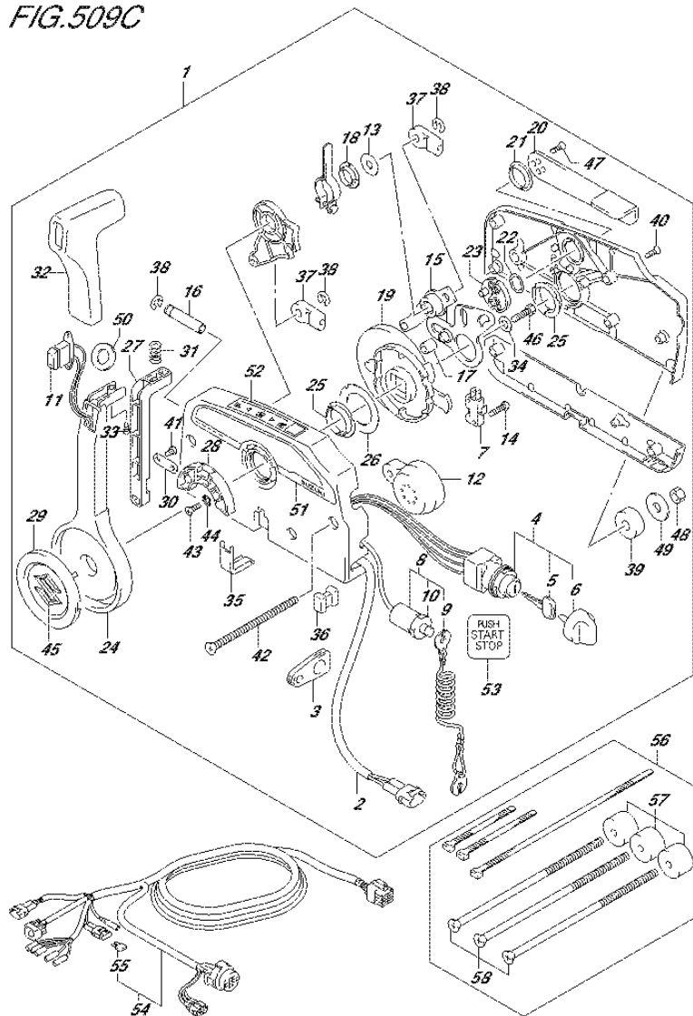
FIG.509C (3-C-12) OPT:REMOTE CONTROL (1) (DF115AZ E11)
