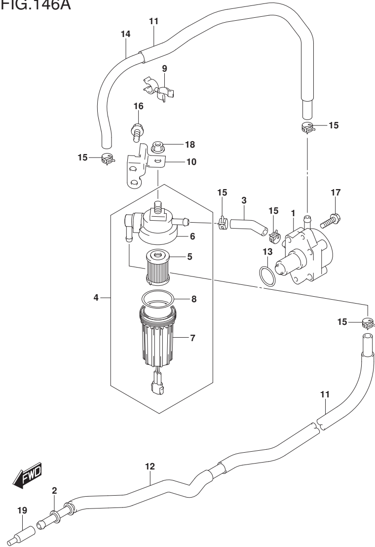
DF140A_E11_019_146A FUEL PUMP
