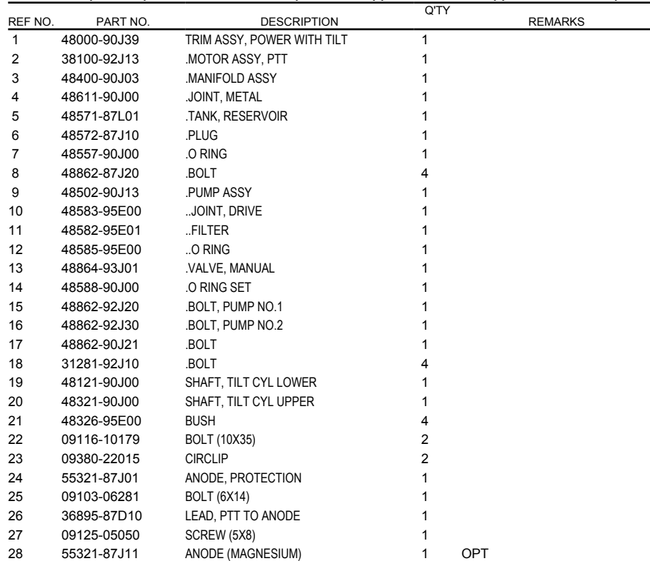
FIG.337A (1-F-14) TRIM CYLINDER (DF100AT)(DF115AT E11)(DF115AZ E11)
