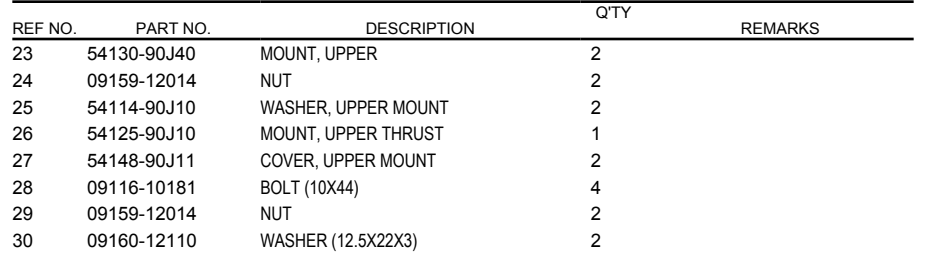
FIG.401B (1-G-10) ENGINE HOLDER (DF115AT)(DF115AZ)(DF140AT)(DF140AZ)
