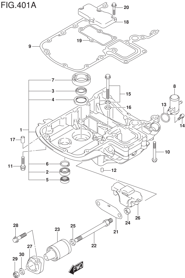
DF140A_E11_019_401A ENGINE HOLDER
