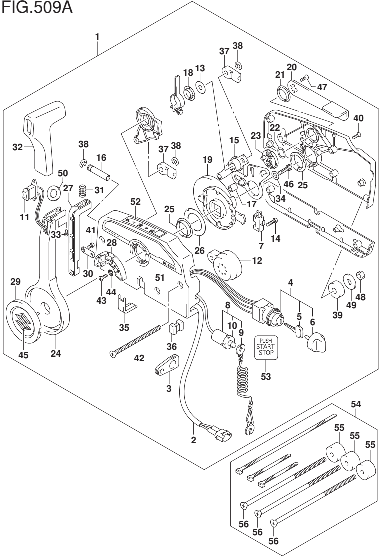
FIG.509A (1-J-15) OPT:REMOTE CONTROL (1) (E11)
