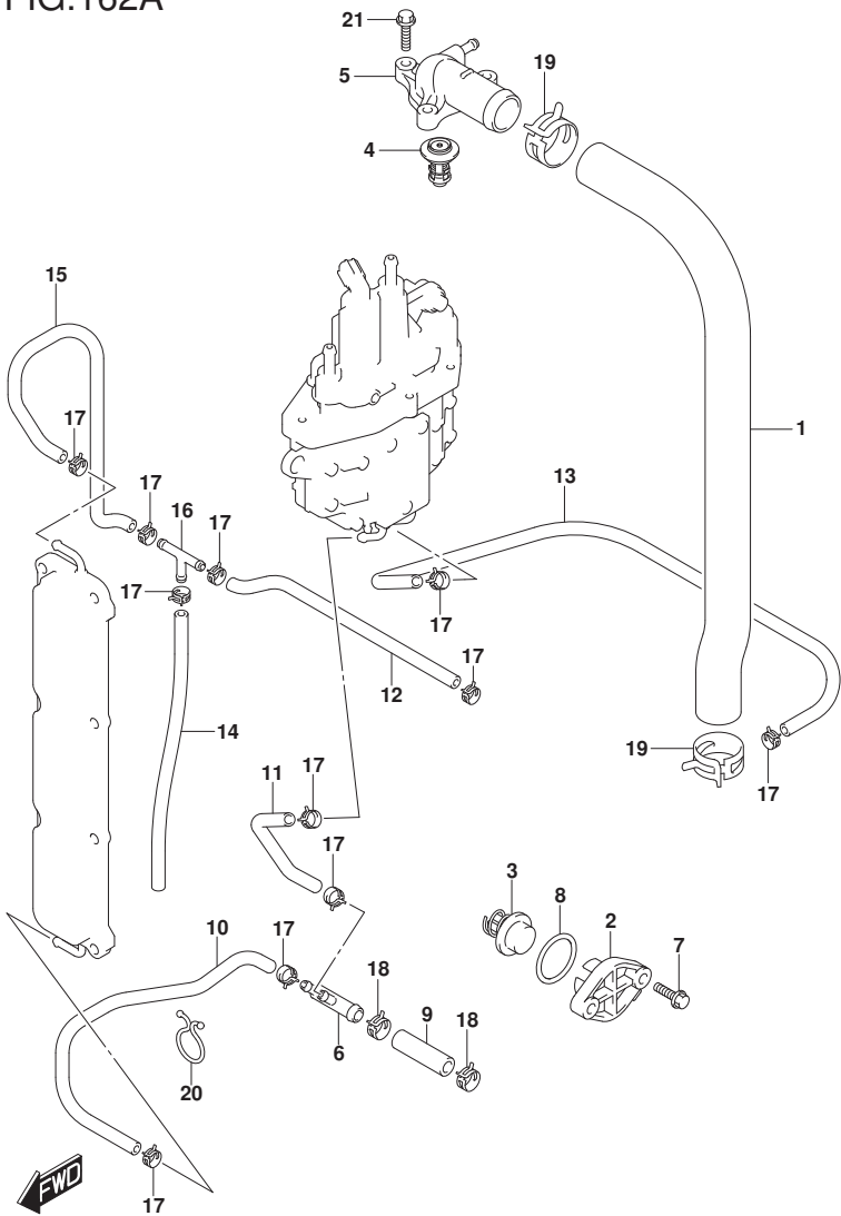
DF140A_E11_020_162A THERMOSTAT
