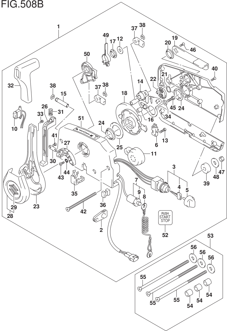
FIG.508B (1-J-12) OPT:REMOTE CONTROL (W/KEY LESS START) (E11)
