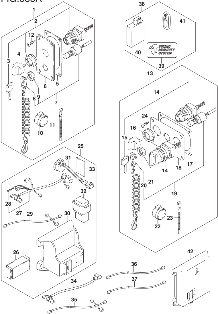
DF140A_E11_020_535A OPT:KEY LESS START
