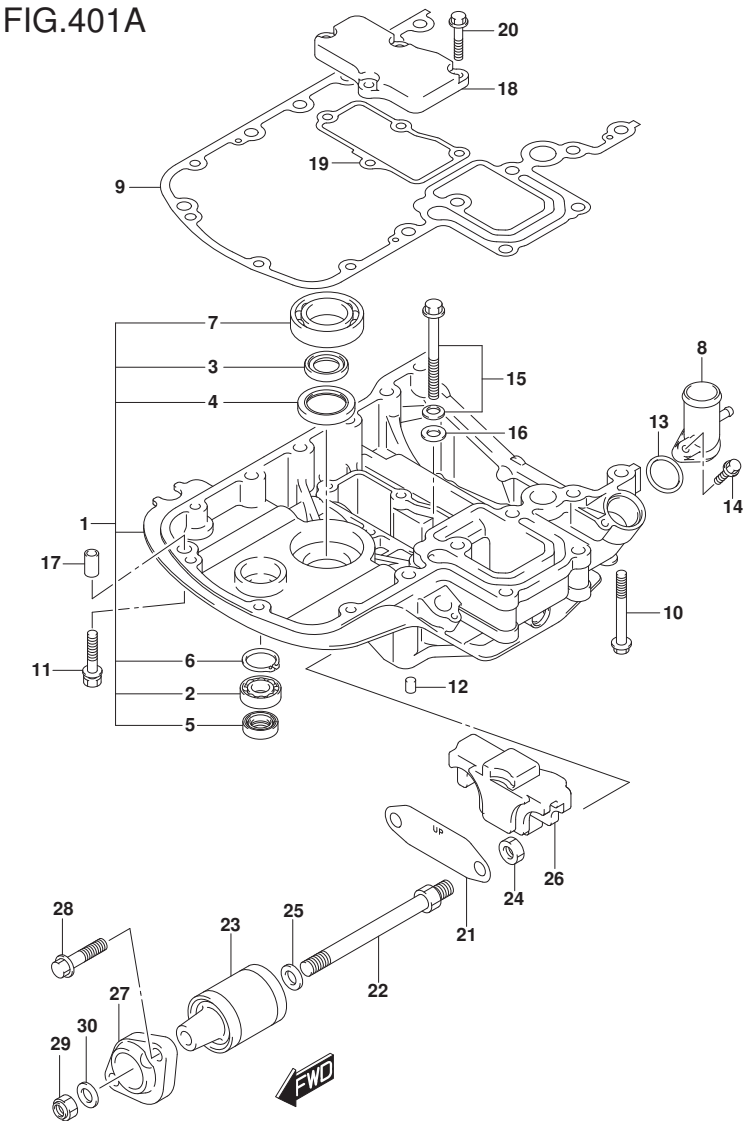
DF140A_E11_020_401A ENGINE HOLDER
