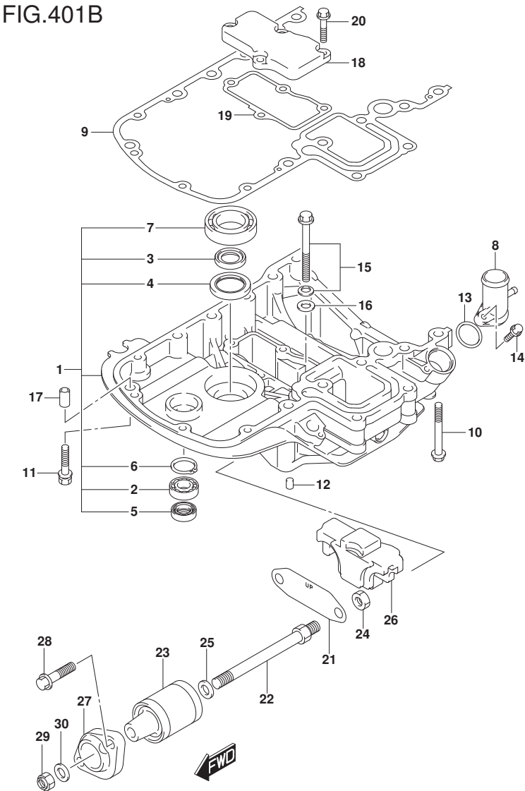
DF140A_E11_020_401B ENGINE HOLDER
