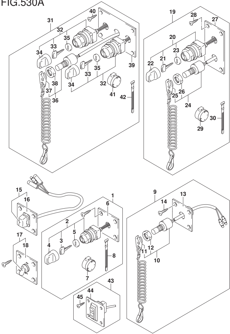
DF140A_E11_020_530A OPT:SWITCH
