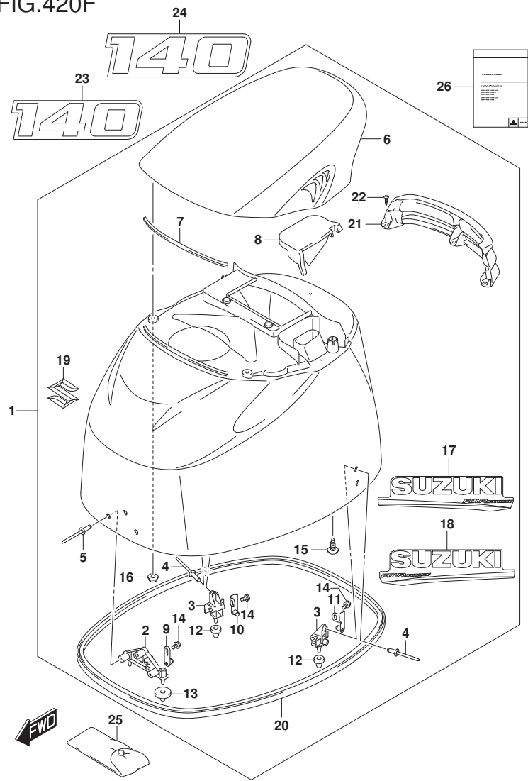
DF140A_E11_020_420F ENGINE COVER
