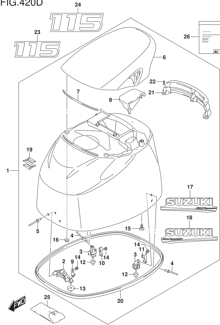
DF140A_E11_020_420D ENGINE COVER
