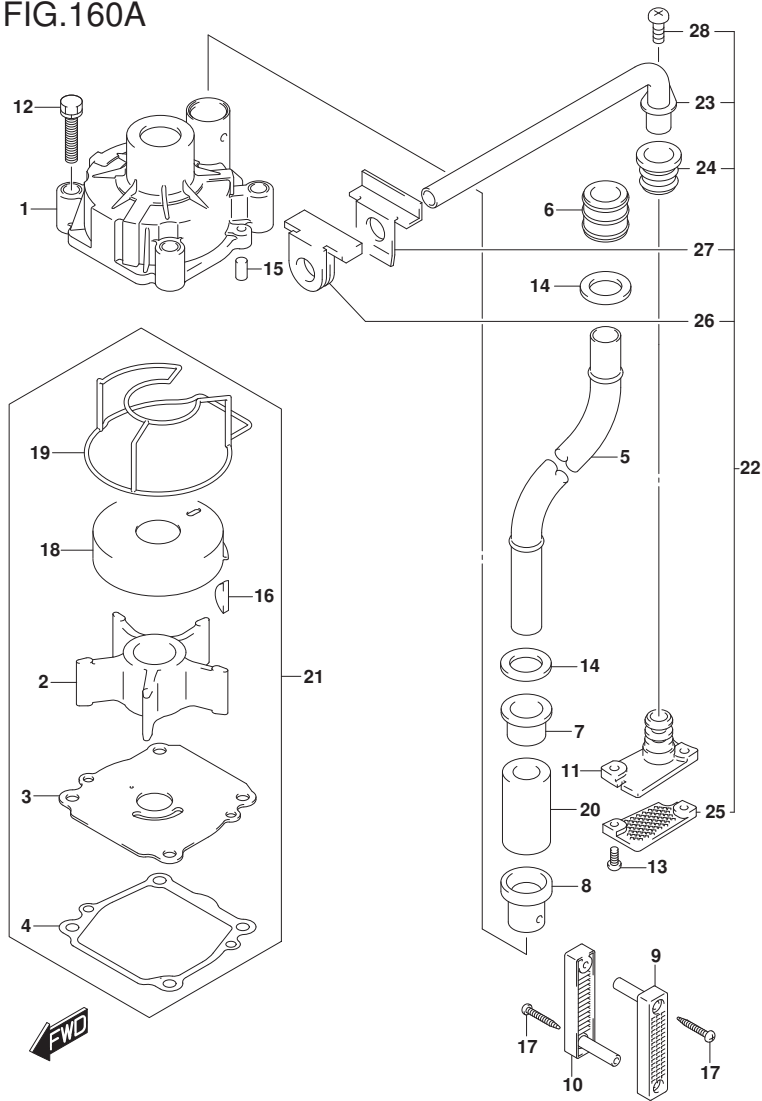
FIG.160A (1-C-6) WATER PUMP (E03)(E11)
