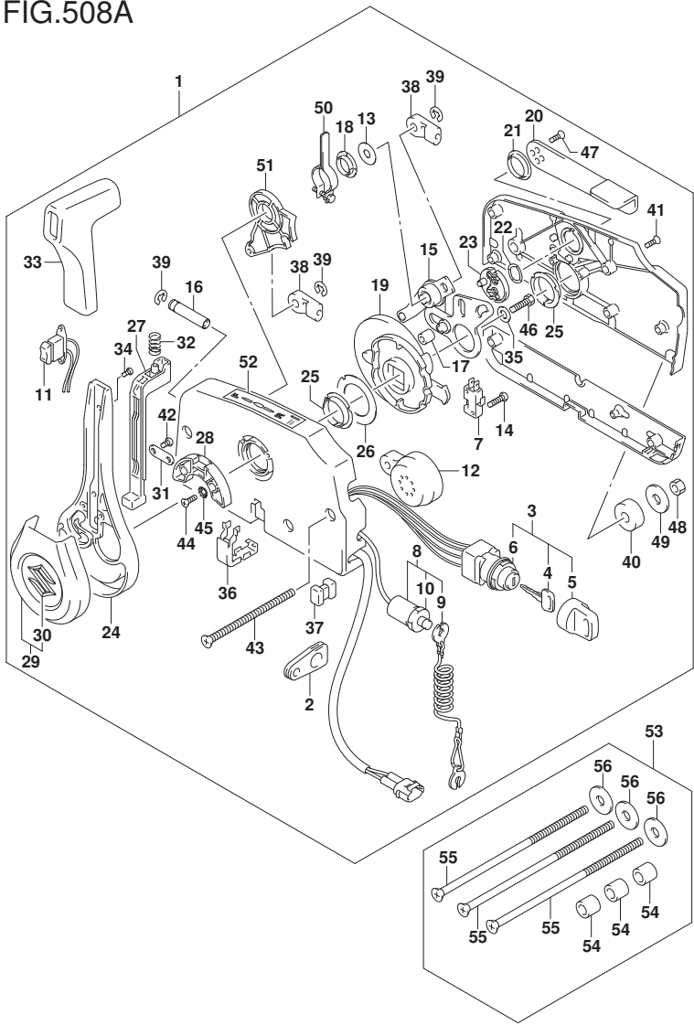
FIG.508A (1-J-10) OPT:REMOTE CONTROL (N/KEY LESS START) (E11)(E40)
