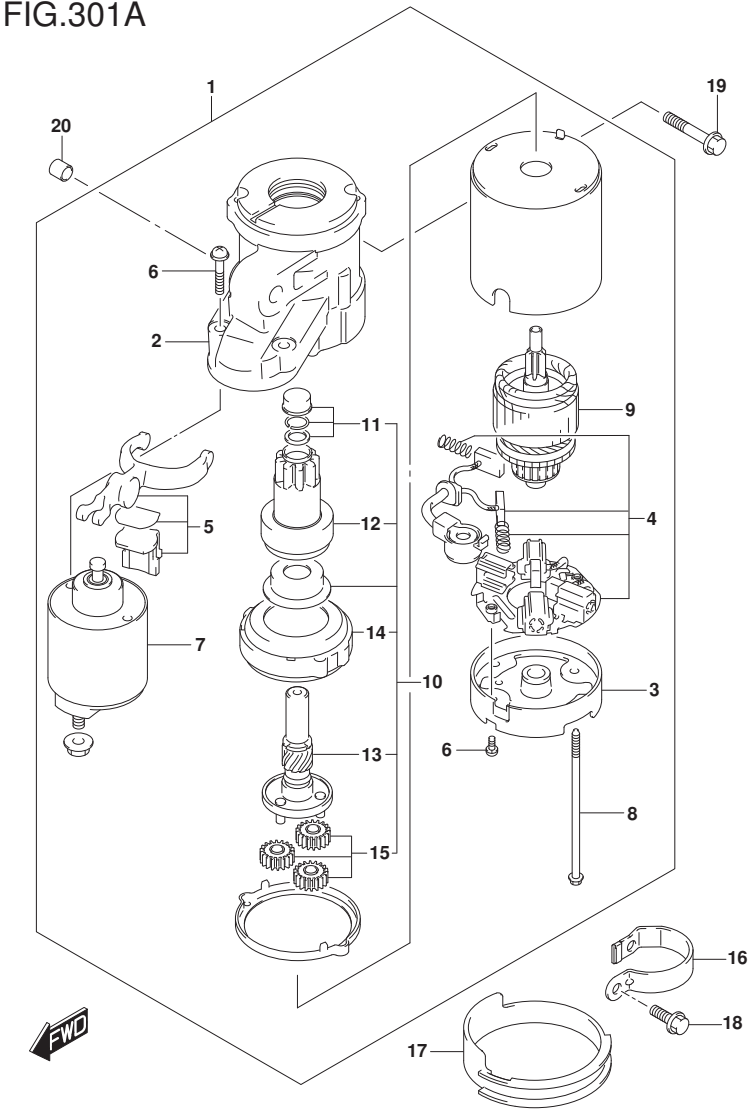
DF140A_E11_020_301A STARTING MOTOR
