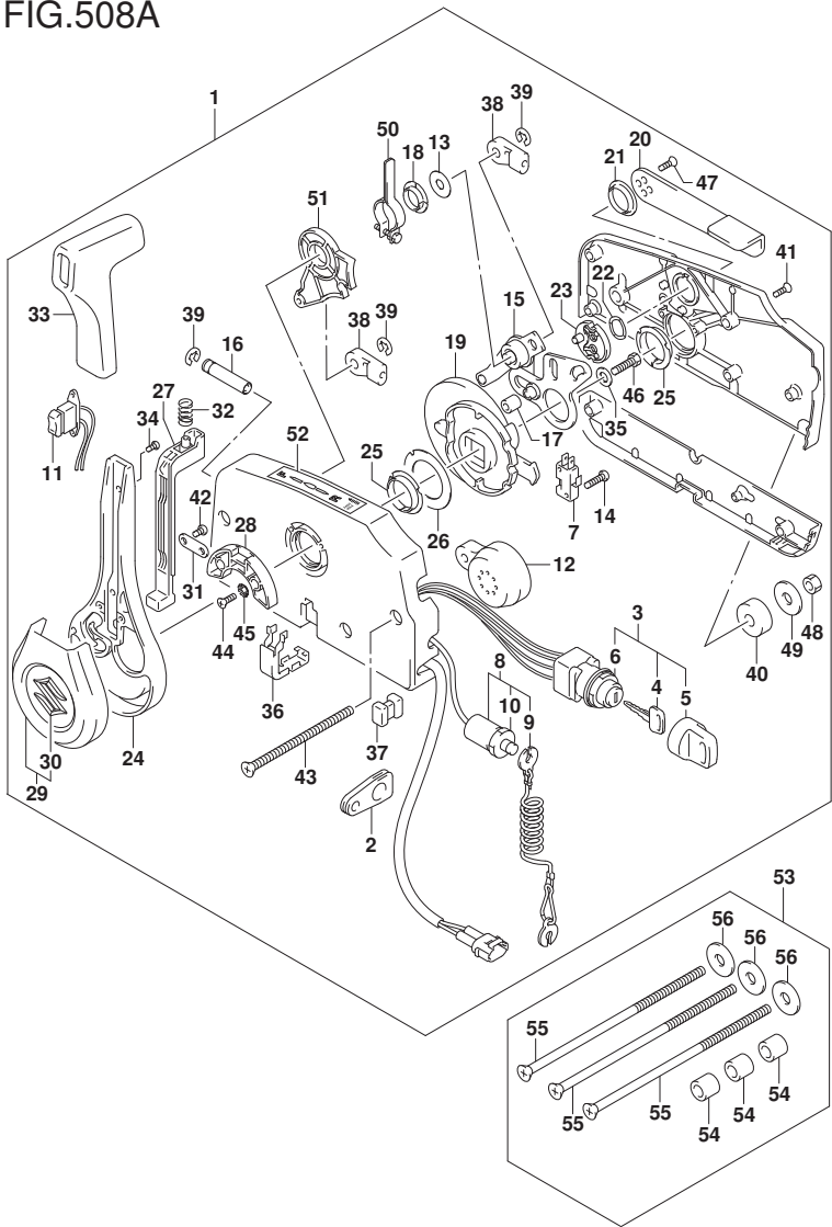
FIG.508A (1-J-9) OPT:REMOTE CONTROL (N/KEY LESS START) (E11)(E40)
