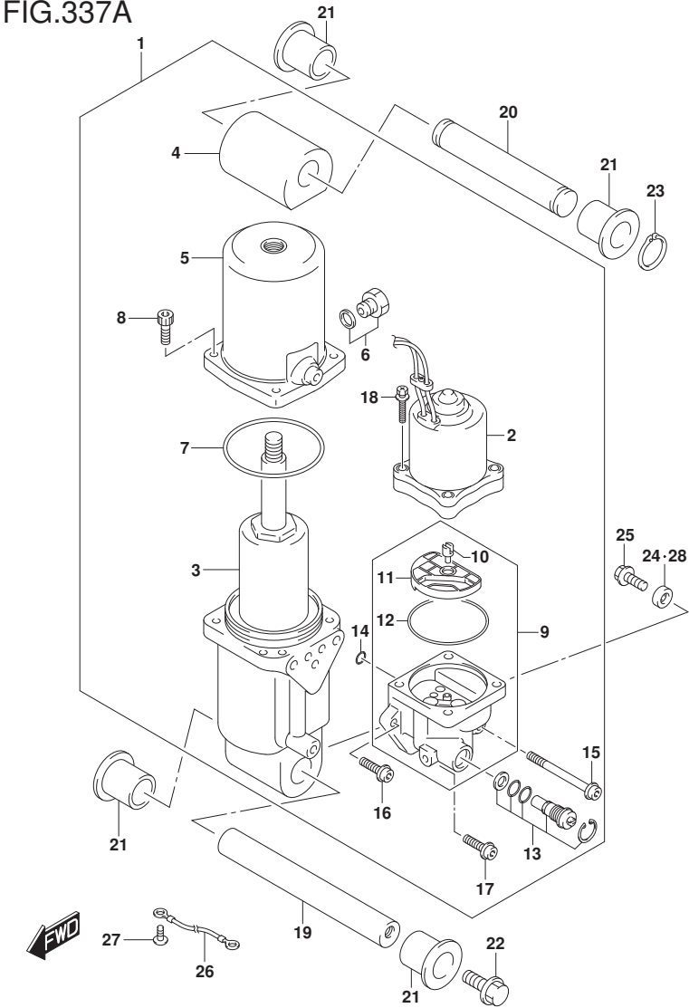
FIG.337A (1-F-12) TRIM CYLINDER (DF100AT)(DF115AT E11)(DF115AZ E11)
