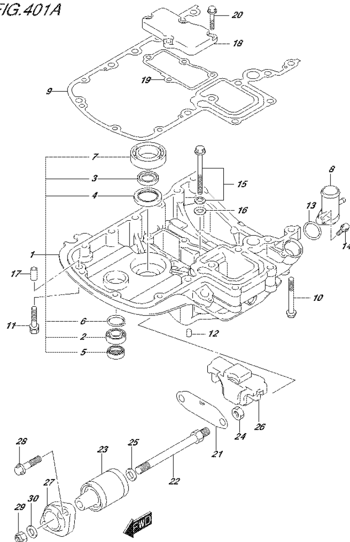
FIG.401A (2-F-3) ENGINE HOLDER (DF100AT E01)
