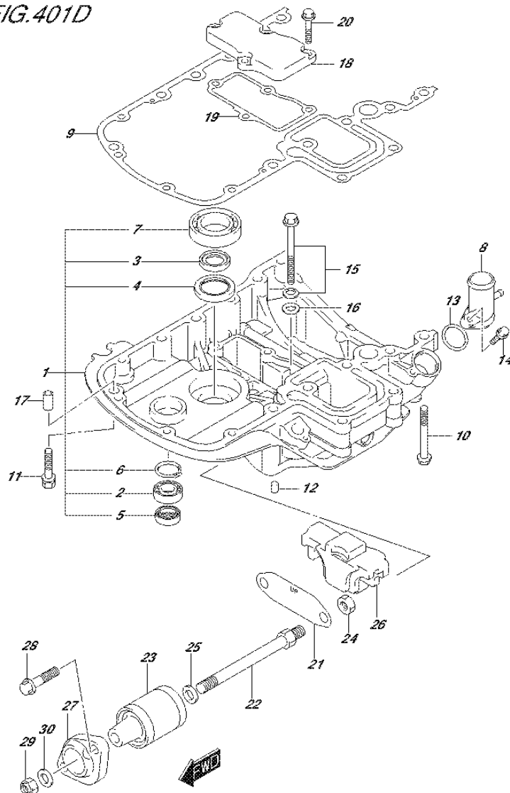
FIG.401D (2-F-6) ENGINE HOLDER (DF115AZ E01)
