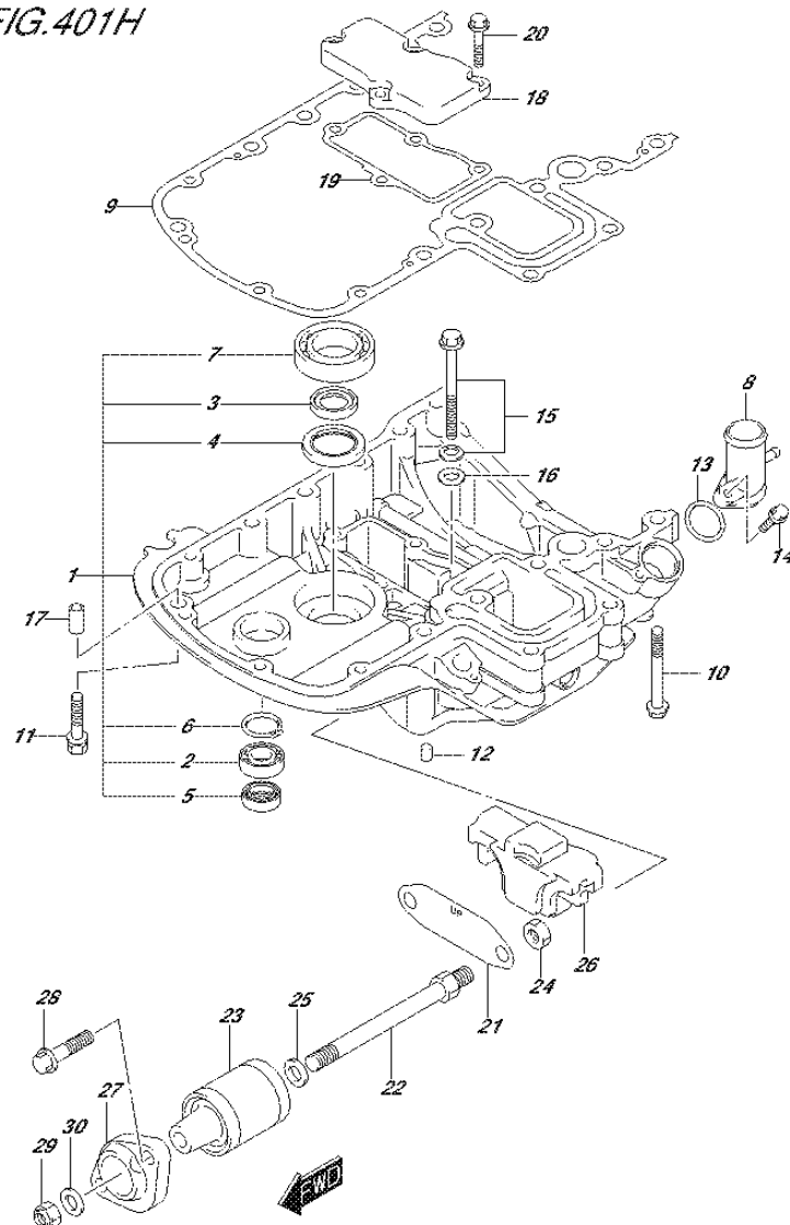
FIG.401H (2-F-10) ENGINE HOLDER (DF140AZ E01)
