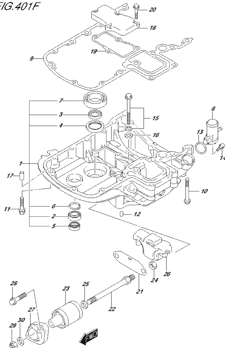
FIG.401F (2-F-8) ENGINE HOLDER (DF140AT E01)
