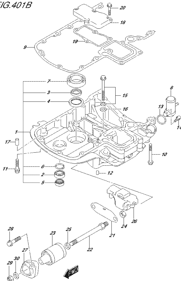
FIG.401B (2-F-4) ENGINE HOLDER (DF115AT E01)
