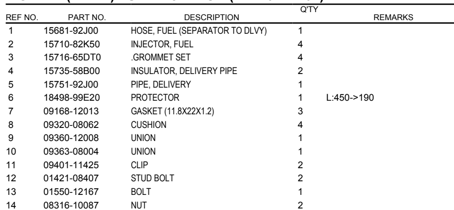
FIG.144F (1-F-11) FUEL INJECTOR (DF140AT E01)
