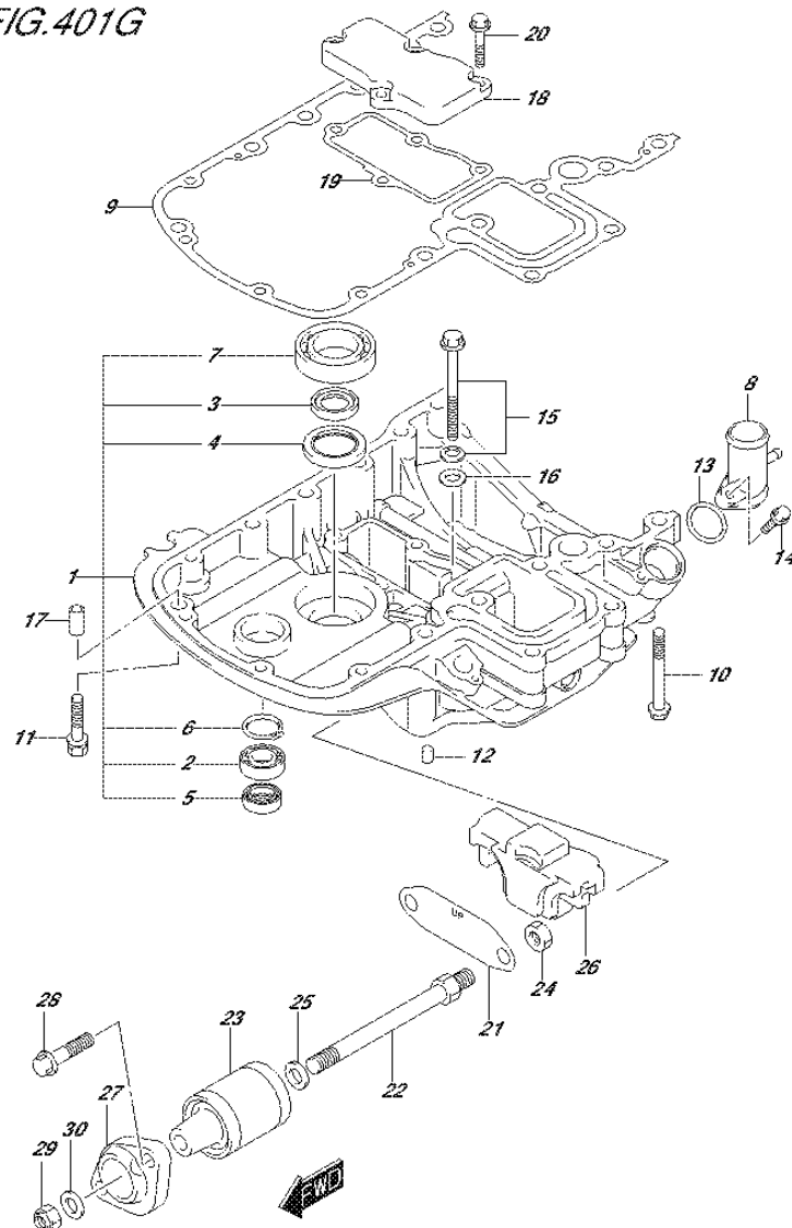
FIG.401G (2-F-9) ENGINE HOLDER (DF140AT E40)
