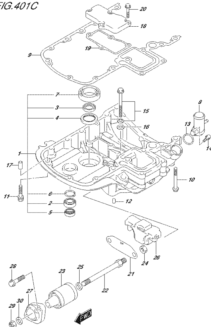
FIG.401C (2-F-5) ENGINE HOLDER (DF115AT E40)
