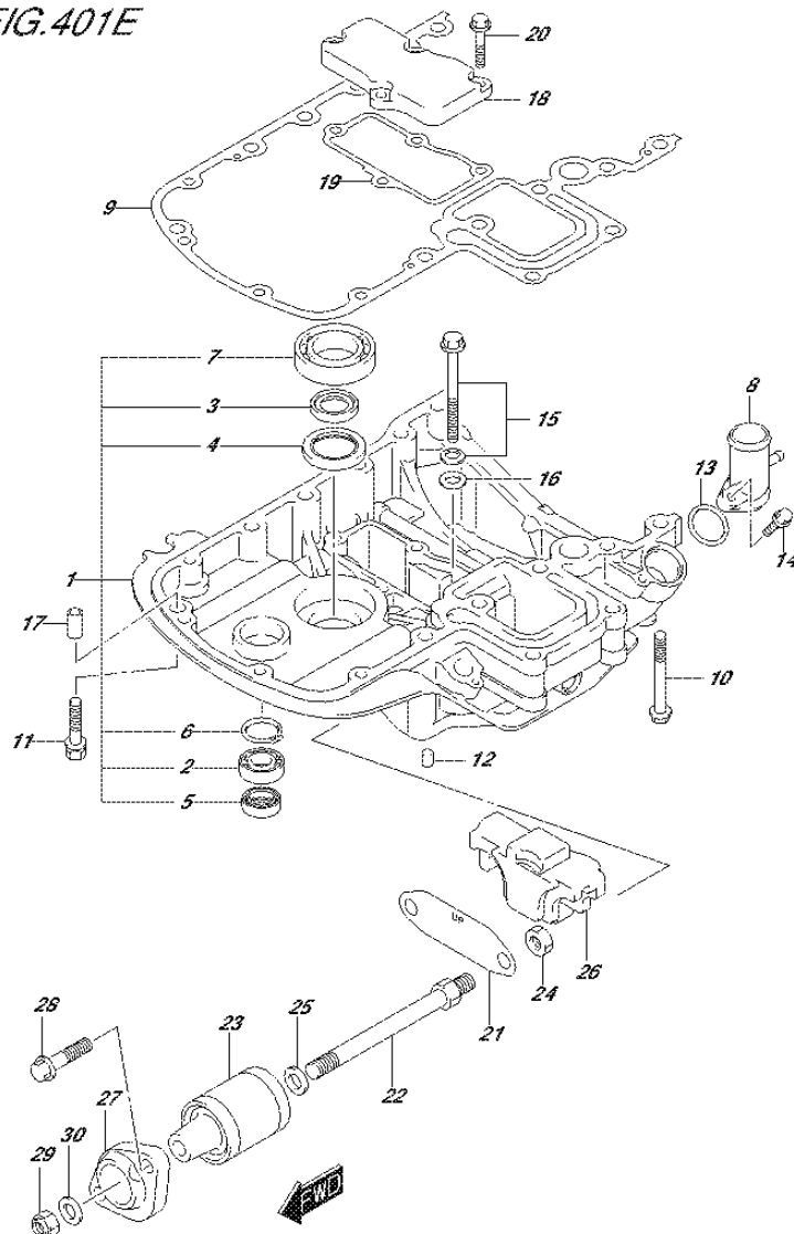
FIG.401E (2-F-7) ENGINE HOLDER (DF115AZ E40)
