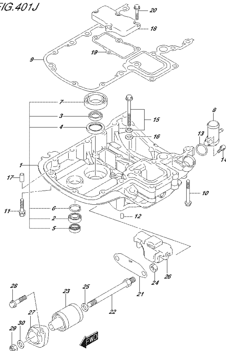
FIG.401J (2-F-11) ENGINE HOLDER (DF140AZ E40)
