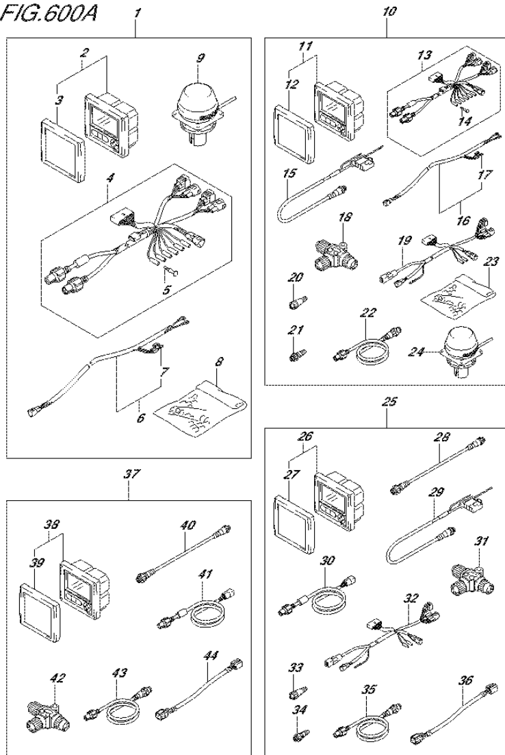
FIG.600A (3-D-9) OPT:MULTI FUNCTION GAUGE
