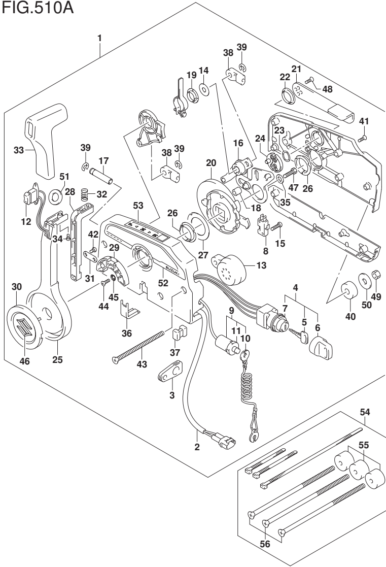
FIG.510A (1-K-5) OPT:REMOTE CONTROL (2) (E11)
