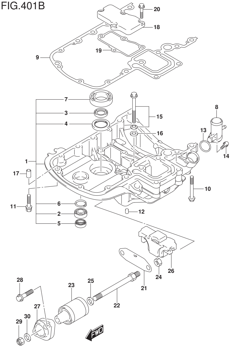
DF140A_E11_018_401B ENGINE HOLDER
