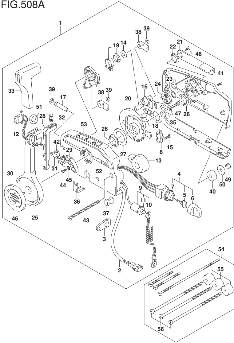
FIG.508A (1-J-13) OPT:REMOTE CONTROL (E40)
