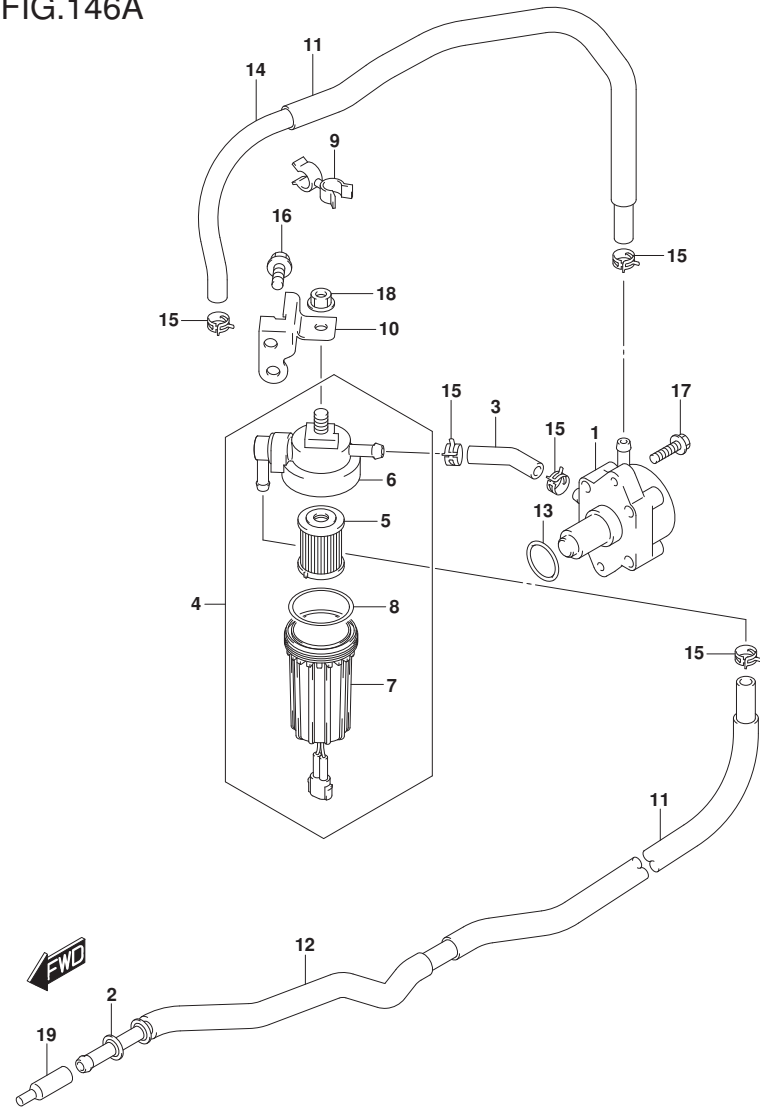
DF140A_E11_018_146A FUEL PUMP
