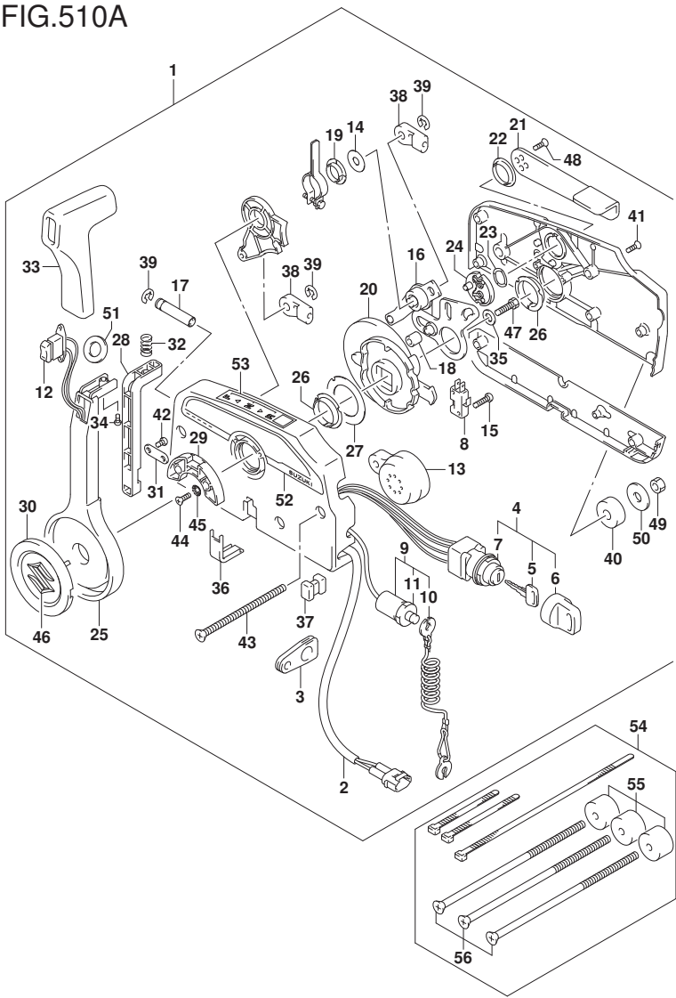
FIG.510A (1-K-6) OPT:REMOTE CONTROL (2) (E11)
