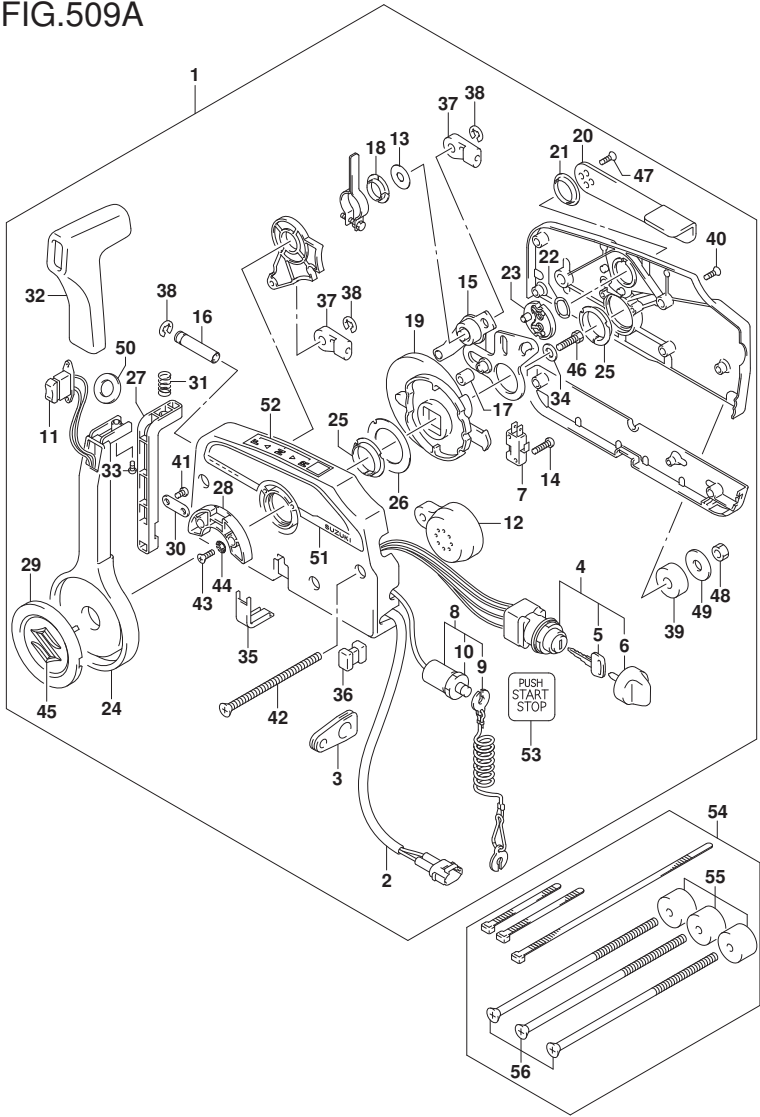
FIG.509A (1-K-3) OPT:REMOTE CONTROL (1) (E11)
