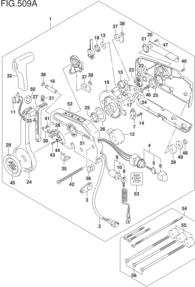
FIG.509A (1-K-2) OPT:REMOTE CONTROL (1) (E11)
