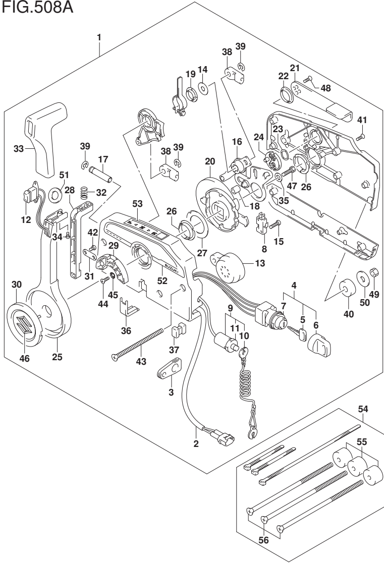
FIG.508A (1-J-12) OPT:REMOTE CONTROL (E40)
