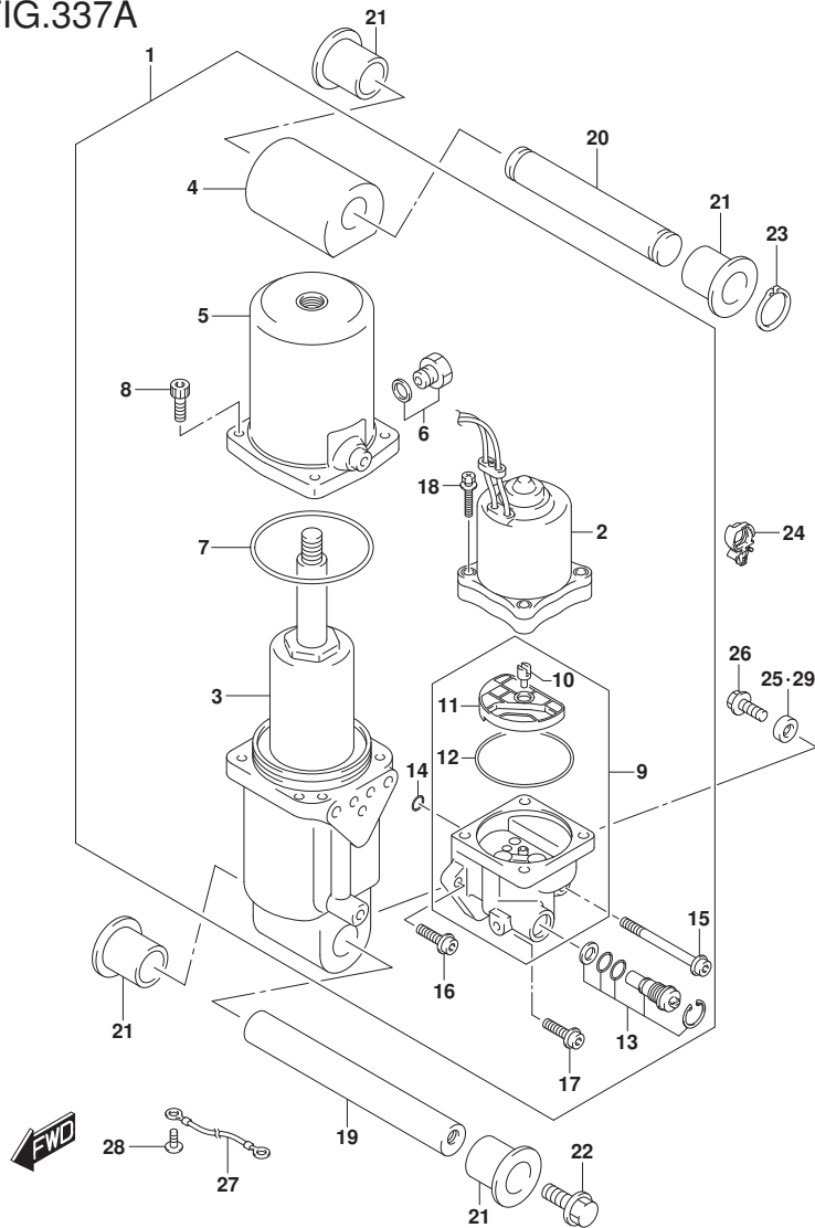
FIG.337A (1-F-15) TRIM CYLINDER (DF100AT)(DF115AT E11)(DF115AZ E11)
