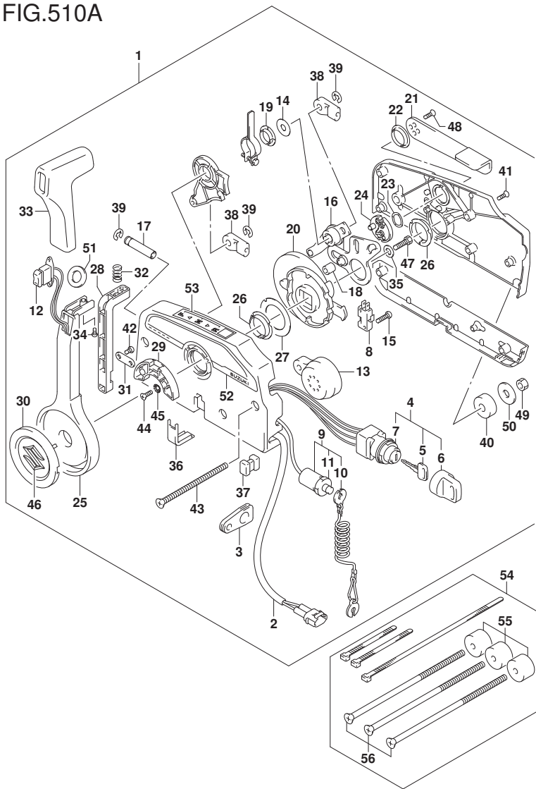
FIG.510A (1-K-4) OPT:REMOTE CONTROL (2) (E11)
