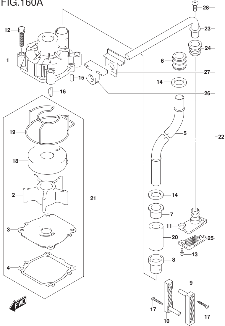
DF140A_E11_018_160A WATER PUMP
