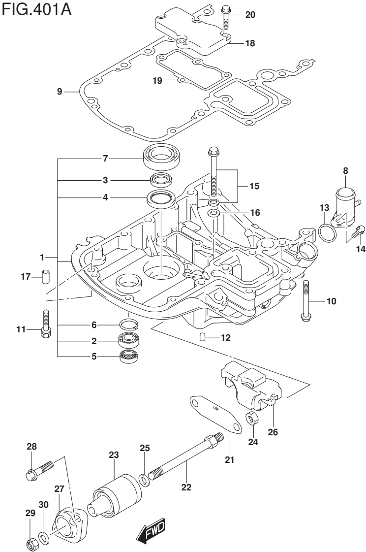
DF140A_E11_018_401A ENGINE HOLDER
