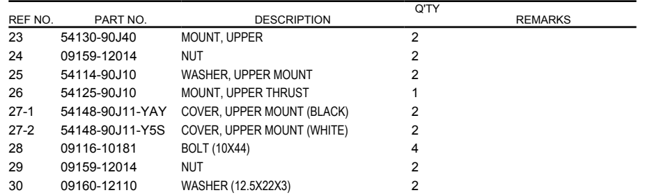
FIG.401B (1-G-11) ENGINE HOLDER (DF115AT)(DF115AZ)(DF140AT)(DF140AZ)
