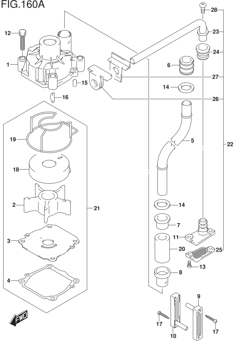
FIG.160A (1-C-6) WATER PUMP (E11)(E03)
