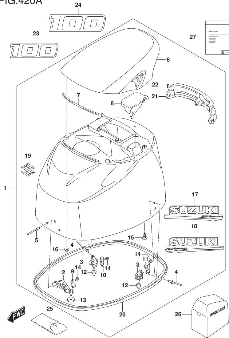
DF140A_E11_018_420A ENGINE COVER
