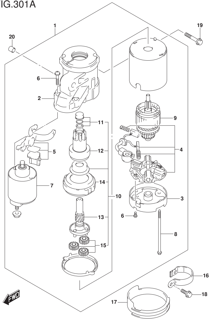
FIG.301A (1-D-14) STARTING MOTOR
