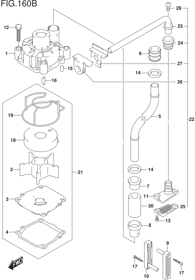
FIG.160B (1-C-8) WATER PUMP (E40)
