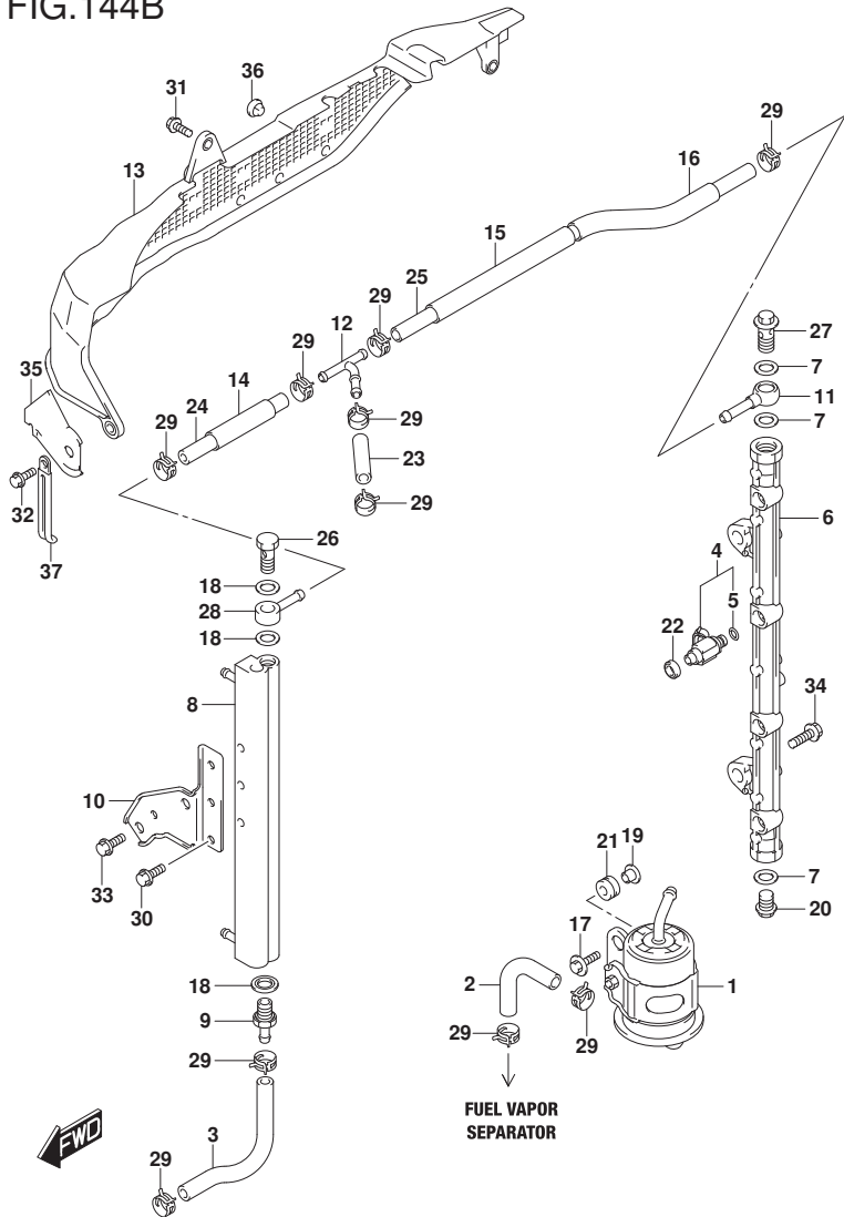
DF175_E01_017_144B FUEL INJECTOR
