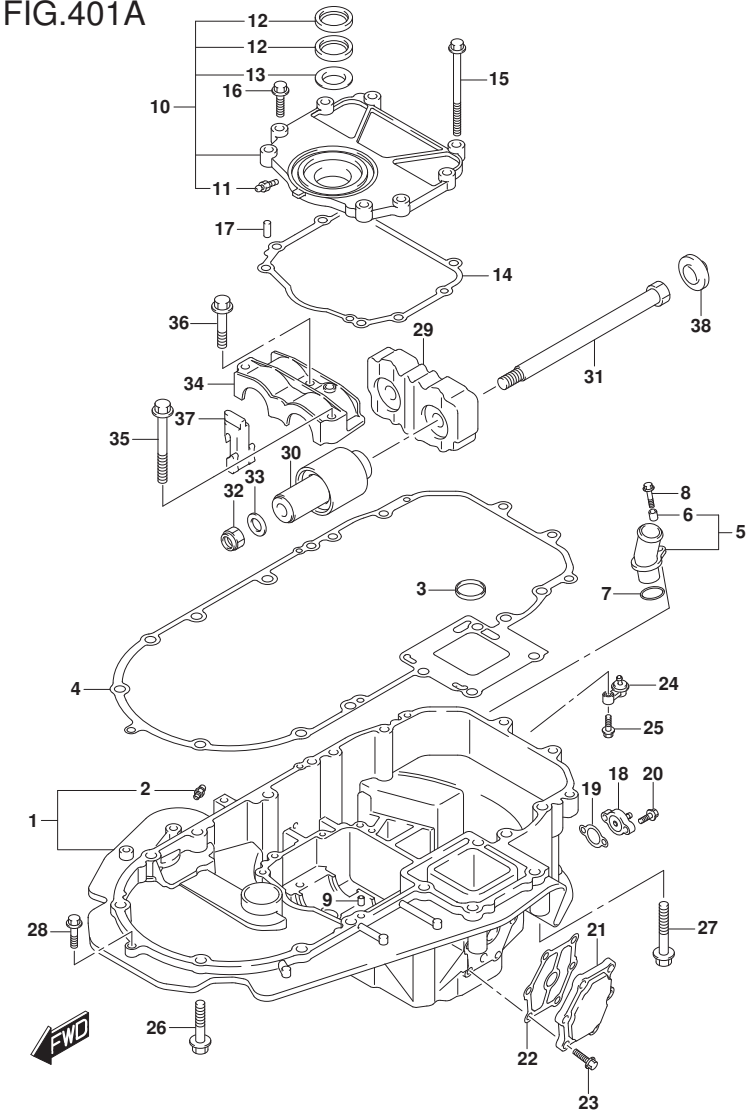
FIG.401A (1-K-13) ENGINE HOLDER
