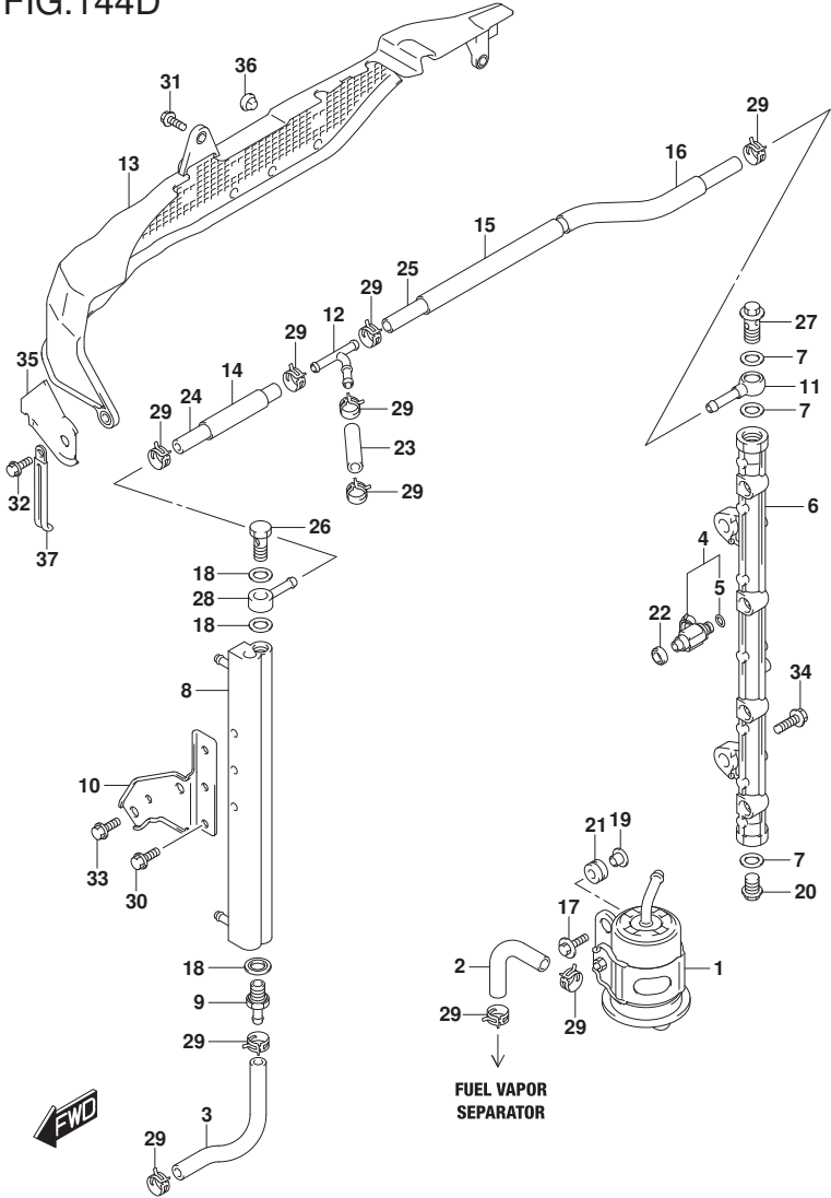
DF175_E01_017_144D FUEL INJECTOR
