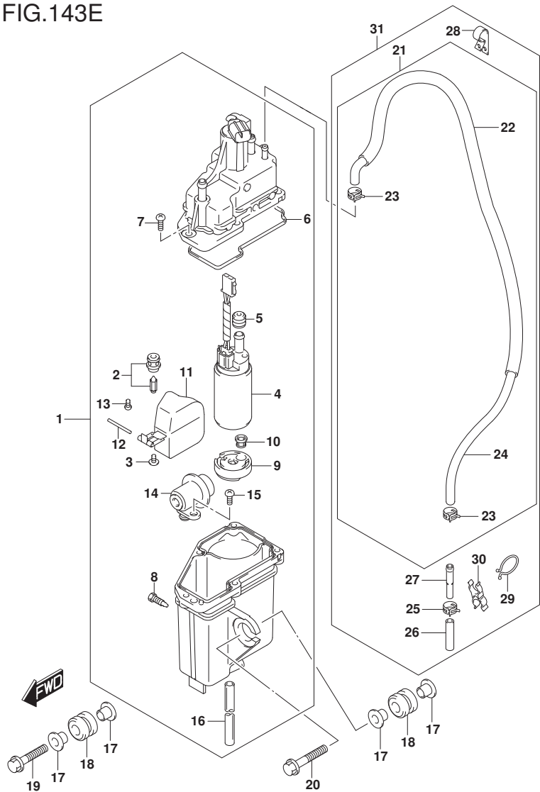
FIG.143E (1-D-10) FUEL VAPOR SEPARATOR (DF175T E01)
