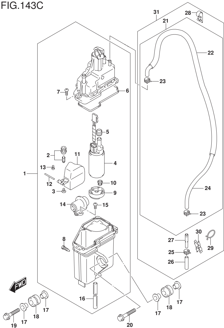
DF175_E01_017_143C FUEL VAPOR SEPARATOR
