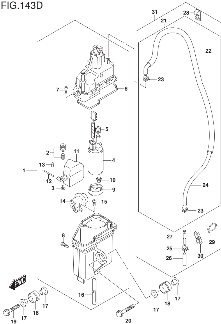
DF175_E01_017_143D FUEL VAPOR SEPARATOR
