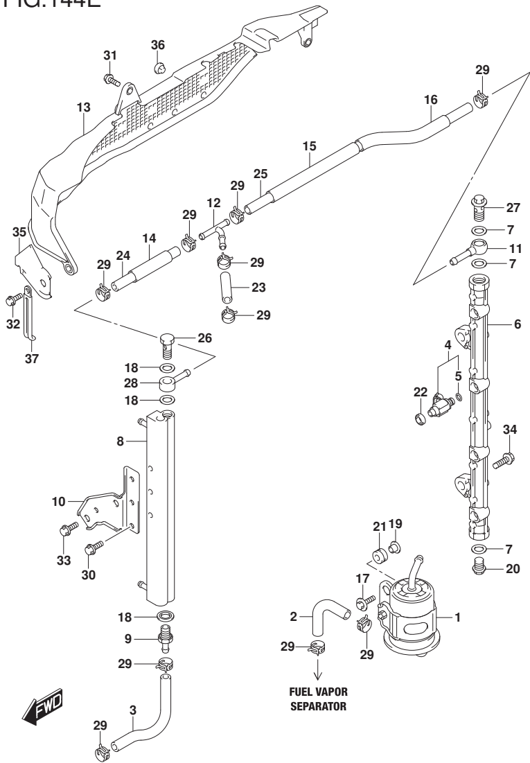
DF175_E01_017_144E FUEL INJECTOR
