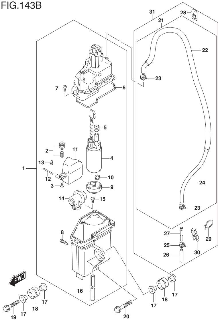
DF175_E01_017_143B FUEL VAPOR SEPARATOR
