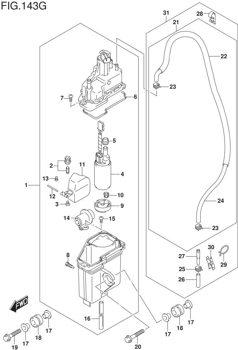
DF175_E01_017_143G FUEL VAPOR SEPARATOR
