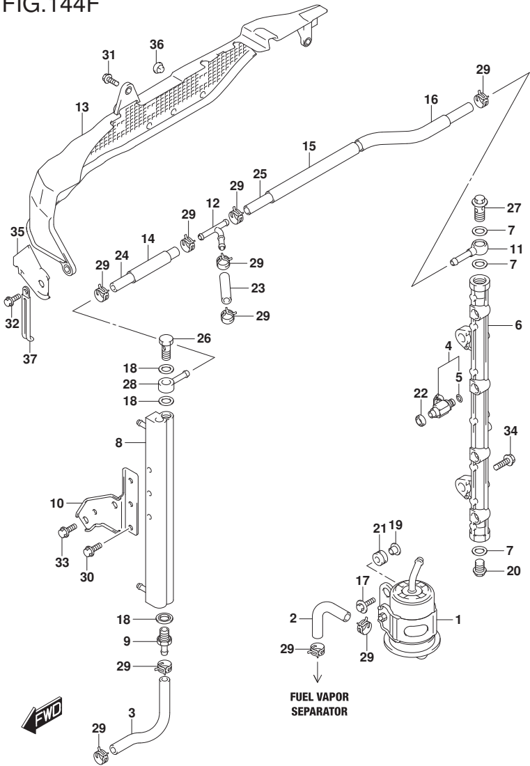
DF175_E01_017_144F FUEL INJECTOR
