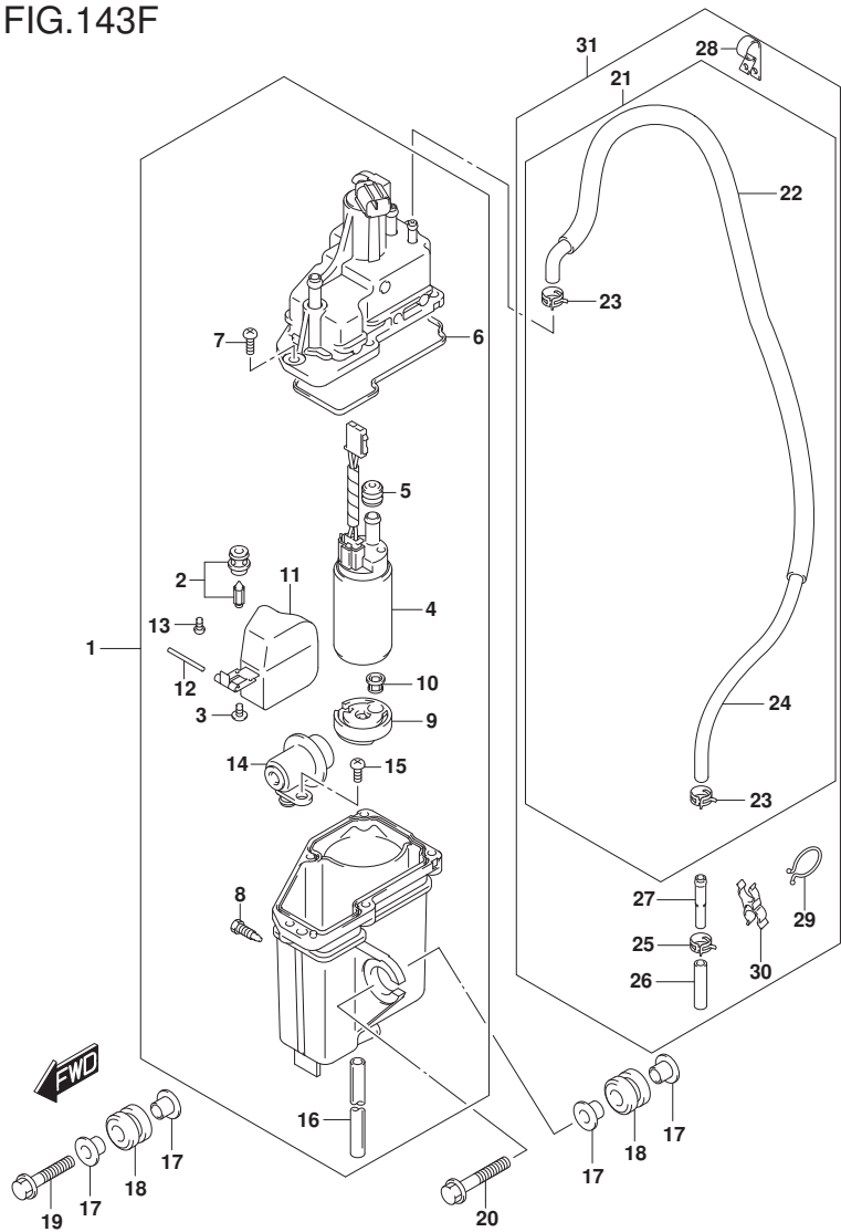
DF175_E01_017_143F FUEL VAPOR SEPARATOR
