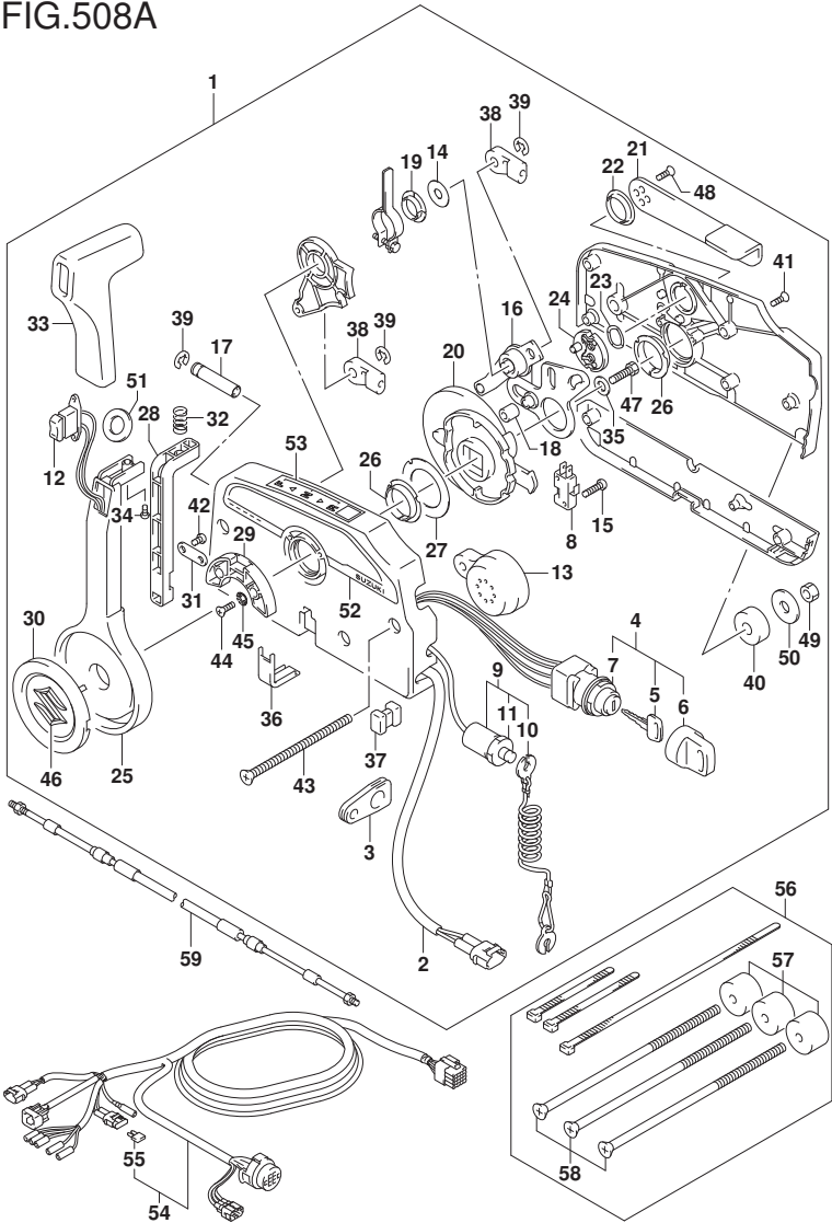
FIG.508A (2-C-13) OPT:REMOTE CONTROL
