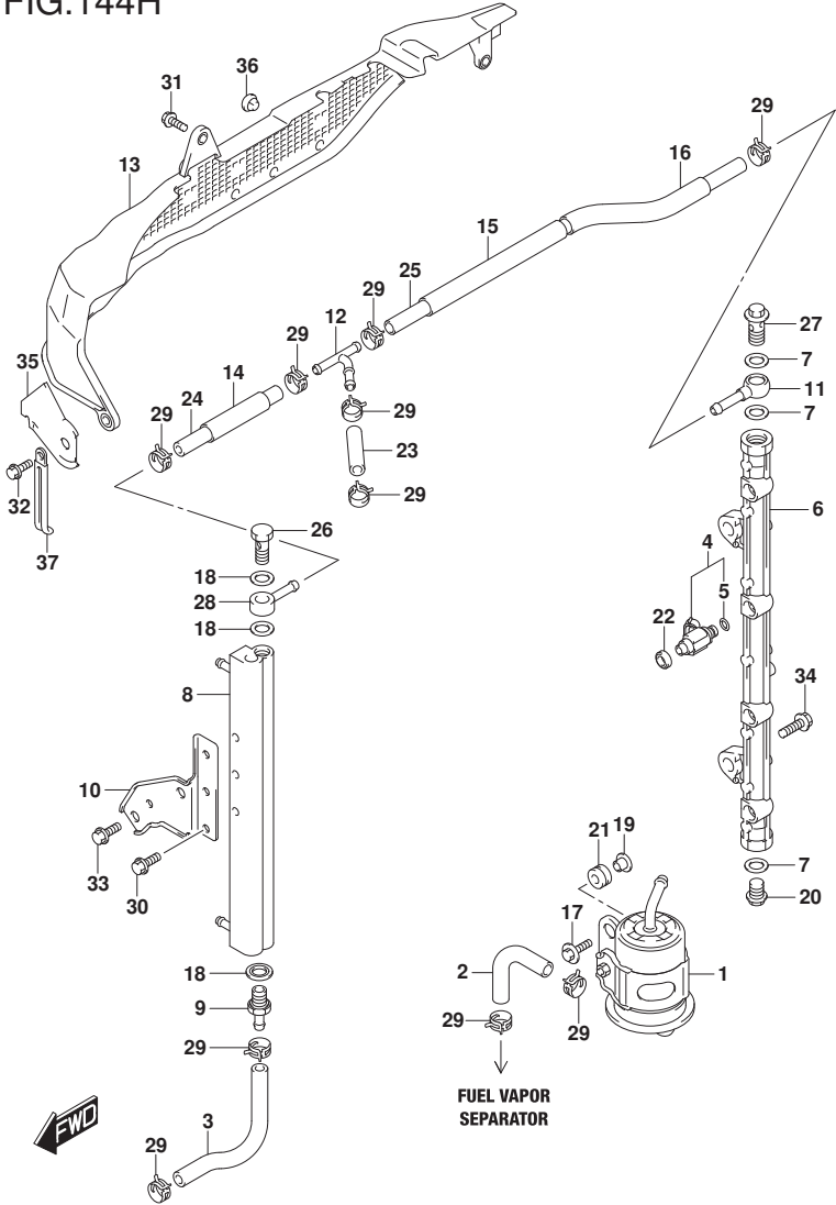
DF175_E01_017_144H FUEL INJECTOR
