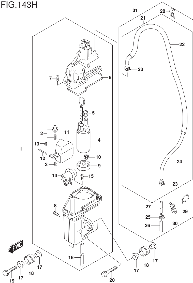
DF175_E01_017_143H FUEL VAPOR SEPARATOR
