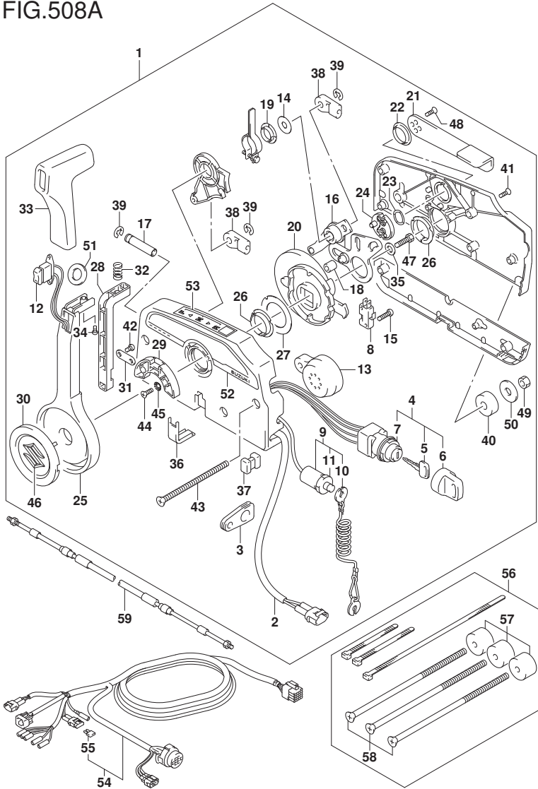
FIG.508A (2-C-12) OPT:REMOTE CONTROL
