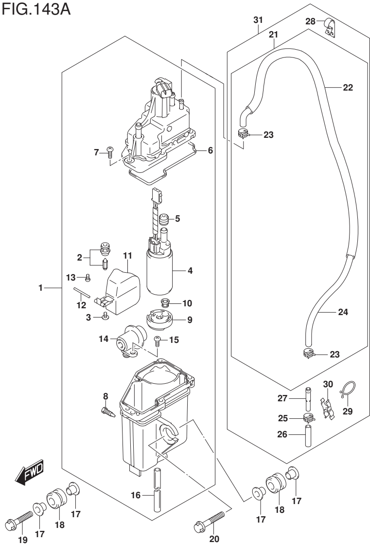
DF175_E01_017_143A FUEL VAPOR SEPARATOR
