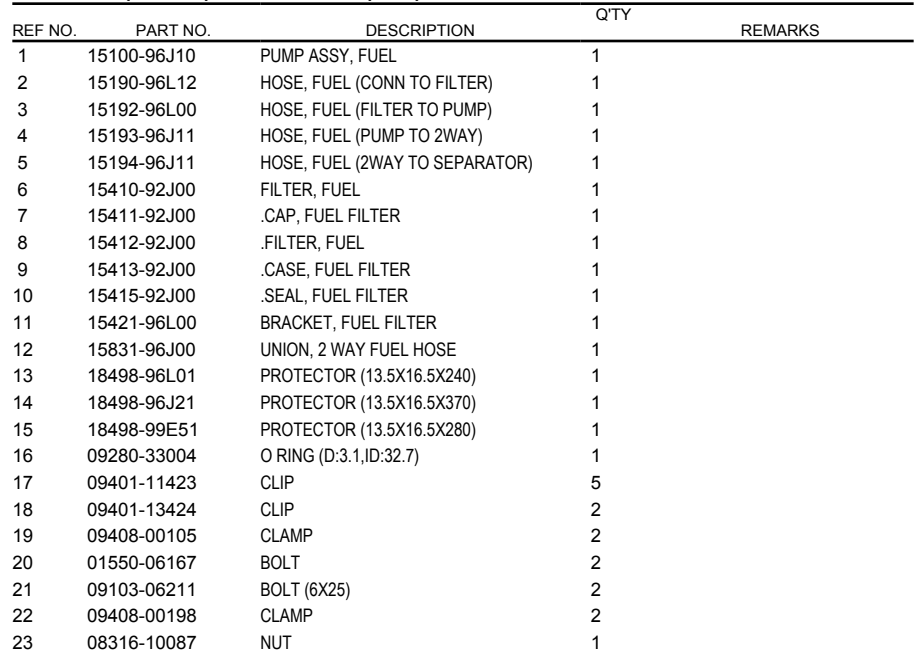
FIG.146B (1-C-15) FUEL PUMP (E40)
