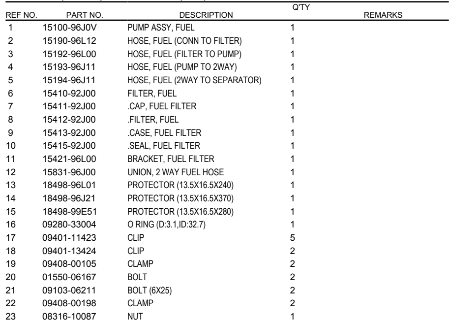
FIG.146A (1-C-14) FUEL PUMP (E01)
