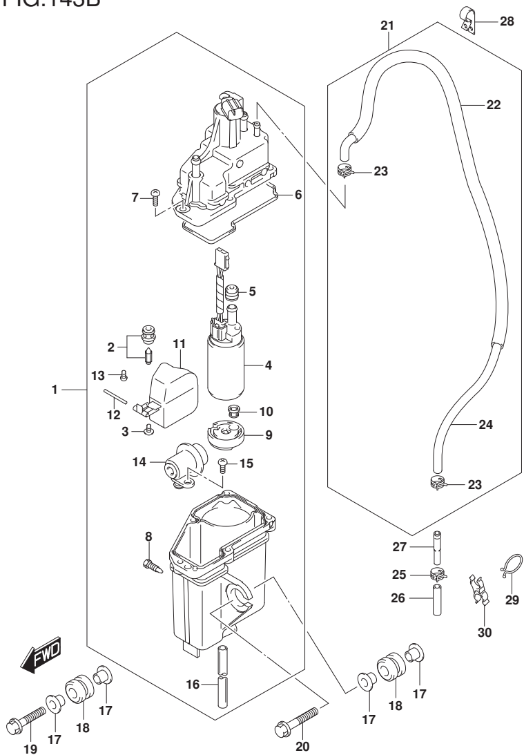
DF200A_E01_019_143B FUEL VAPOR SEPARATOR
