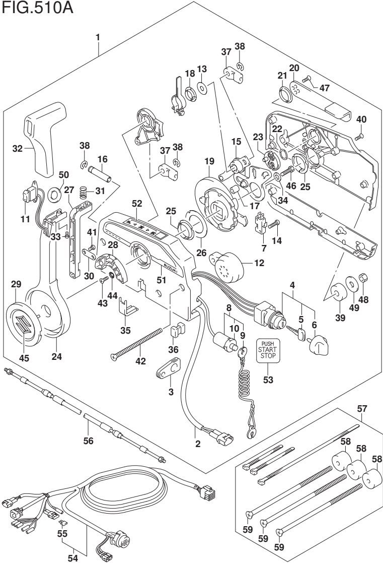
FIG.510A (1-I-9) OPT:REMOTE CONTROL (2) (W/KEY LESS START)
