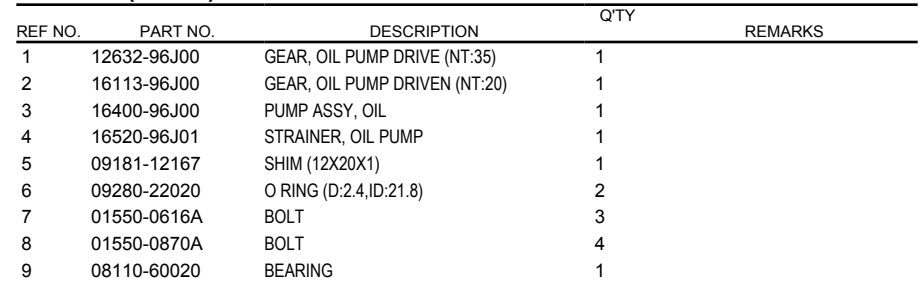
FIG.175A (1-D-10) OIL PUMP
