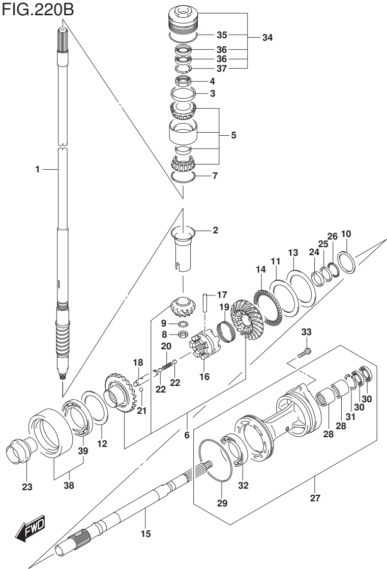
FIG.220B (1-E-8) TRANSMISSION (DF200AZ)
