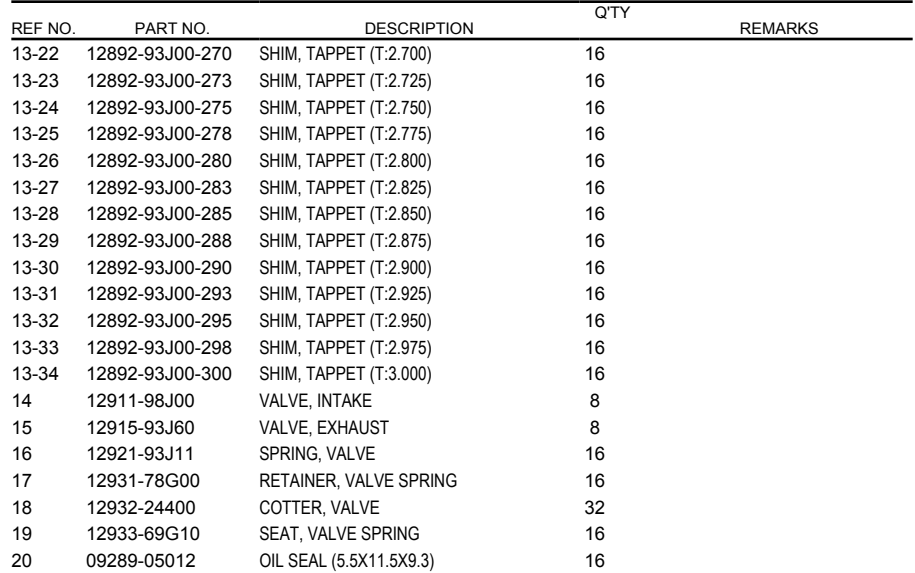
FIG.121A (1-B-11) CAMSHAFT (DF200AT)(DF200AZ)
