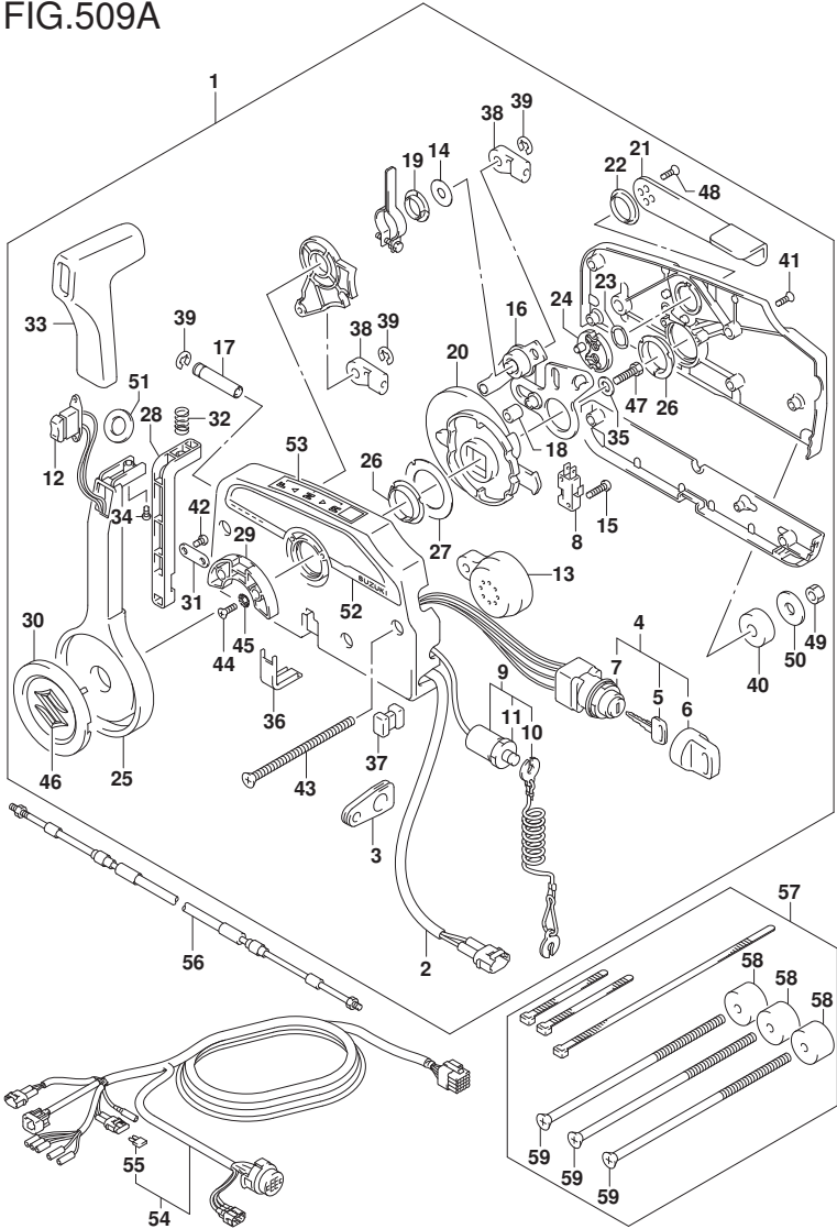
FIG.509A (1-I-8) OPT:REMOTE CONTROL (1) (N/KEY LESS START)
