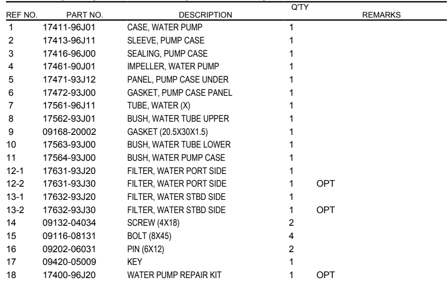
FIG.160D (1-D-5) WATER PUMP (DF200AZ E40)
