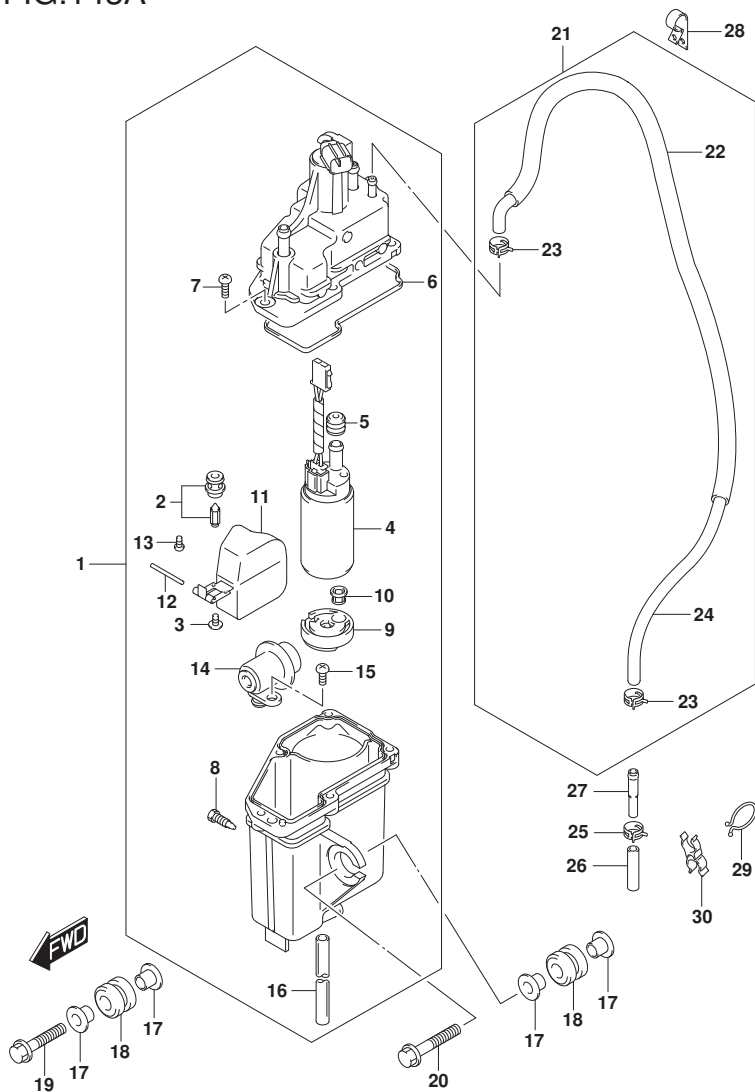
DF200A_E01_020_143A FUEL VAPOR SEPARATOR
