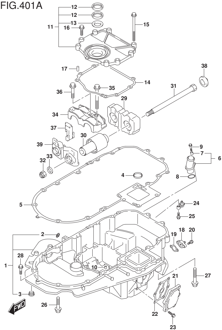
FIG.401A (1-G-6) ENGINE HOLDER
