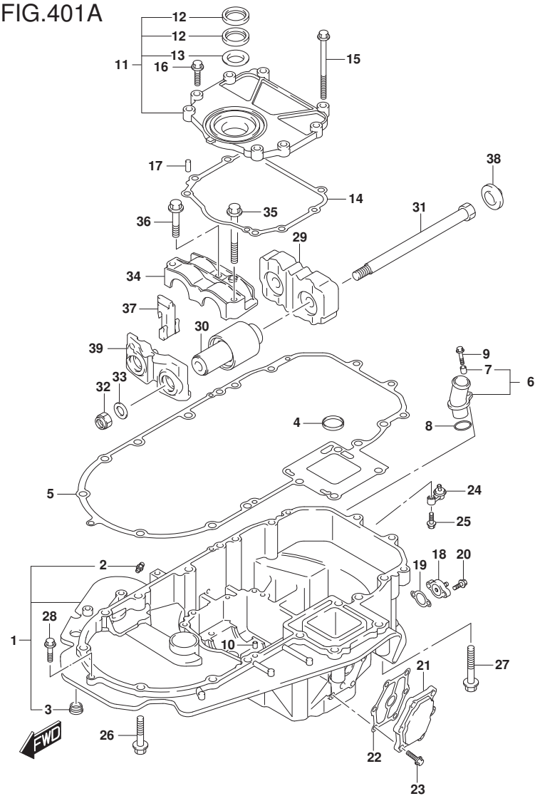
FIG.401A (1-G-7) ENGINE HOLDER
