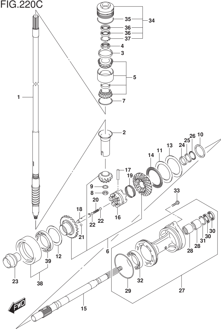
FIG.220C (1-E-11) TRANSMISSION (DF175AZ)(DF150AZ)
