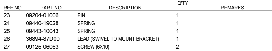
FIG.336A (1-F-14) SWIVEL BRACKET (DF200AT)(DF175AT)(DF175AZ)(DF150AT)(DF150A
