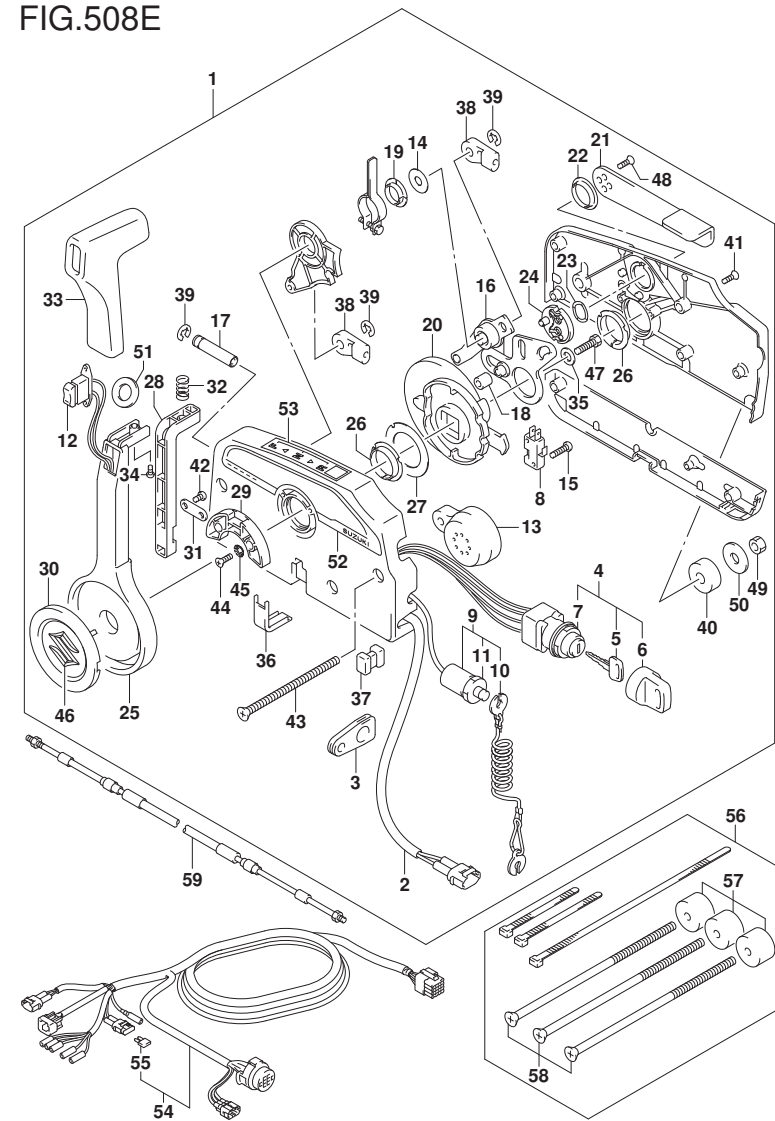
FIG.508E (1-J-7) OPT:REMOTE CONTROL (DF200AZ E40)
