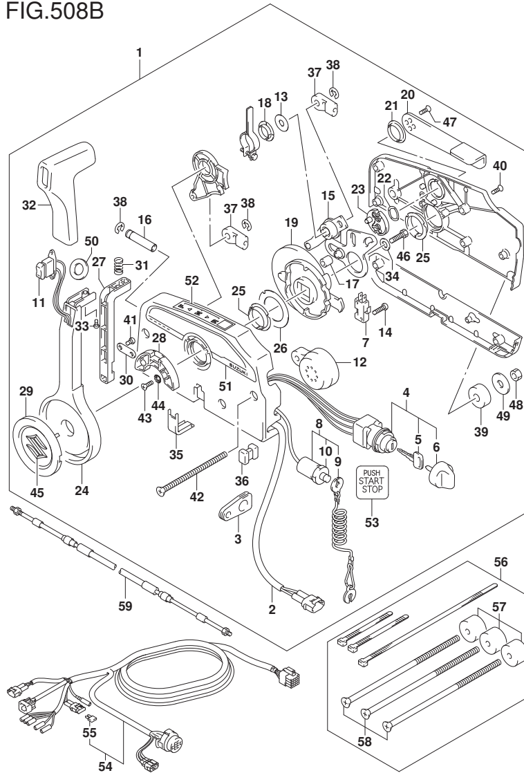
FIG.508B (1-I-11) OPT:REMOTE CONTROL (W/KEY LESS START) (DF200AT E01)
