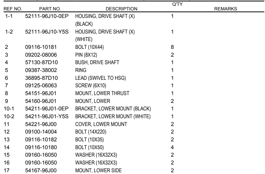
FIG.405C (1-G-6) DRIVE SHAFT HOUSING (DF200AZ E01)
