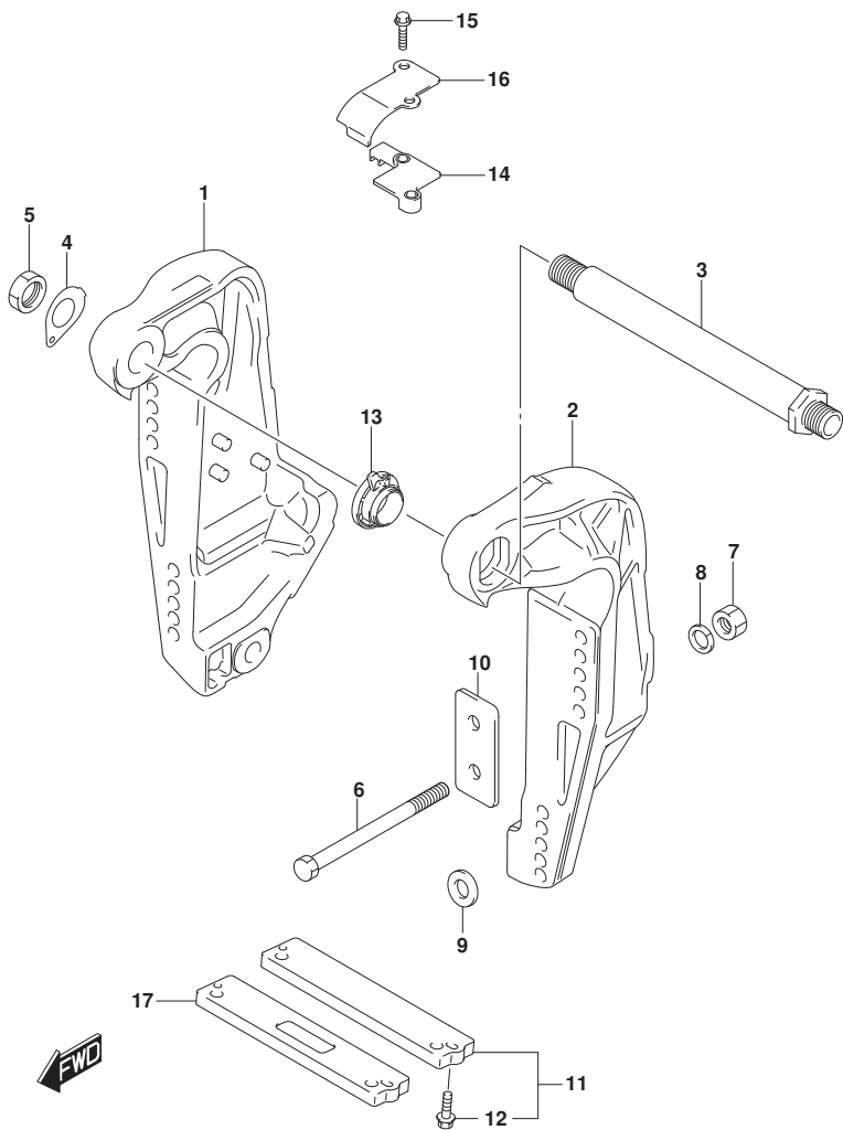
DF200A_E01_016_335A CLAMP BRACKET
