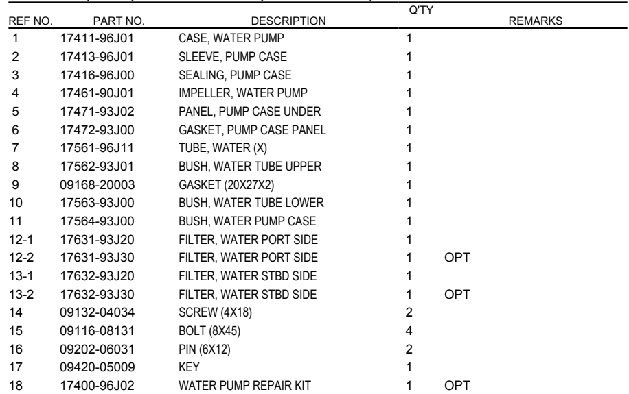
FIG.160C (1-D-2) WATER PUMP (DF200AZ E01)
