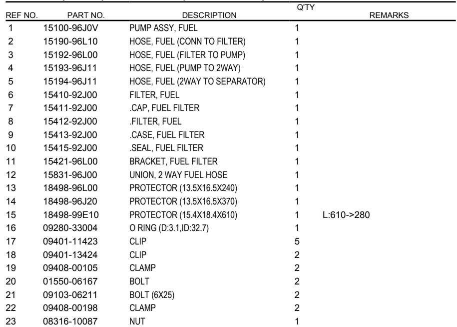
FIG.146C (1-C-12) FUEL PUMP (DF200AZ E01)
