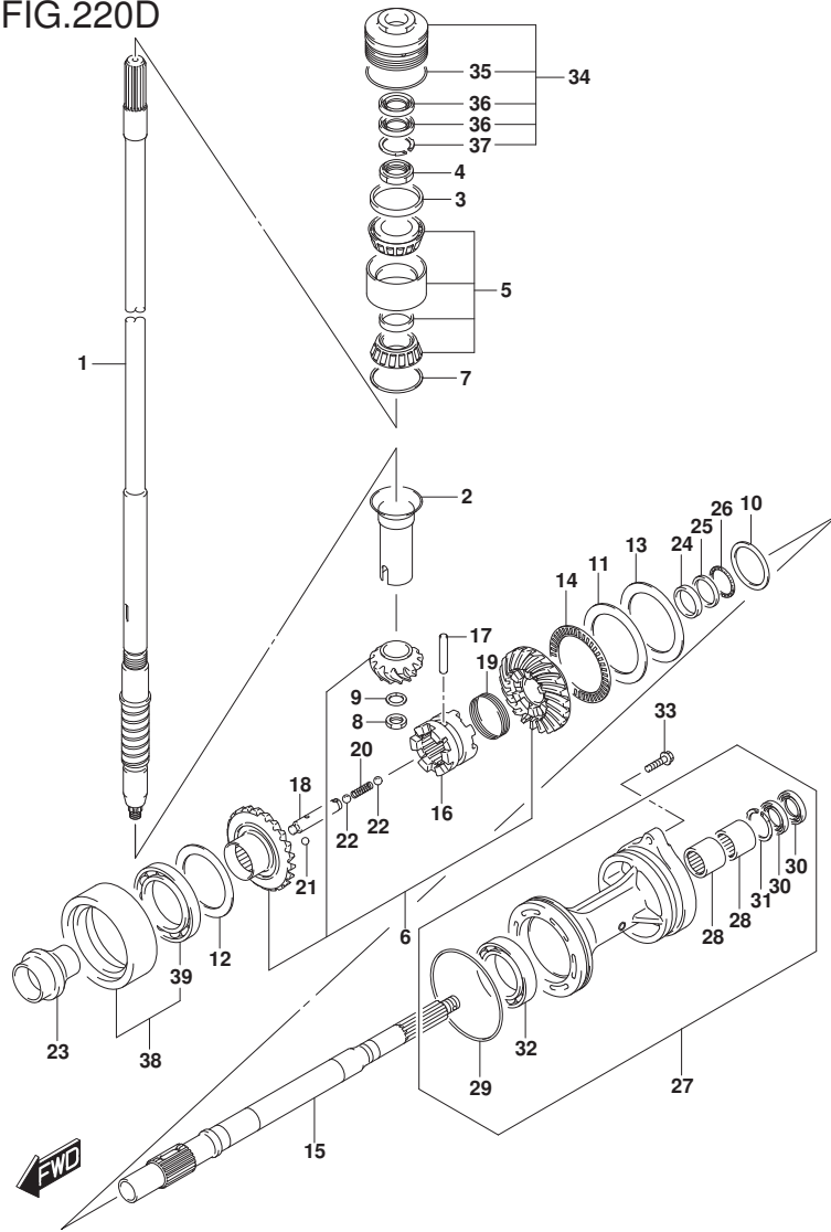
FIG.220D (1-E-12) TRANSMISSION (DF200AZ E40)
