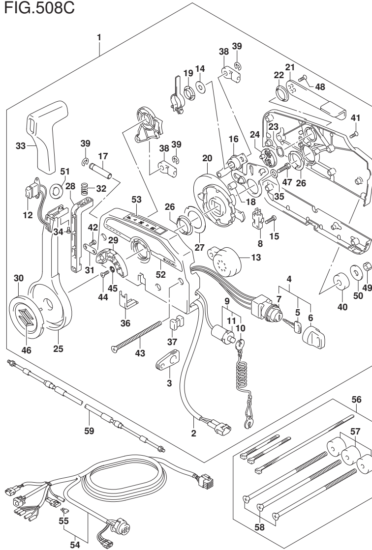
FIG.508C (1-I-13) OPT:REMOTE CONTROL (DF200AT E40)
