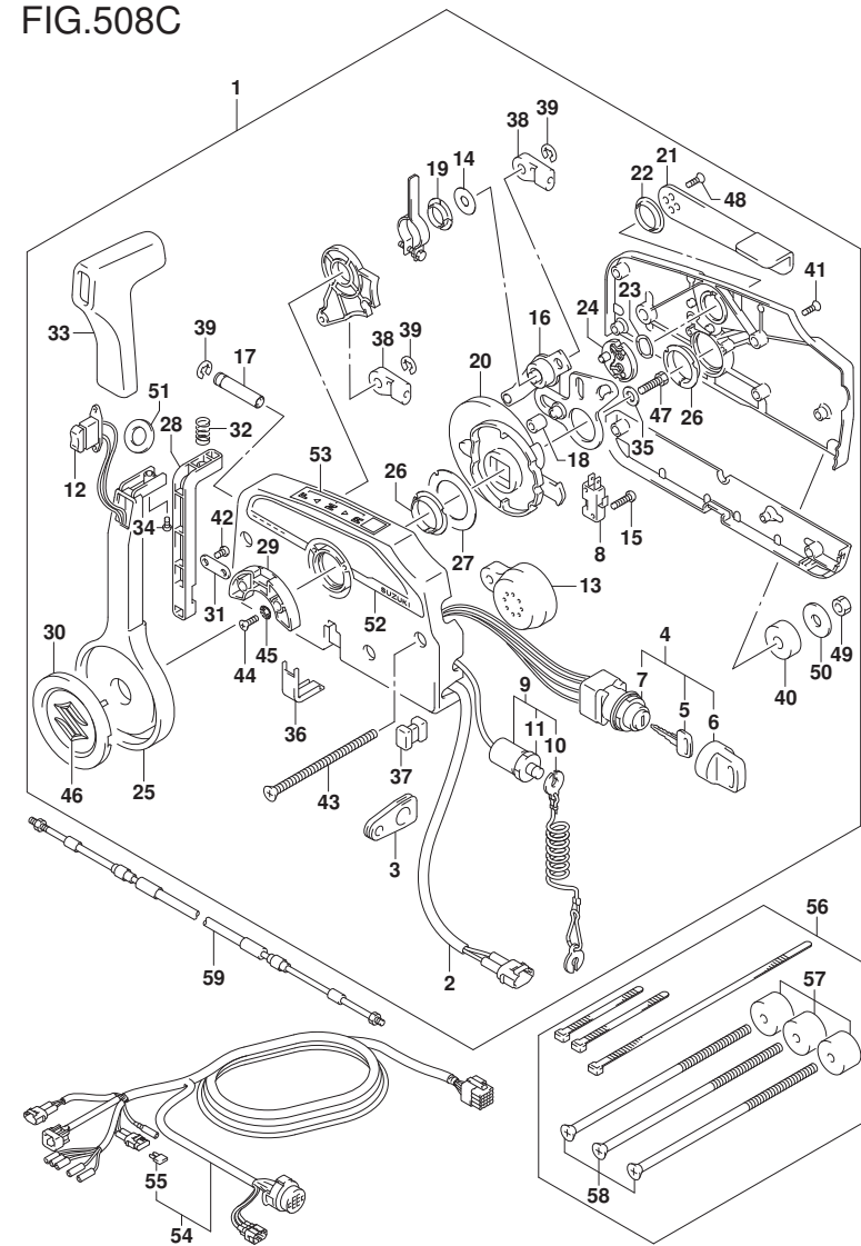
FIG.508C (1-I-15) OPT:REMOTE CONTROL (DF200AT E40)
