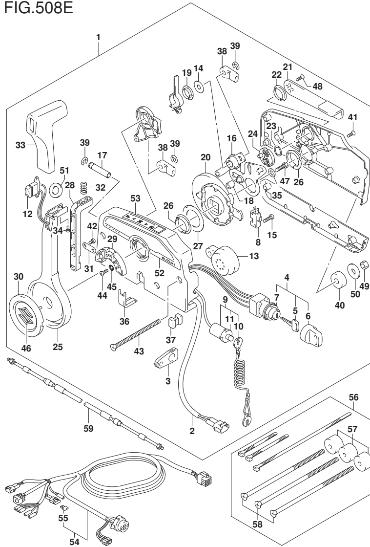
FIG.508E (1-J-6) OPT:REMOTE CONTROL (DF200AZ E40)
