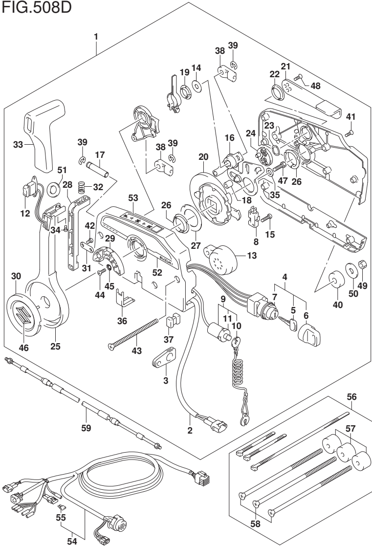
FIG.508D (1-J-5) OPT:REMOTE CONTROL (N/KEY LESS START) (DF200AZ E01)
