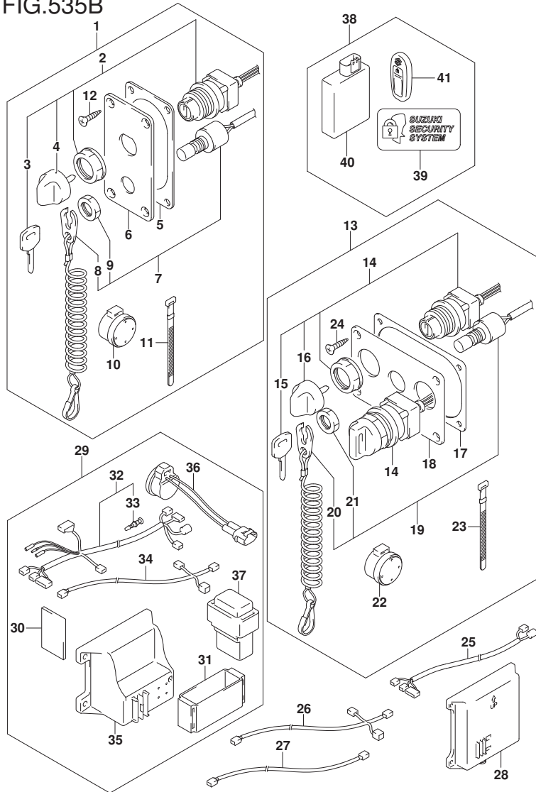
DF200A_E01_017_535B OPT:KEY LESS START
