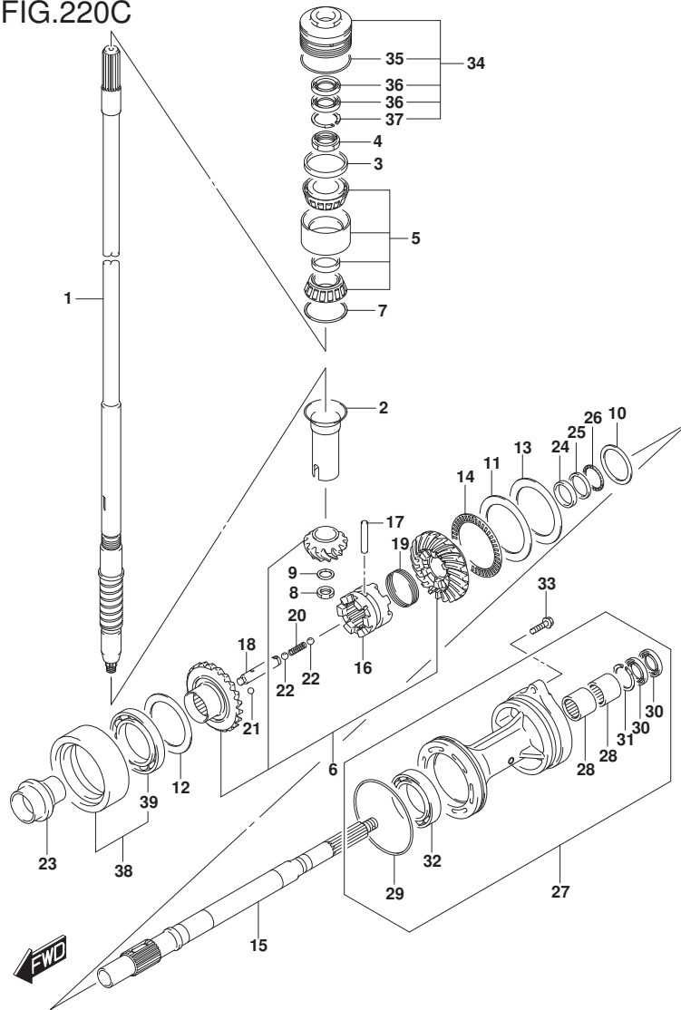
FIG.220C (1-E-11) TRANSMISSION (DF200AZ E01)
