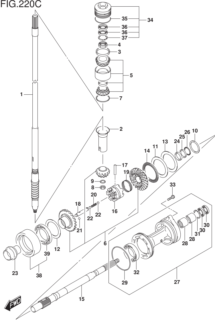
FIG.220C (1-E-10) TRANSMISSION (DF200AZ E01)
