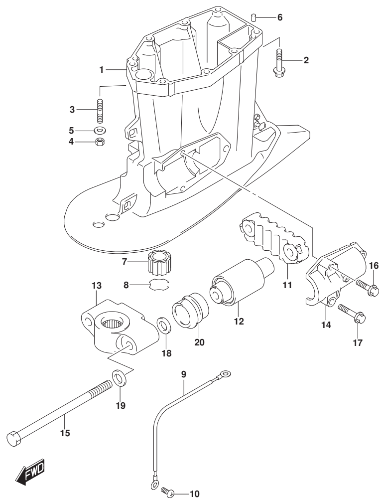
DF200A_E01_017_405B DRIVE SHAFT HOUSING
