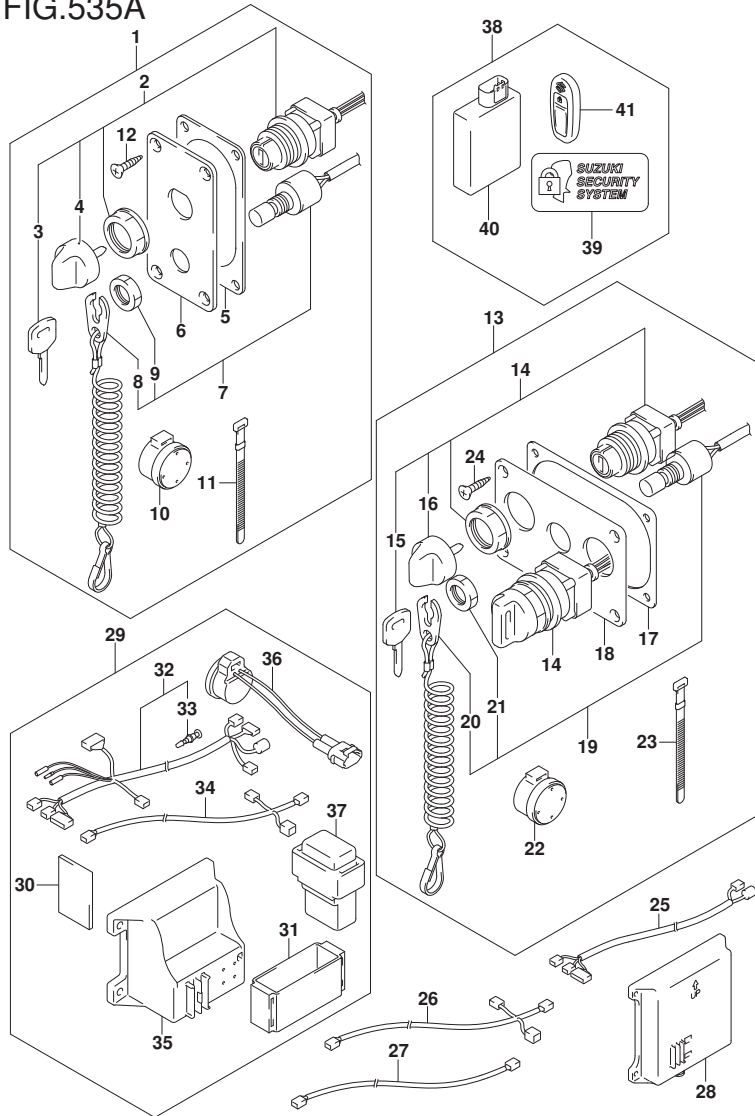
DF200A_E01_017_535A OPT:KEY LESS START
