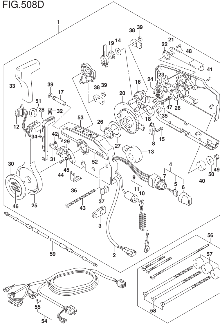
FIG.508D (1-J-4) OPT:REMOTE CONTROL (N/KEY LESS START) (DF200AZ E01)
