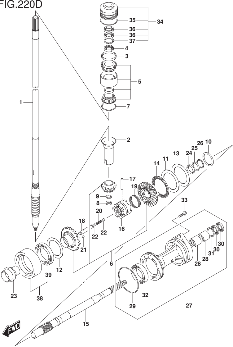
FIG.220D (1-E-15) TRANSMISSION (DF200AZ E40)
