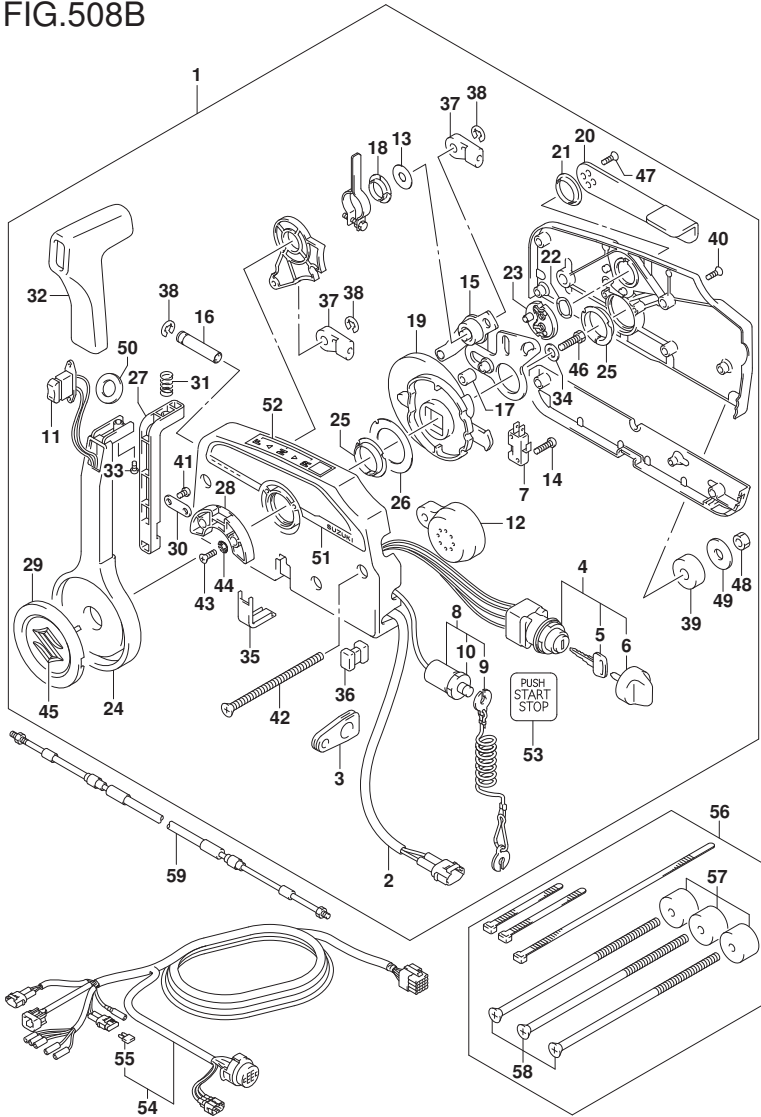
FIG.508B (1-1-12) OPT:REMOTE CONTROL (W/KEY LESS START) (DF200AT E01)
