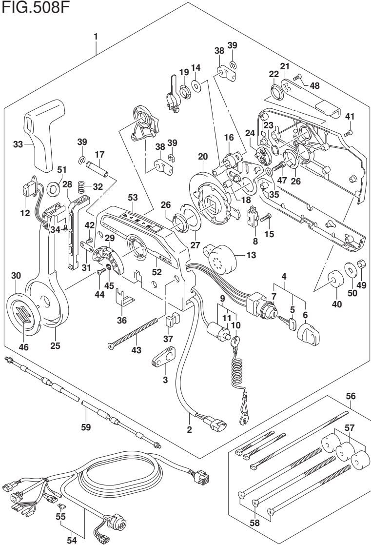
FIG.508F (1-J-12) OPT:REMOTE CONTROL (DF200AZ E40)
