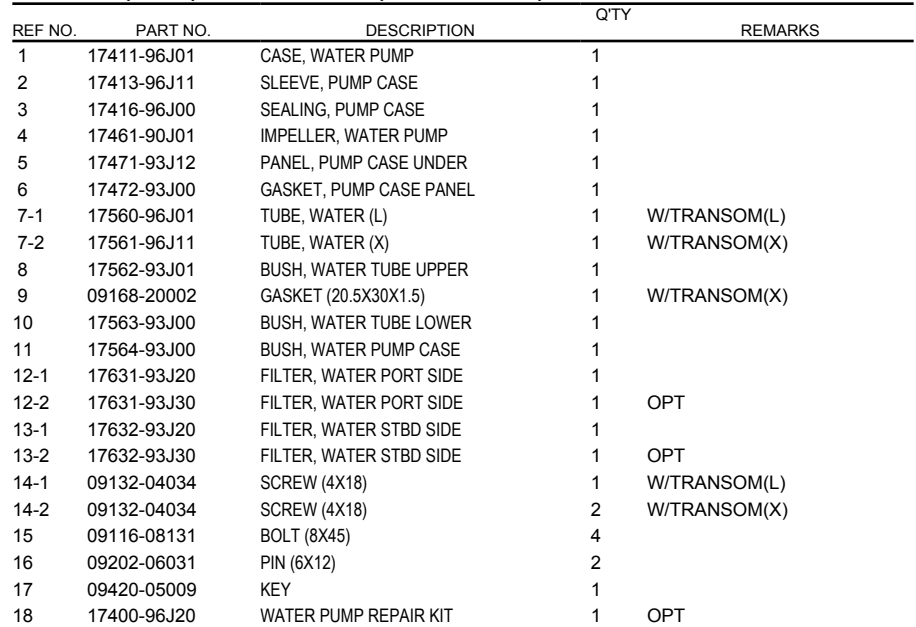
FIG.160B (1-D-2) WATER PUMP (DF200AT E40)
