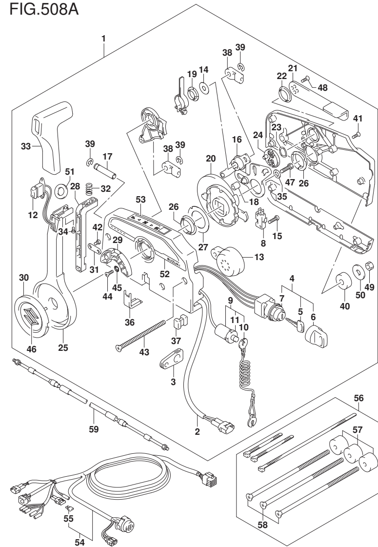
FIG.508A (1-I-11) OPT:REMOTE CONTROL (N/KEY LESS START) (DF200AT E01)
