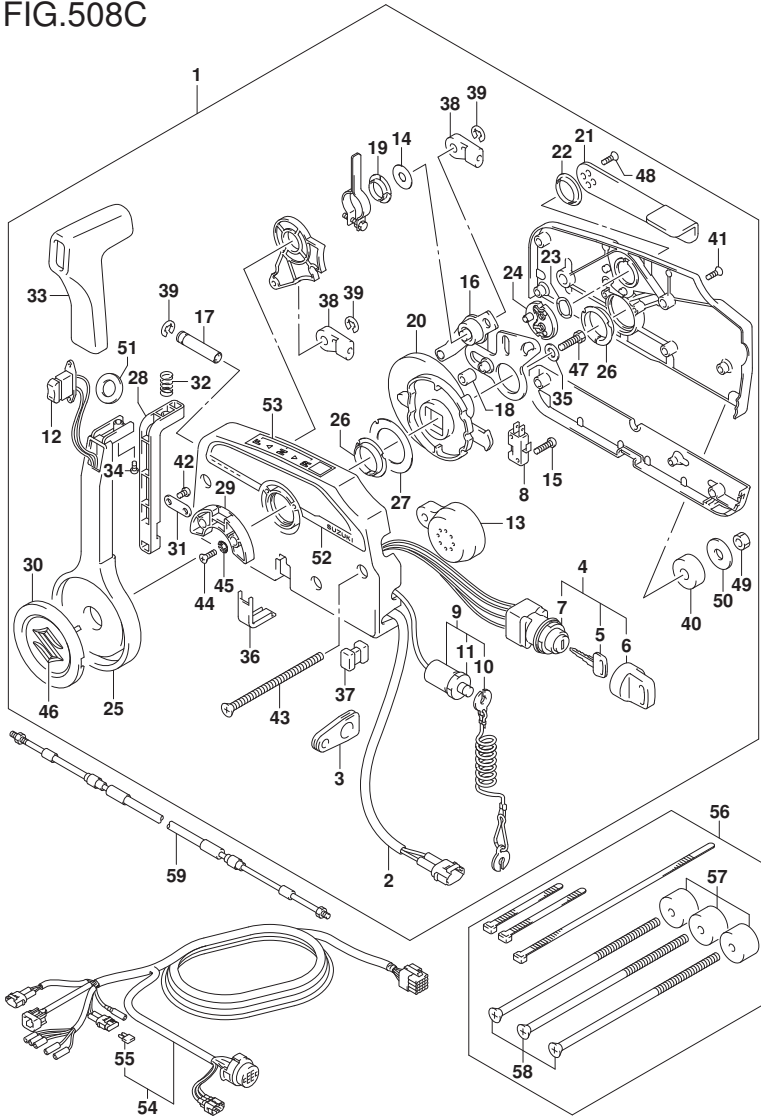
FIG.508C (1-J-3) OPT:REMOTE CONTROL (DF200AT E40)
