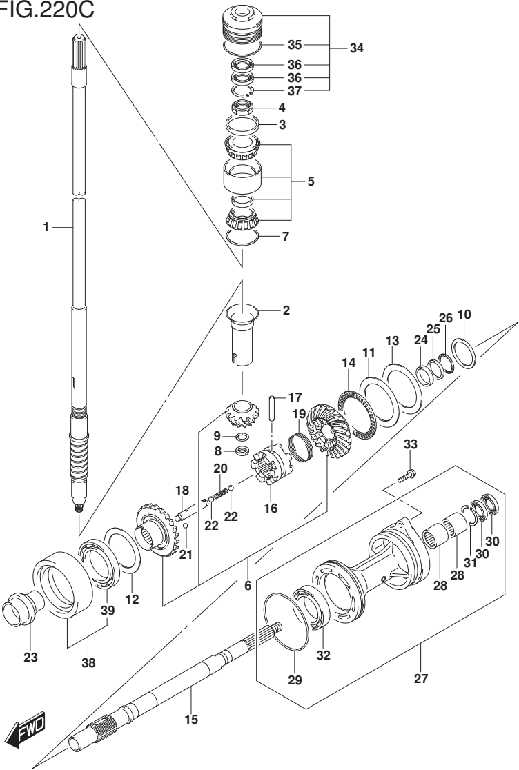
FIG.220C (1-E-12) TRANSMISSION (DF200AZ E01)
