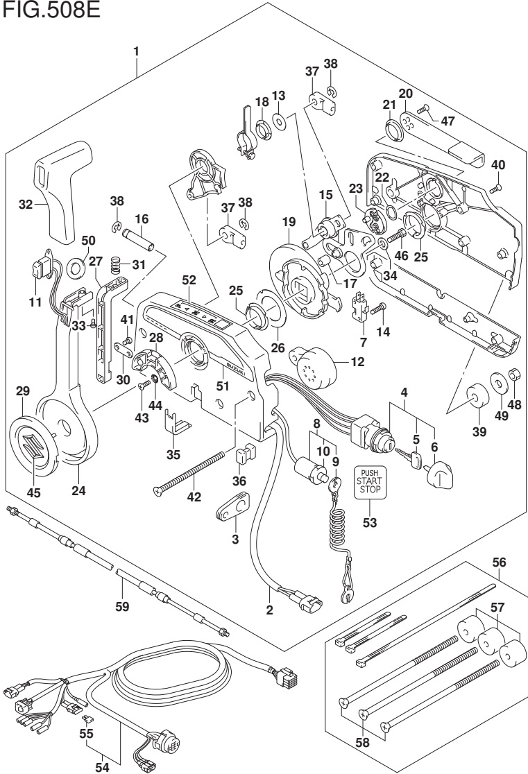
FIG.508E (1-J-7) OPT:REMOTE CONTROL (W/KEY LESS START) (DF200AZ E01)
