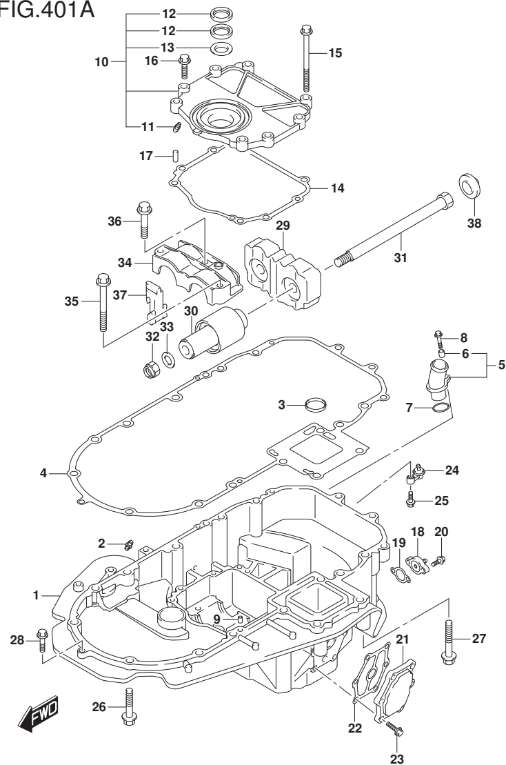
FIG.401A (1-G-5) ENGINE HOLDER
