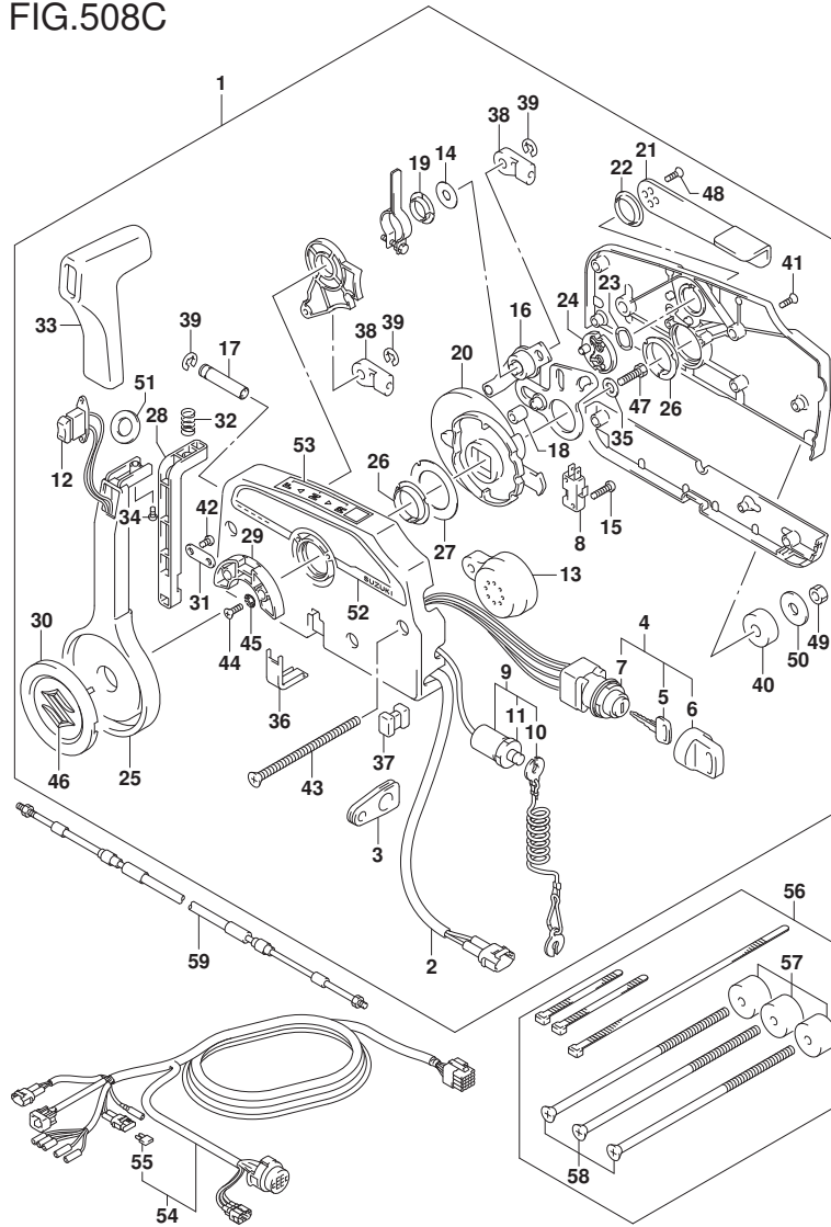
FIG.508C (1-I-15) OPT:REMOTE CONTROL (DF200AT E40)
