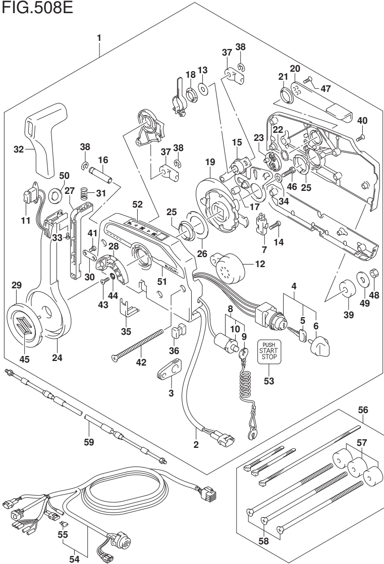
FIG.508E (1-J-8) OPT:REMOTE CONTROL (W/KEY LESS START) (DF200AZ E01)
