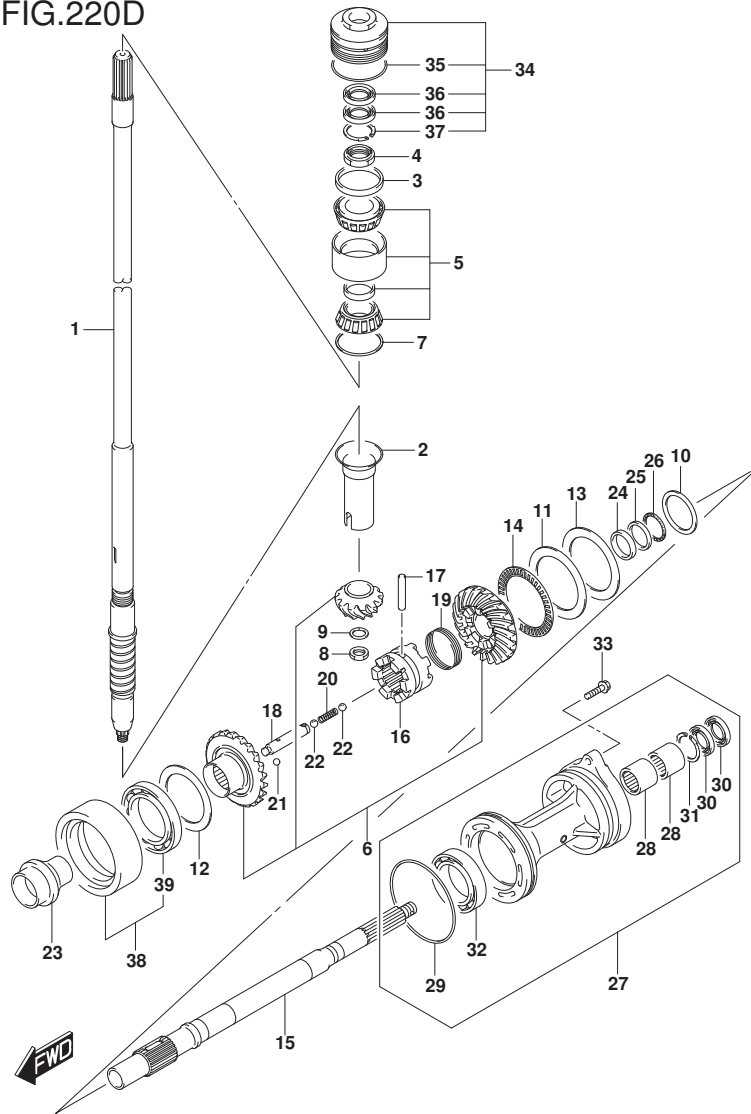
FIG.220D (1-E-14) TRANSMISSION (DF200AZ E40)
