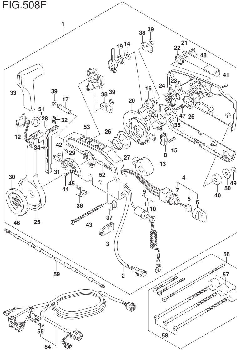
FIG.508F (1-J-10) OPT:REMOTE CONTROL (DF200AZ E40)
