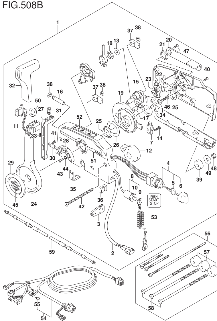
FIG.508B (1-I-13) OPT:REMOTE CONTROL (W/KEY LESS START) (DF200AT E01)
