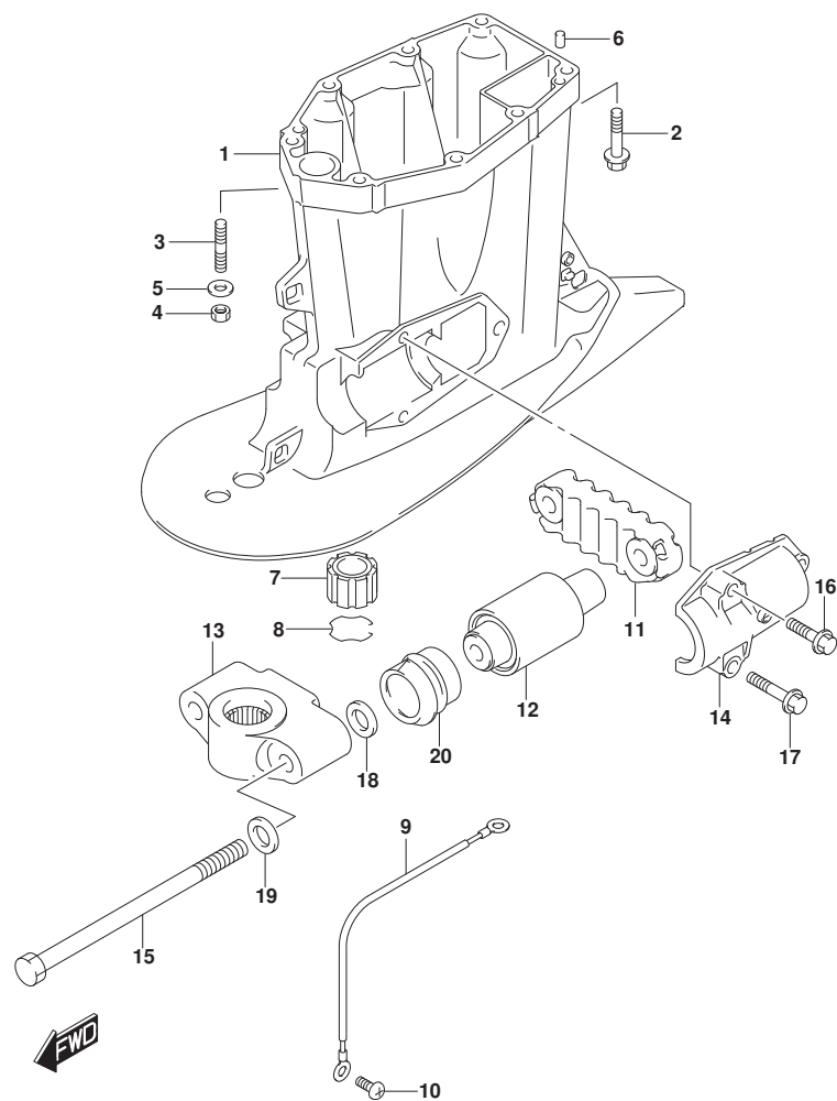
DF200A_E01_017_405A DRIVE SHAFT HOUSING
