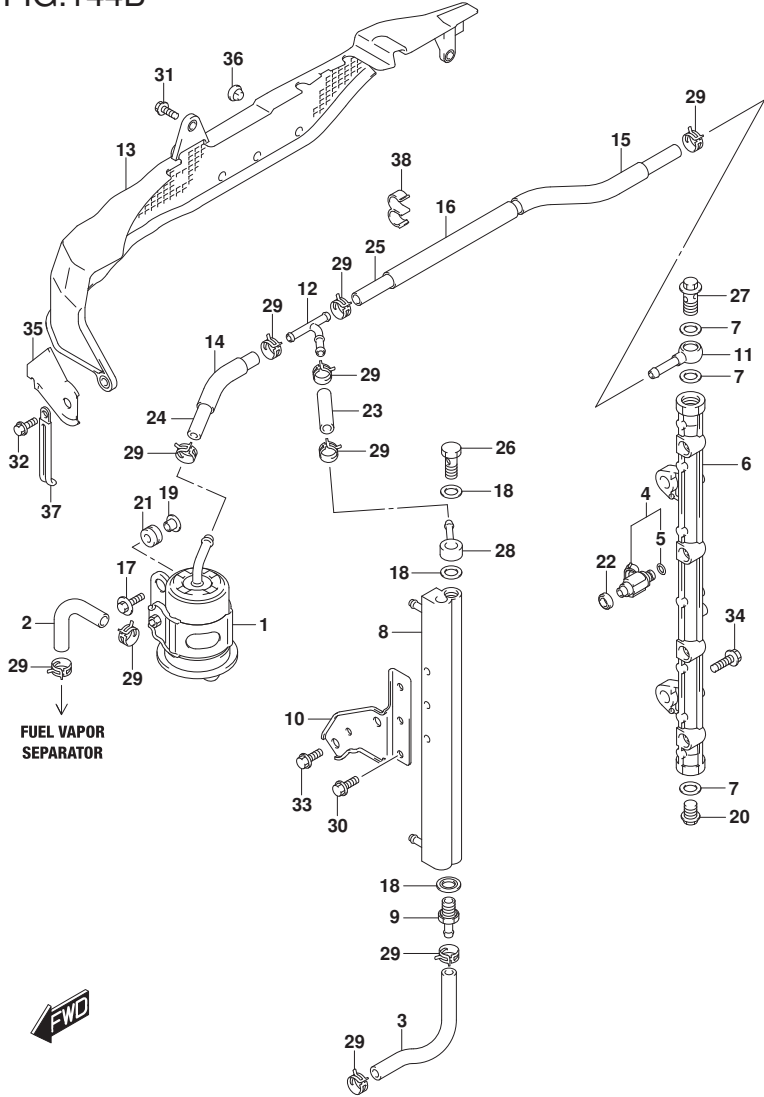
DF200A_E01_017_144B FUEL INJECTOR
