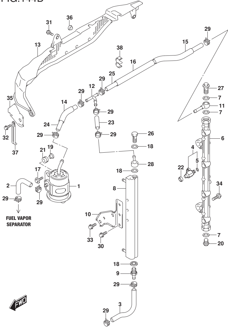
DF200A_E01_017_144D FUEL INJECTOR
