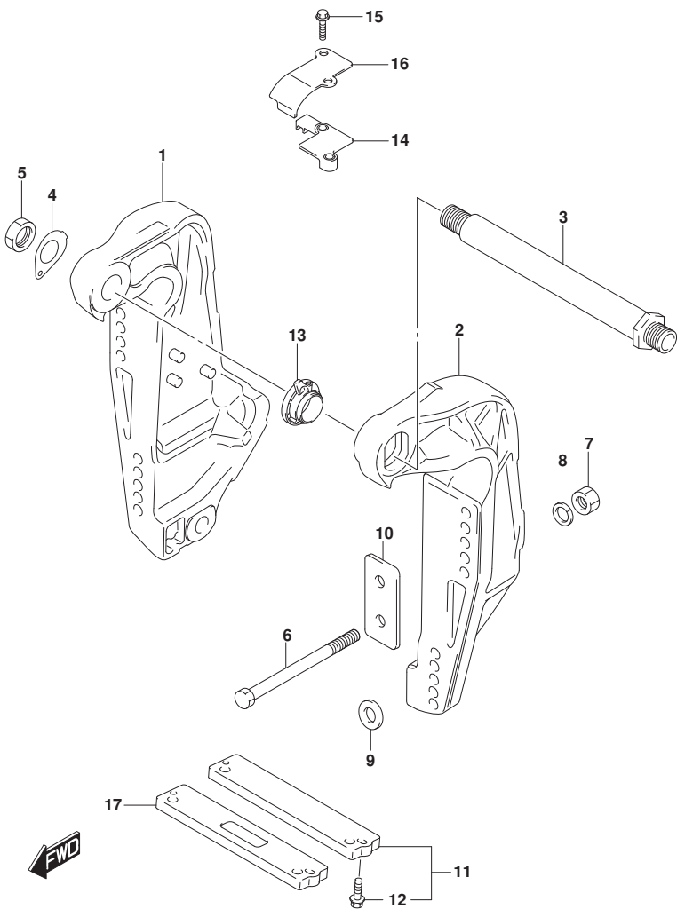
DF200A_E01_018_335A CLAMP BRACKET
