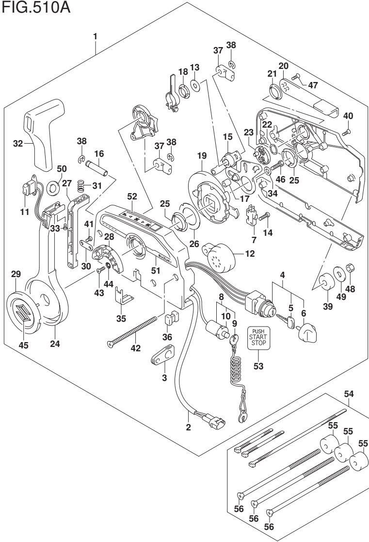
FIG.510A (1-G-9) OPT:REMOTE CONTROL (2) (W/KEY LESS START)
