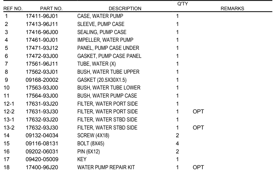
FIG.160D (1-C-12) WATER PUMP (DF200AZ E40)
