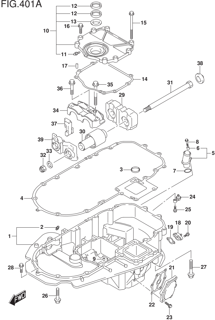
FIG.401A (1-F-3) ENGINE HOLDER
