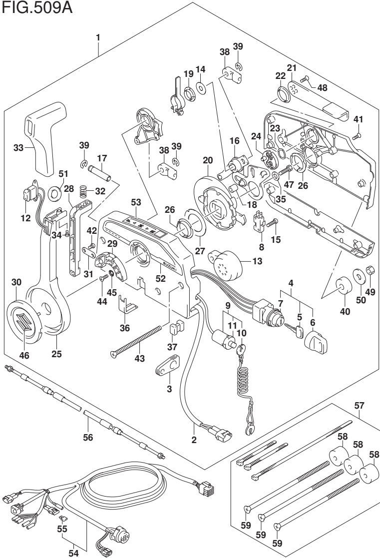
FIG.509A (1-G-6) OPT:REMOTE CONTROL (1) (N/KEY LESS START)
