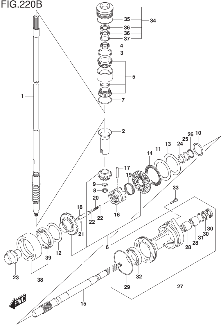
FIG.220B (1-D-12) TRANSMISSION (DF200AZ)
