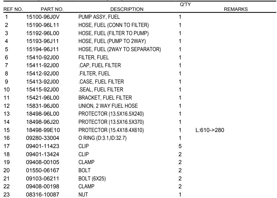
FIG.146A (1-C-7) FUEL PUMP (E01)
