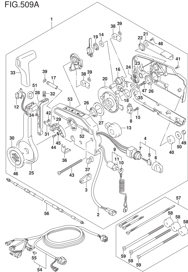
FIG.509A (1-G-7) OPT:REMOTE CONTROL (1) (N/KEY LESS START)
