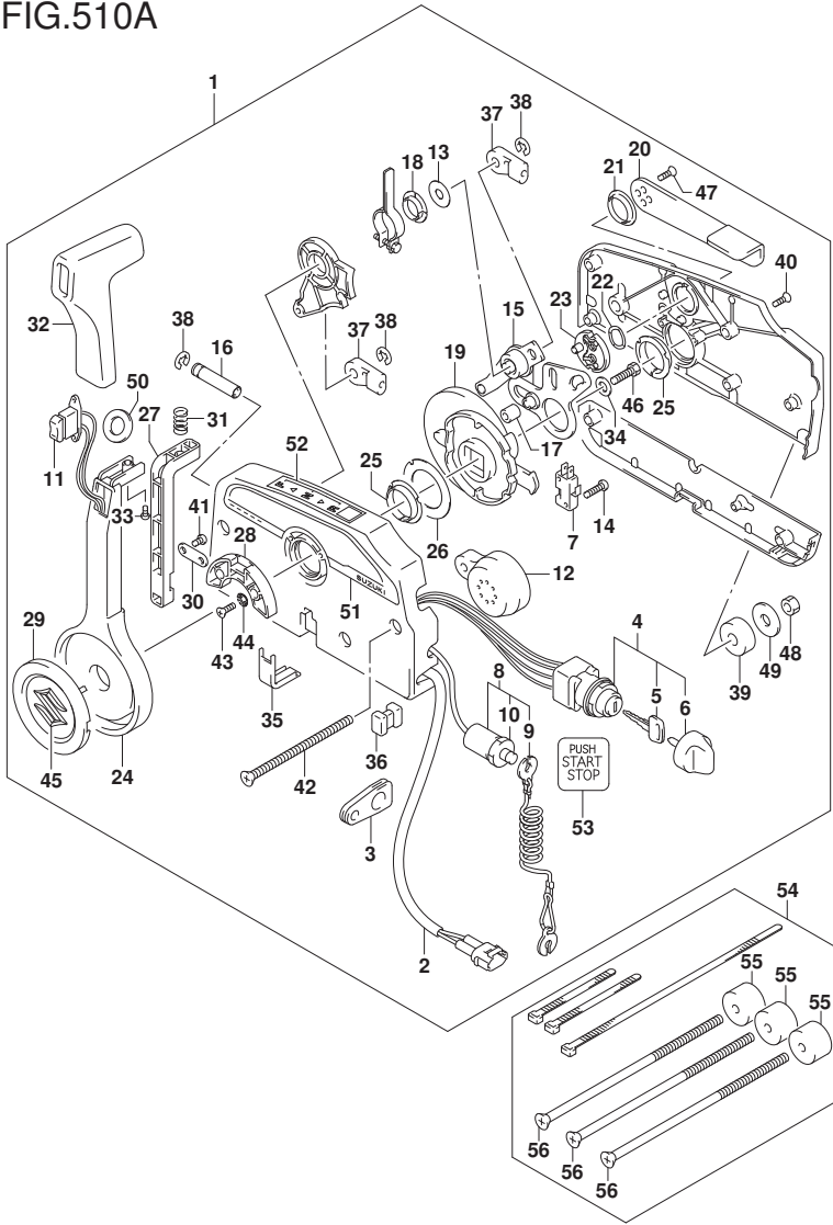
FIG.510A (1-G-10) OPT:REMOTE CONTROL (2) (W/KEY LESS START)
