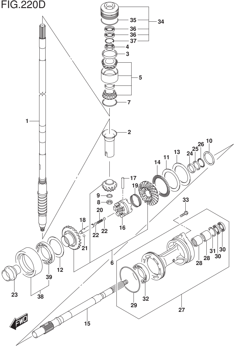
FIG.220D (1-F-10) TRANSMISSION (DF200Z E40)
