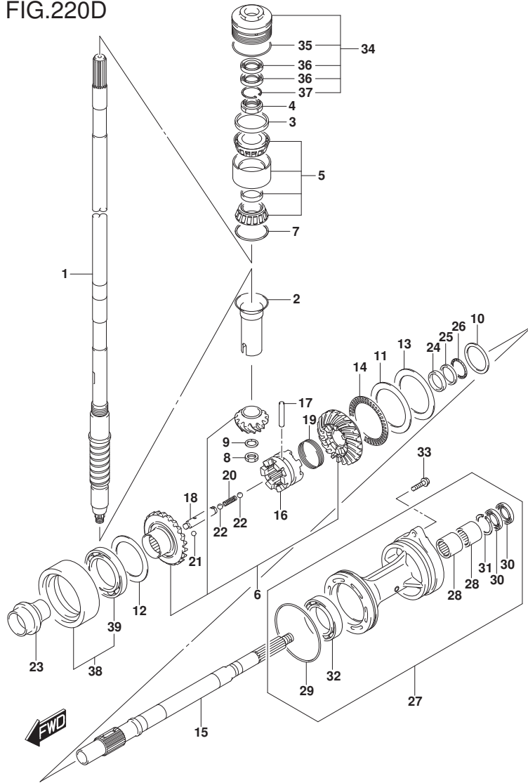
FIG.220D (1-F-11) TRANSMISSION (DF200Z E40)
