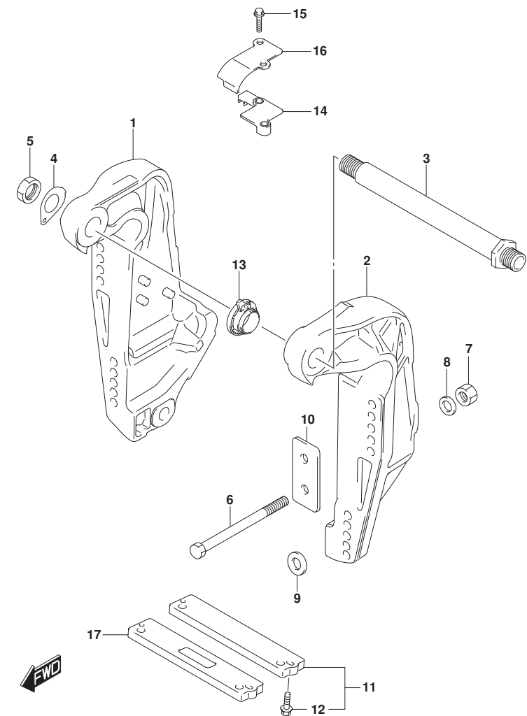
DF250_E01_018_335A CLAMP BRACKET
