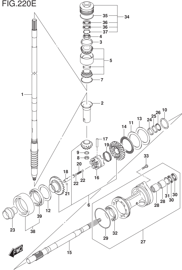
FIG.220E (1-F-14) TRANSMISSION (DF225Z)(DF250Z)
