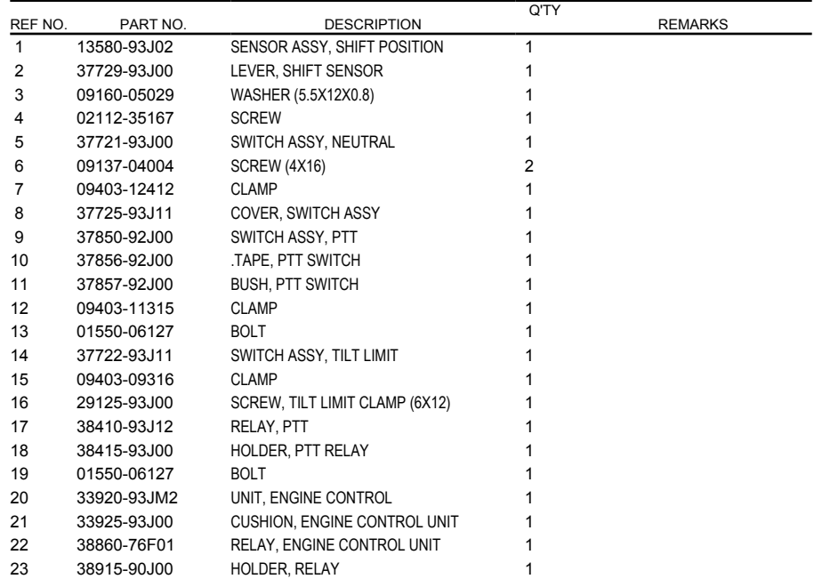
FIG.326C (1-H-6) PTT SWITCH/ENGINE CONTROL UNIT (DF200Z)
