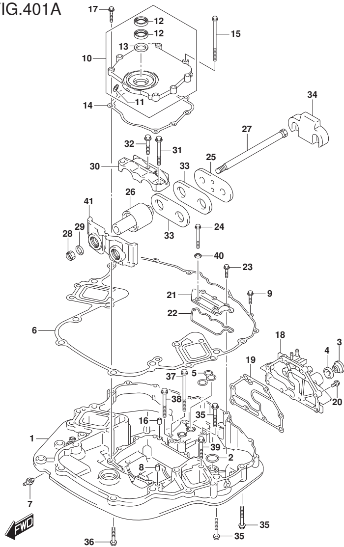
DF250_E01_018_401A ENGINE HOLDER
