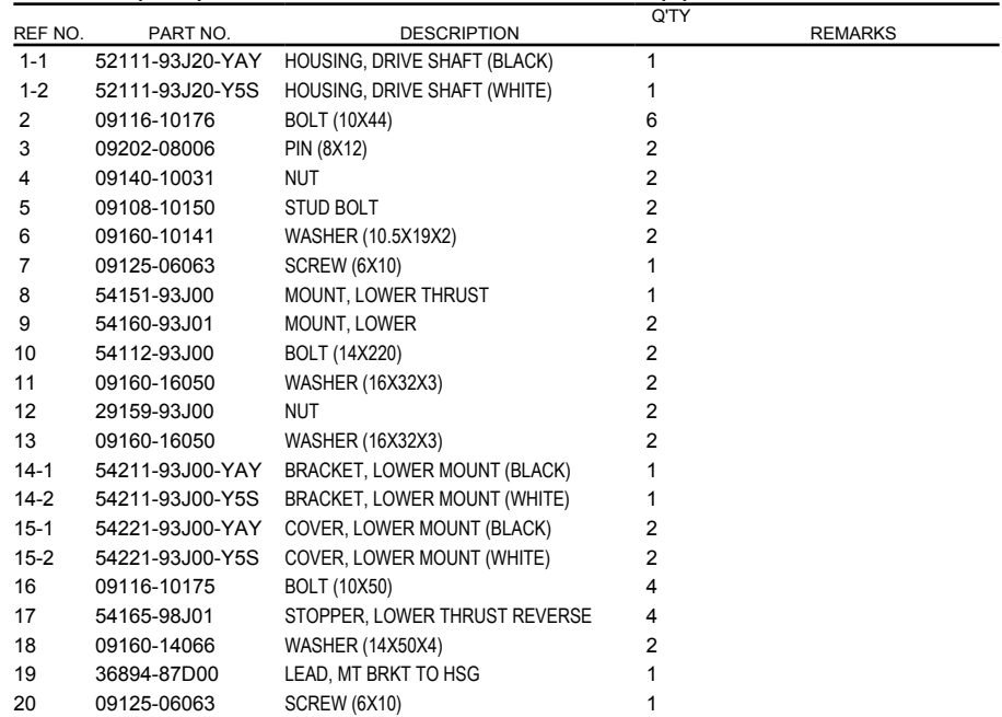
FIG.405A (1-I-9) DRIVE SHAFT HOUSING TRANSOM(L)
