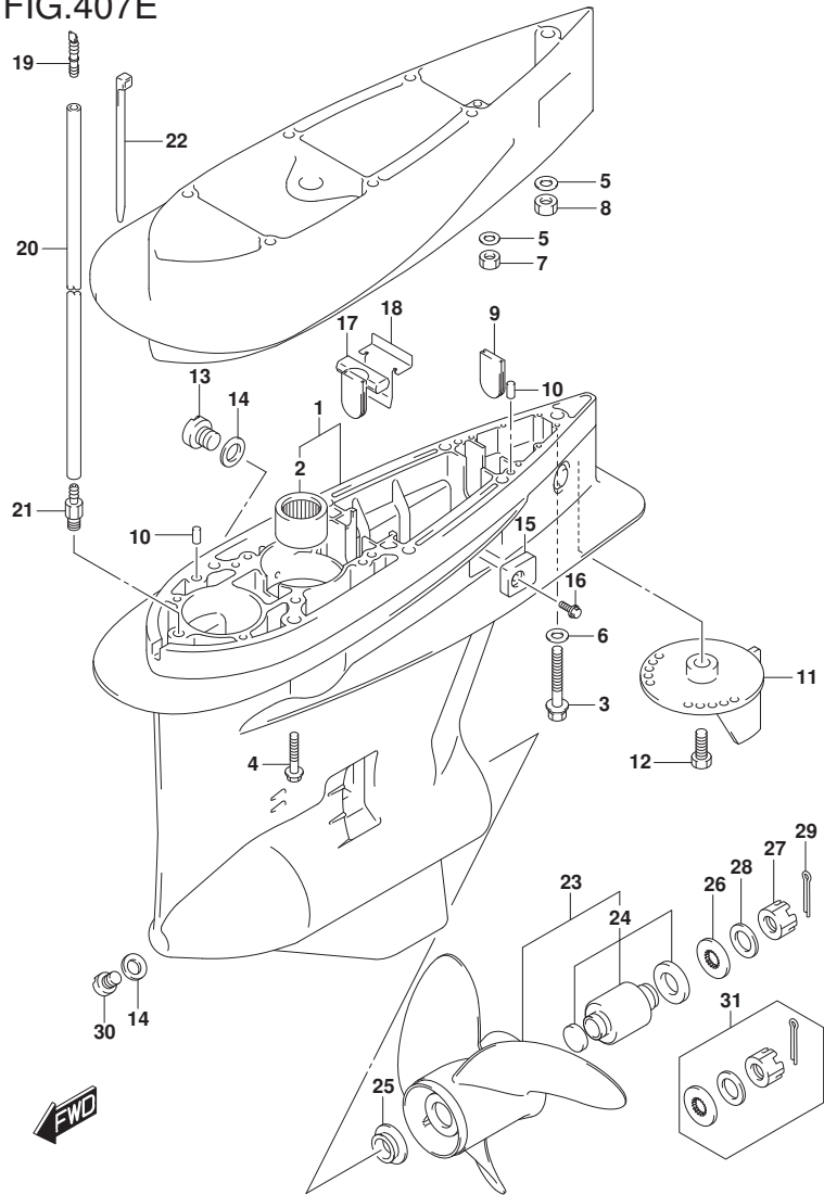
DF250_E01_018_407E GEAR CASE
