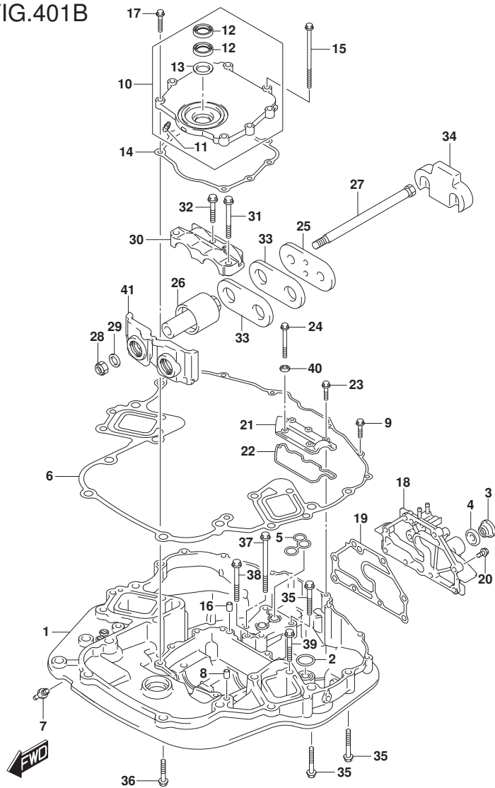
DF250_E01_018_401B ENGINE HOLDER
