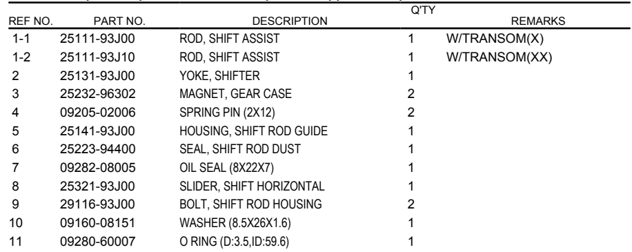
FIG.206E (1-E-14) CLUTCH ROD (DF225Z)(DF250Z)
