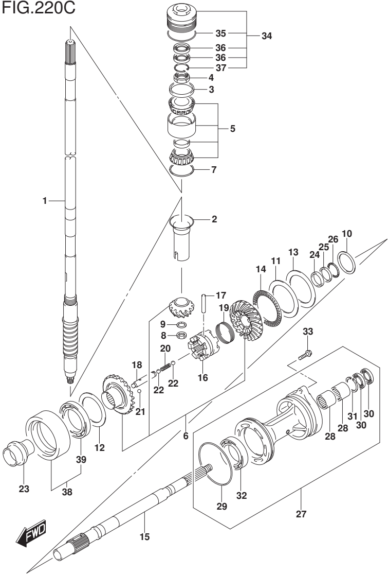
FIG.220C (1-F-9) TRANSMISSION (DF200Z E01)
