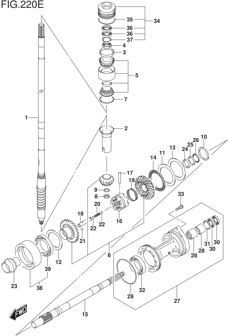
FIG.220E (1-F-13) TRANSMISSION (DF225Z)(DF250Z)
