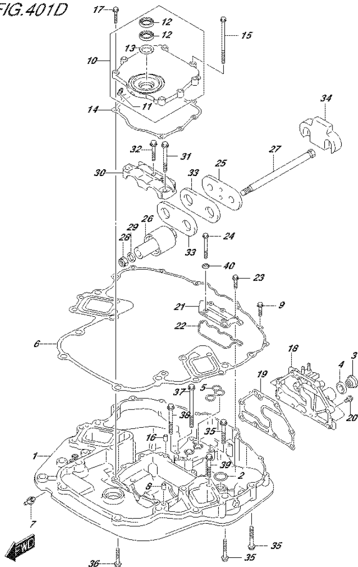
FIG.401D (3-C-9) ENGINE HOLDER (DF200Z E40)
