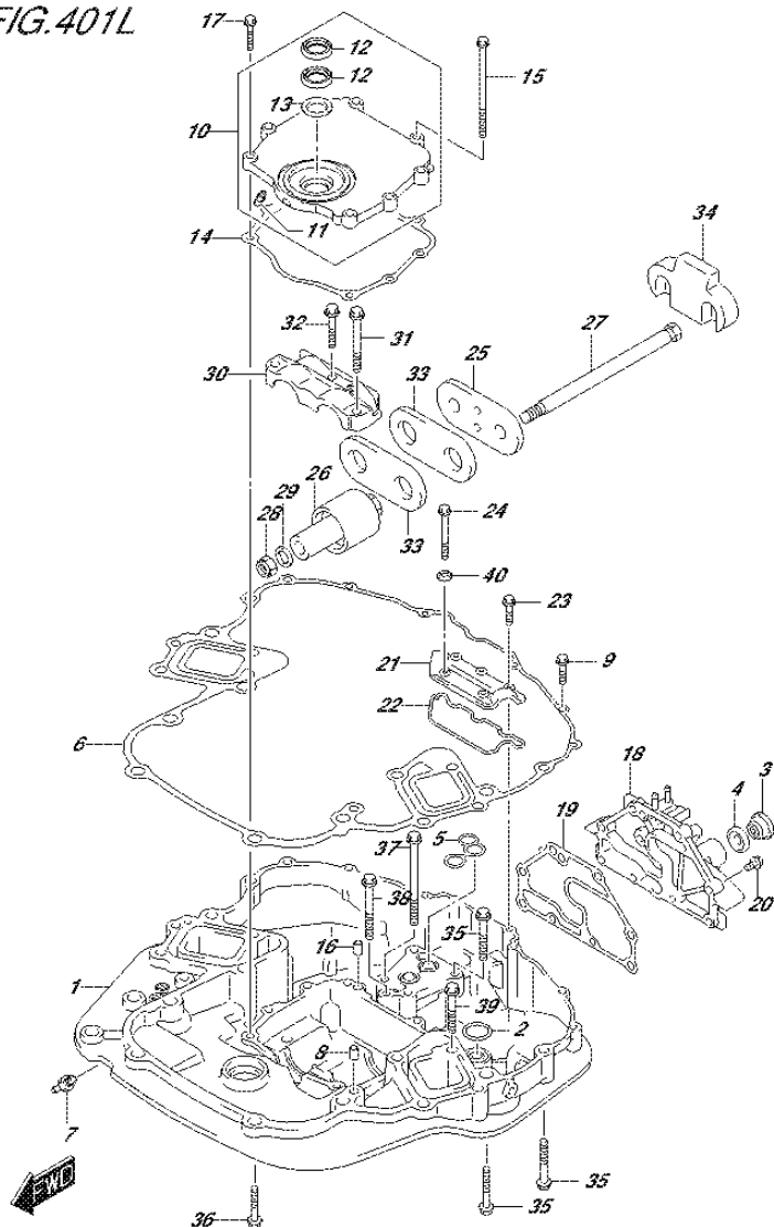
FIG.401L (3-D-9) ENGINE HOLDER (DF250Z E01)
