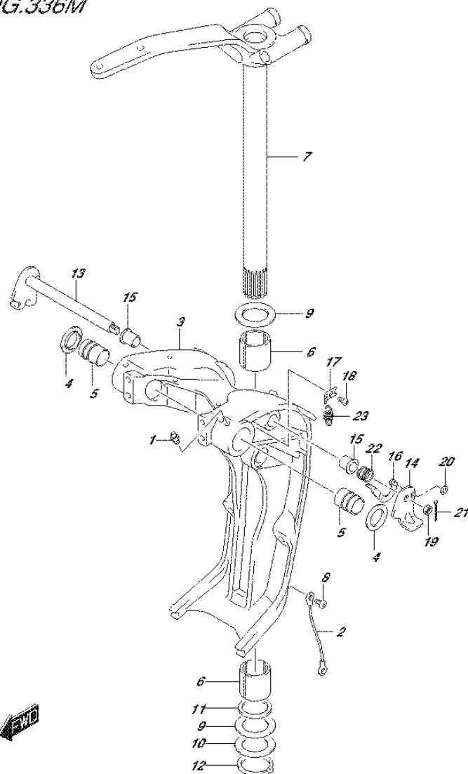
DF250_E01_016_336M SWIVEL BRACKET
