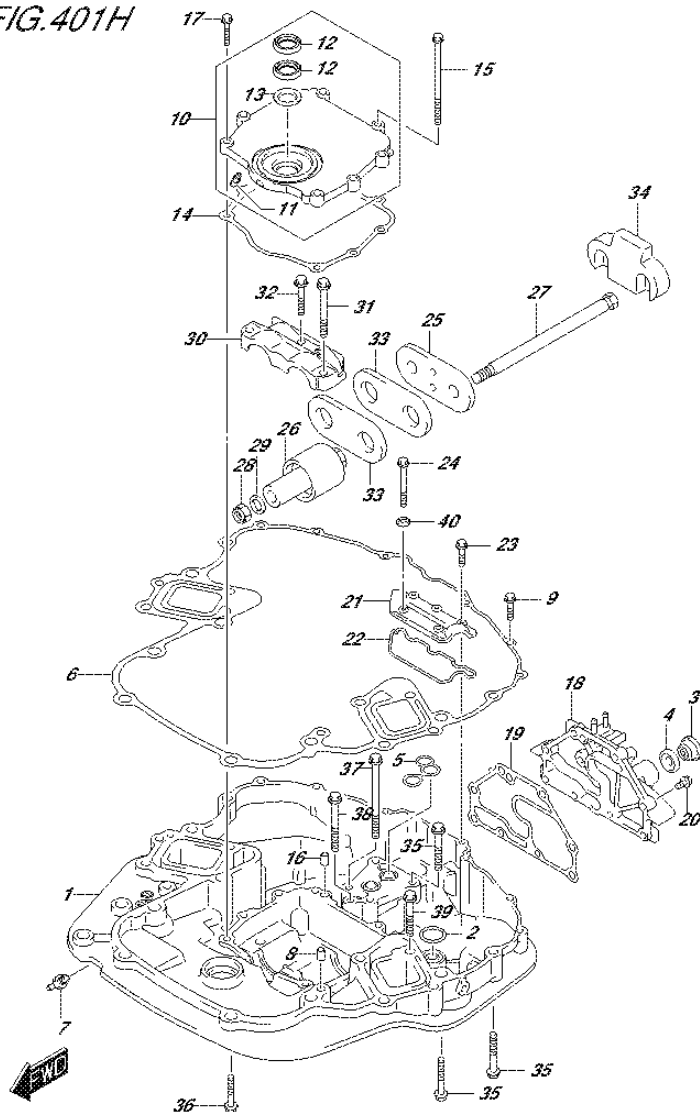
FIG.401H (3-D-2) ENGINE HOLDER (DF225Z E40)
