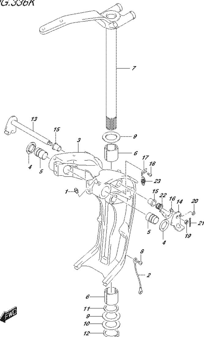
DF250_E01_016_336K SWIVEL BRACKET
