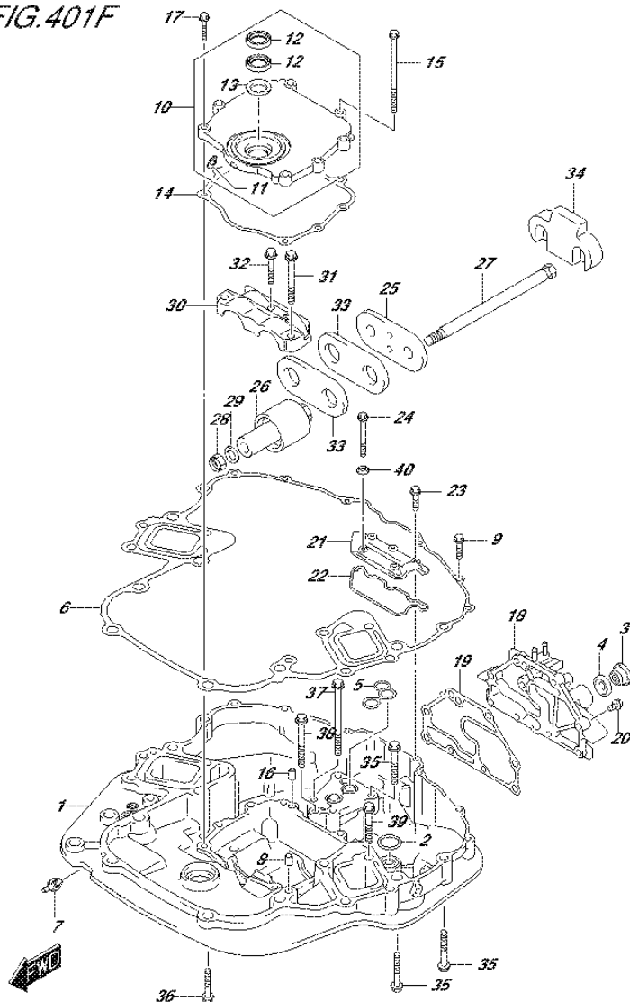
FIG.401F (3-C-12) ENGINE HOLDER (DF225T E40)
