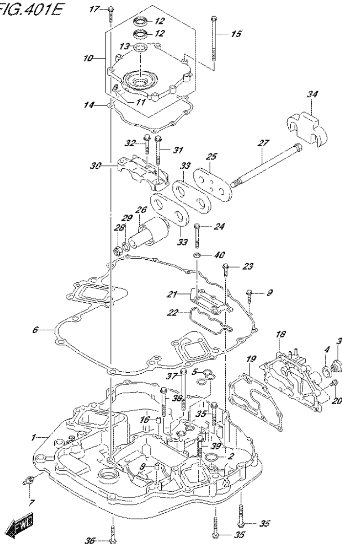
FIG.401E (3-C-10) ENGINE HOLDER (DF25T E01)
