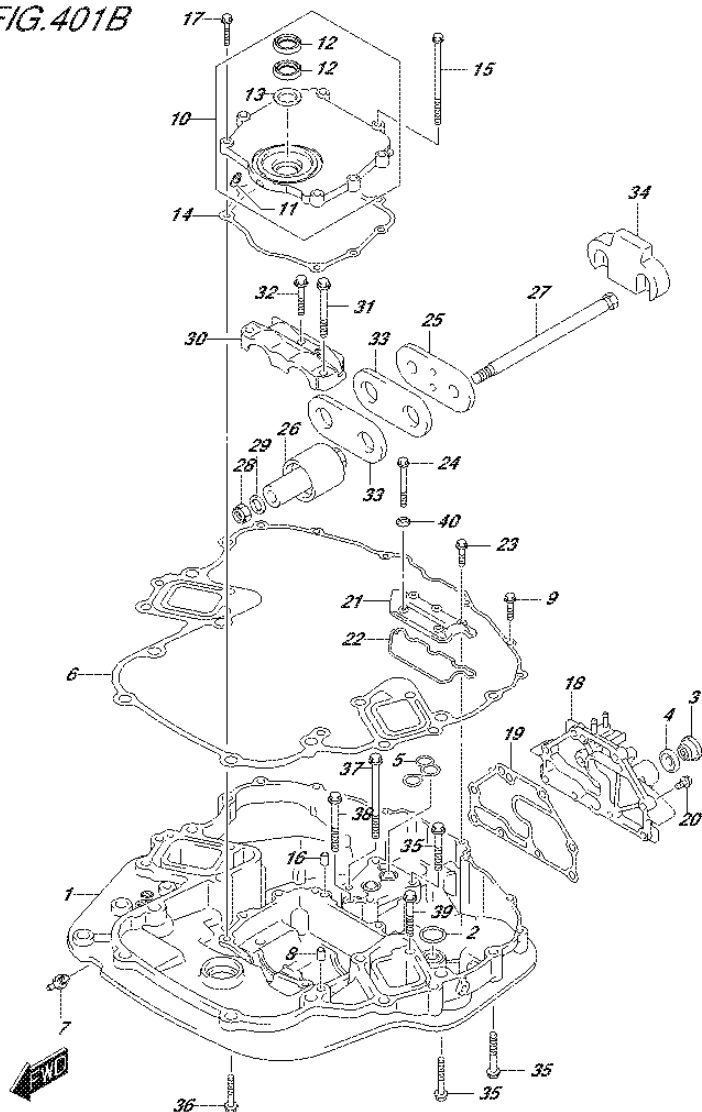
FIG.401B (3-C-5) ENGINE HOLDER (DF200T E40)
