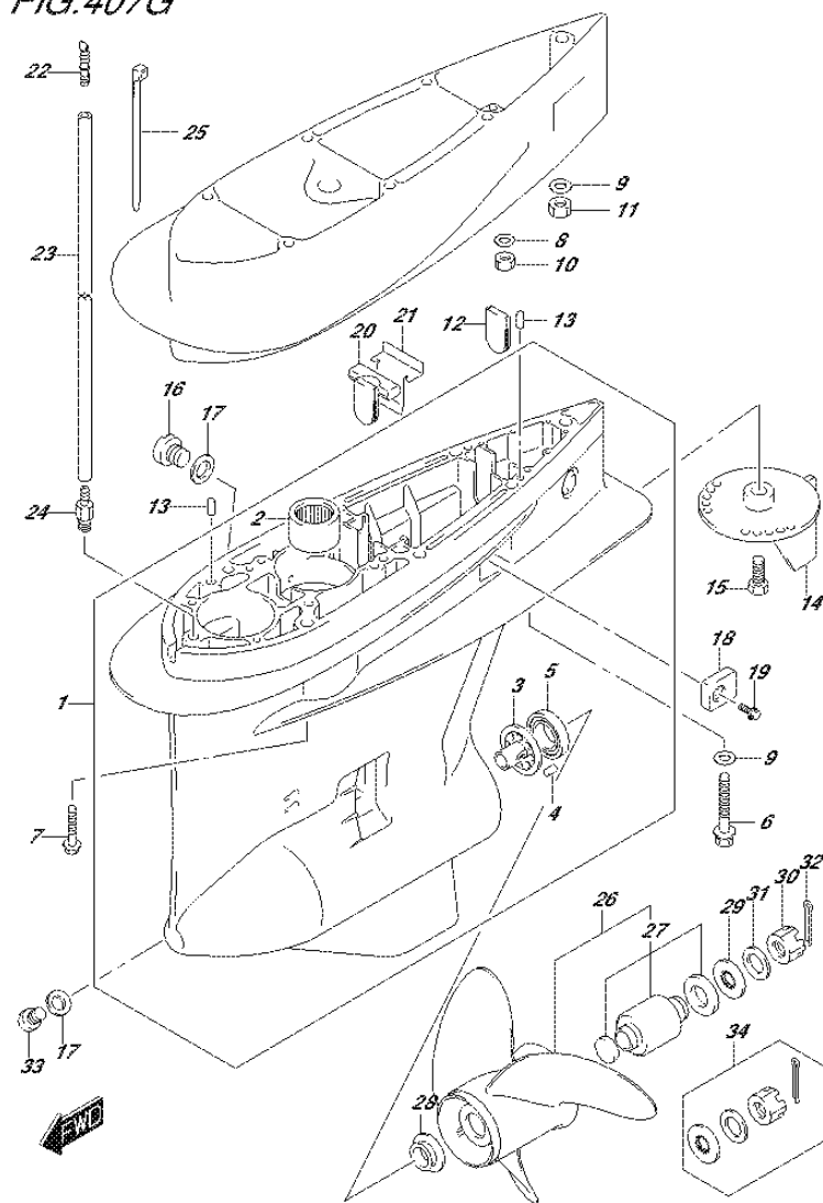
DF250_E01_016_407G GEAR CASE
