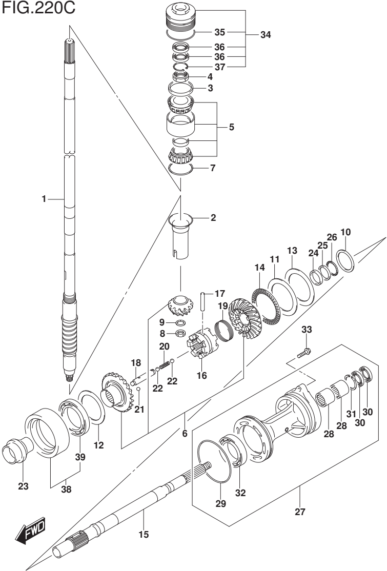
FIG.220C (1-F-10) TRANSMISSION (DF200Z E01)
