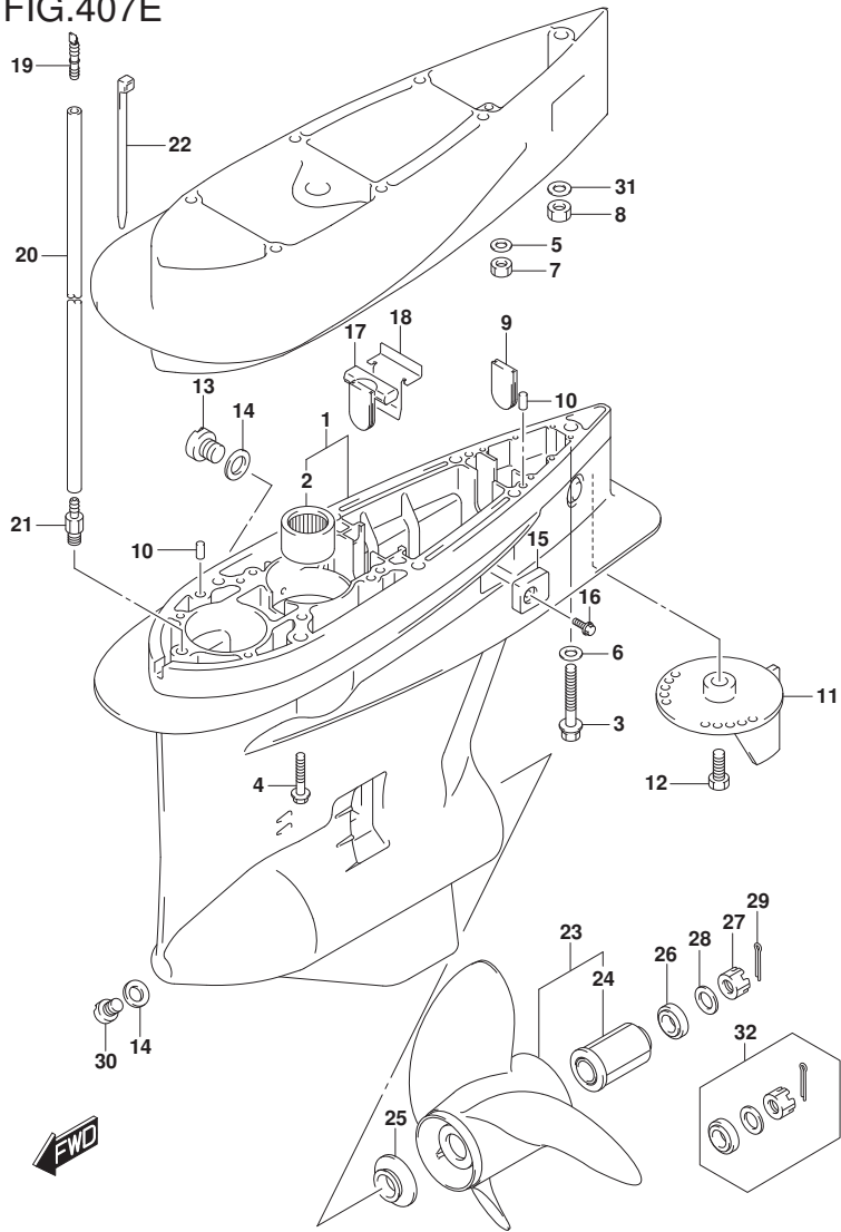
DF250_E01_019_407E GEAR CASE
