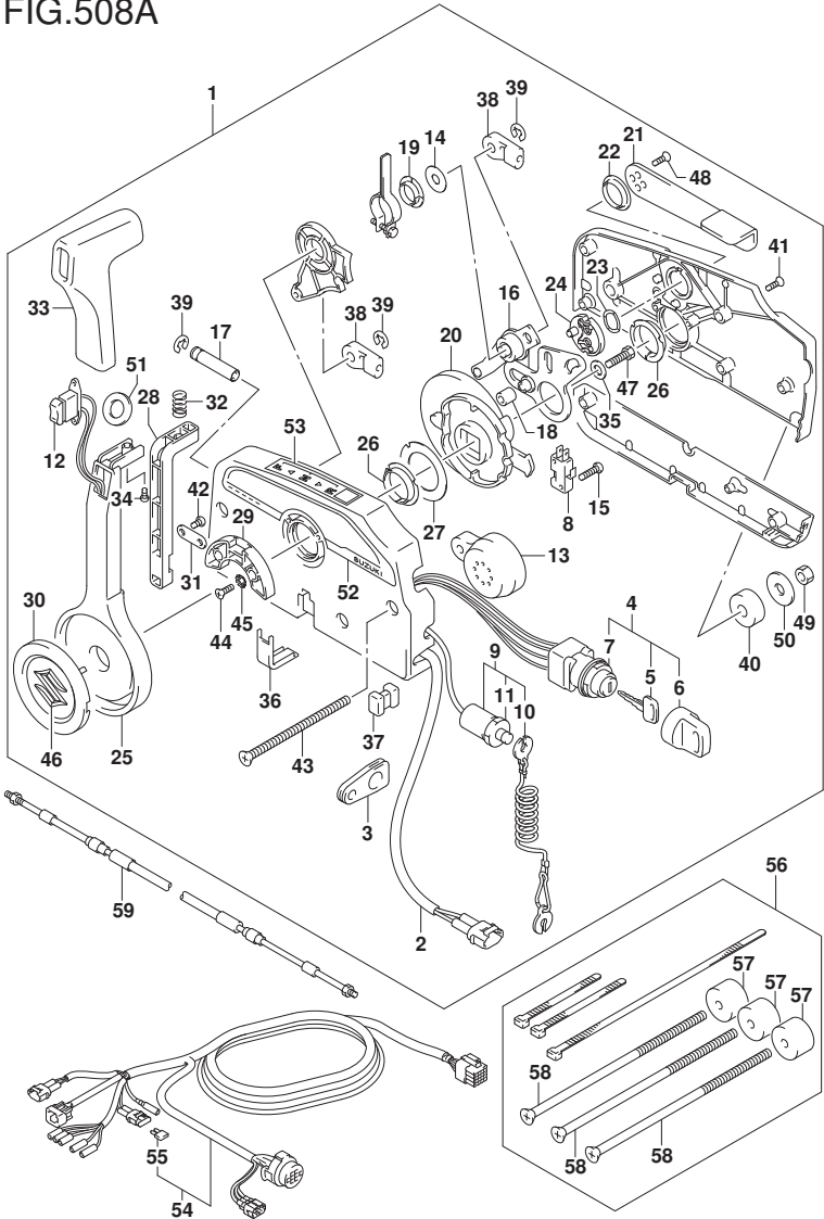
DF250_E01_019_508A OPT:REMOTE CONTROL
