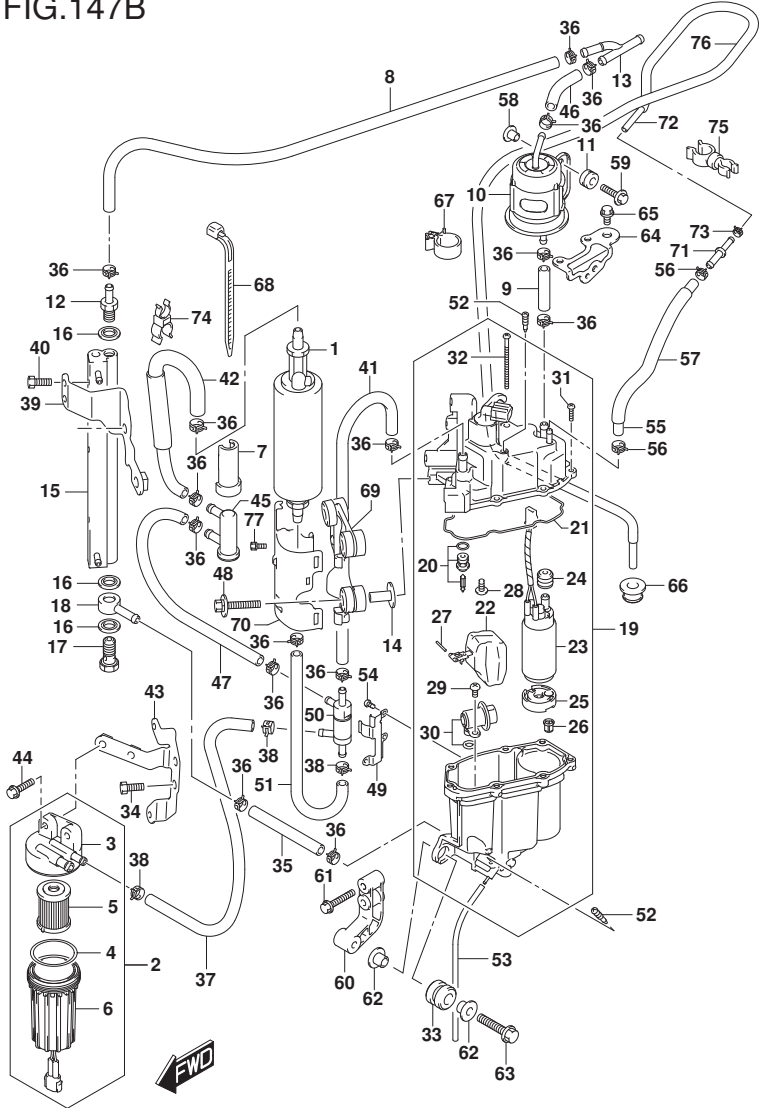
DF250_E01_019_147B FUEL PUMP/FUEL VAPOR SEPARATOR
