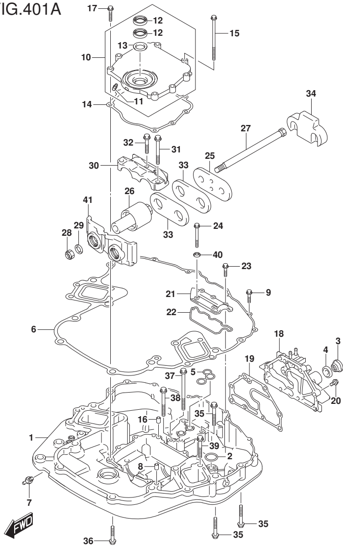
DF250_E01_019_401A ENGINE HOLDER
