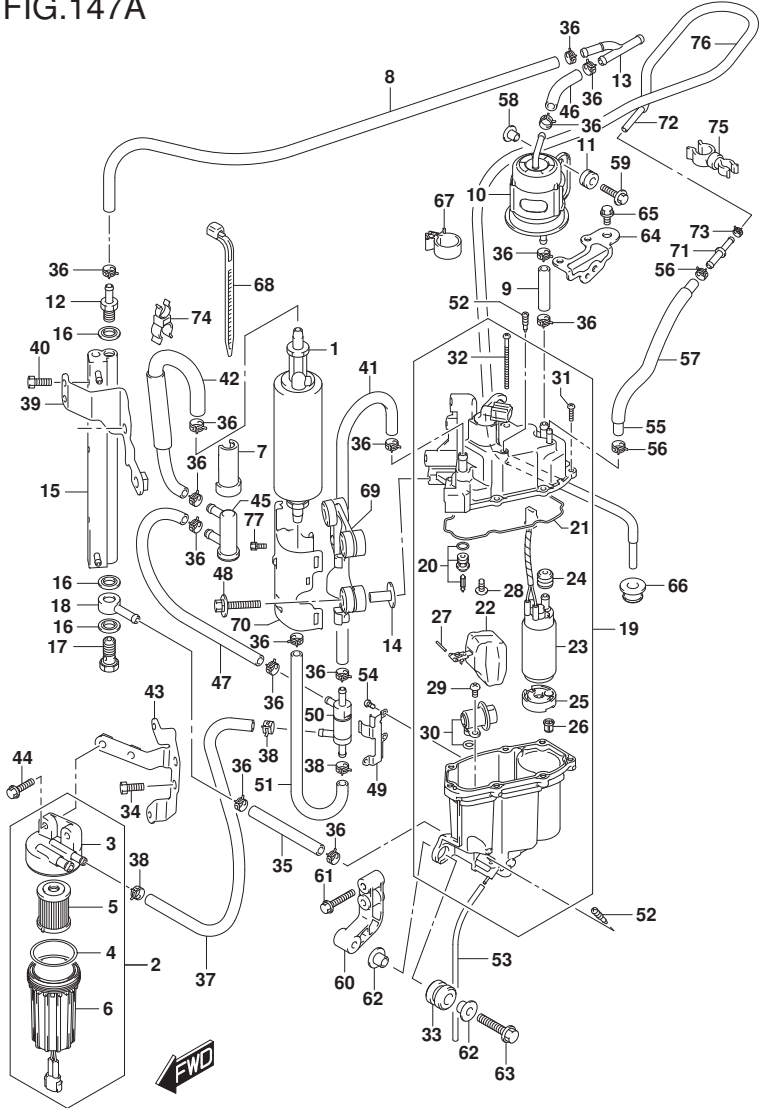
DF250_E01_019_147A FUEL PUMP/FUEL VAPOR SEPARATOR
