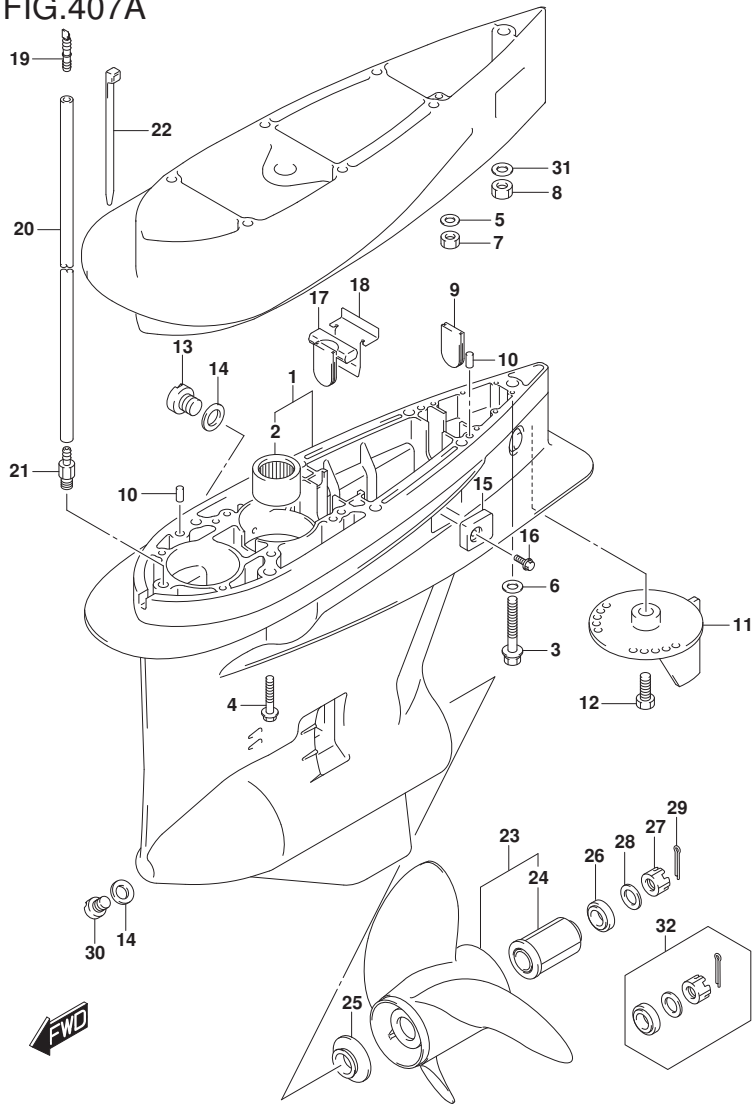
DF250_E01_019_407A GEAR CASE
