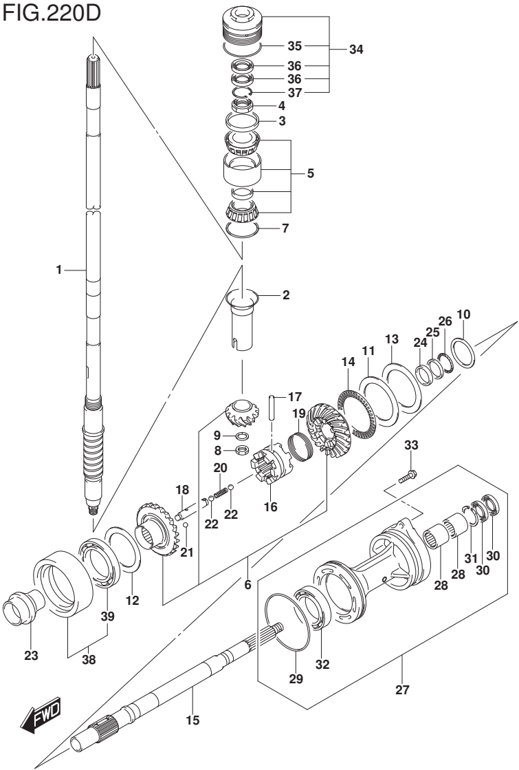
FIG.220D (1-F-13) TRANSMISSION (DF200Z E40)
