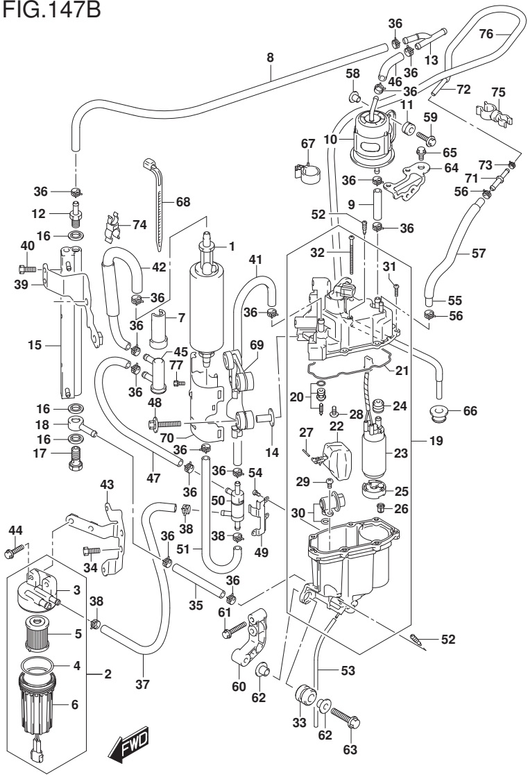
FIG.147B (1-D-2) FUEL PUMP/FUEL VAPOR SEPARATOR (E40)
