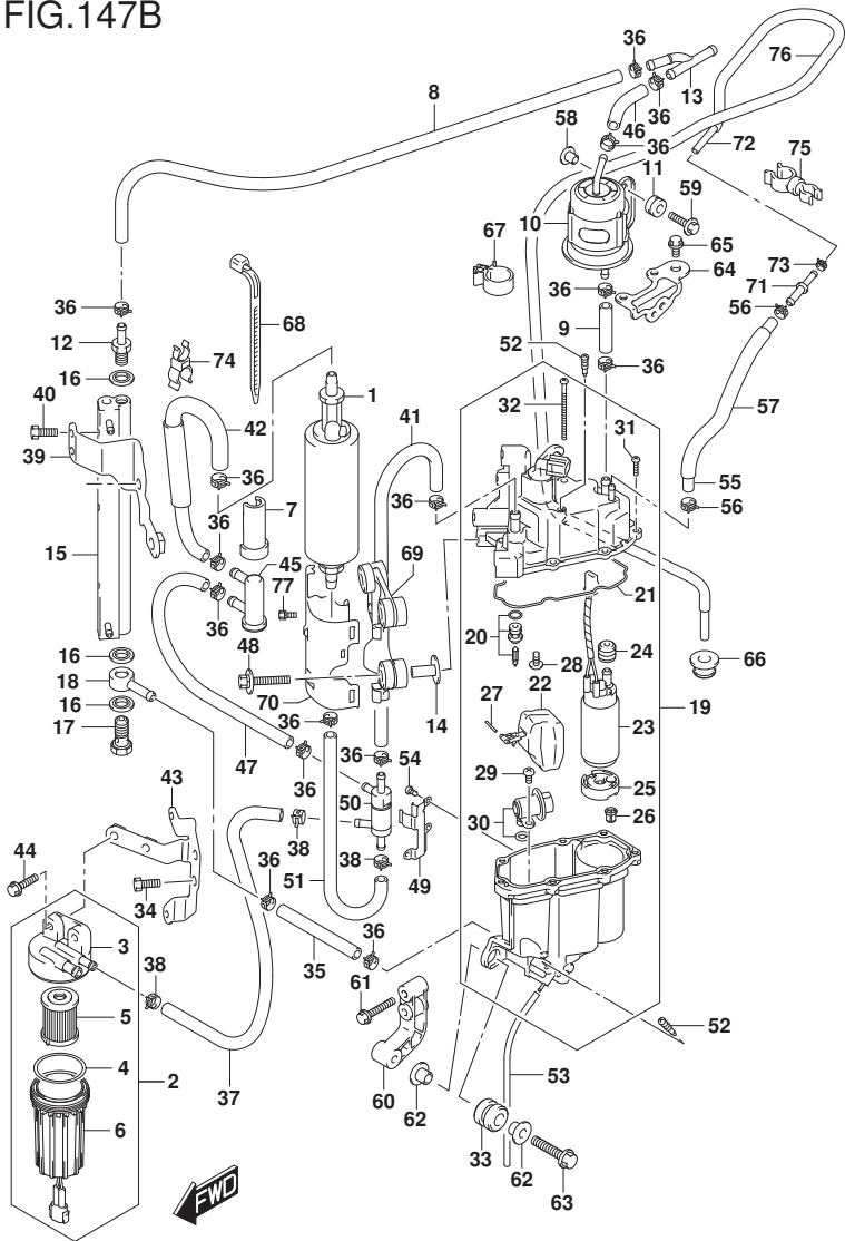
FIG.147B (1-C-15) FUEL PUMP/FUEL VAPOR SEPARATOR (E40)
