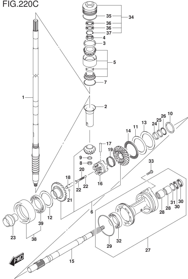
FIG.220C (1-F-8) TRANSMISSION (DF200Z E01)
