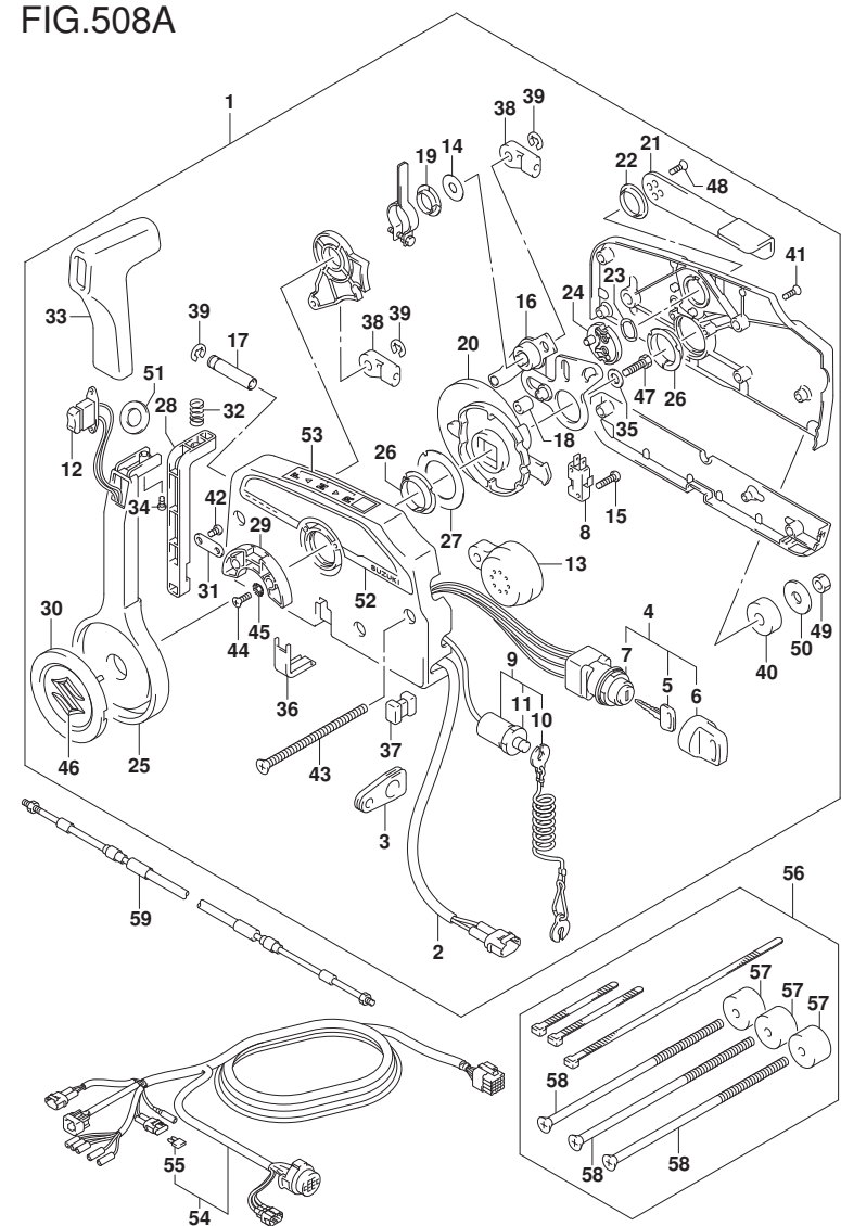
FIG.508A (1-L-8) OPT:REMOTE CONTROL
