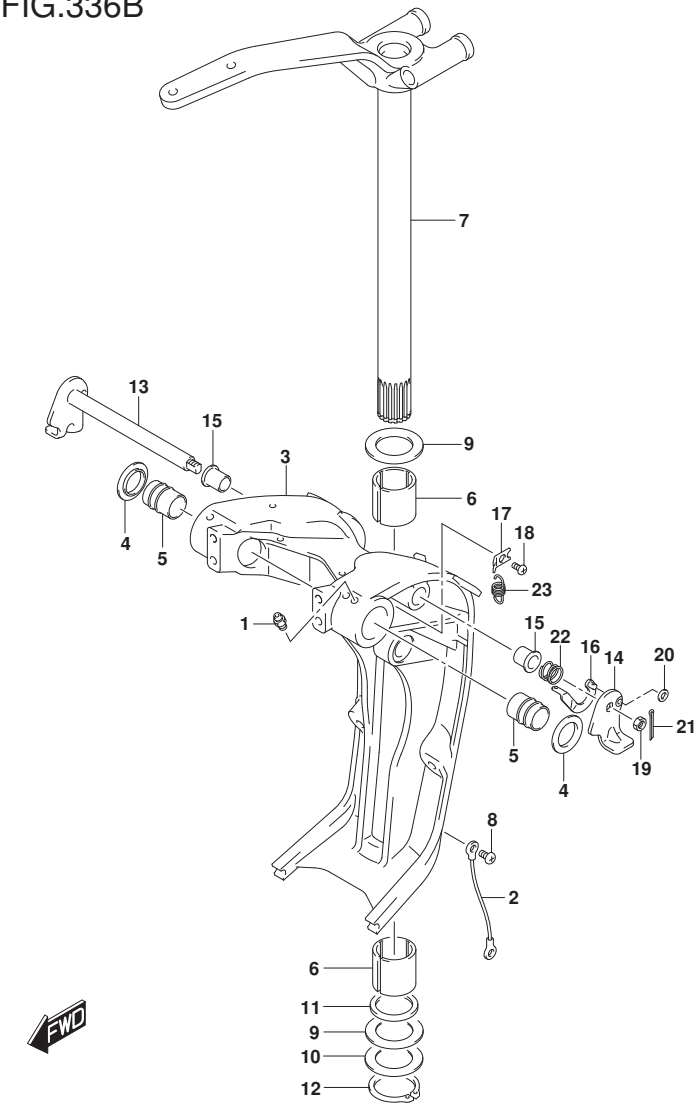
DF250_E01_019_336B SWIVEL BRACKET
