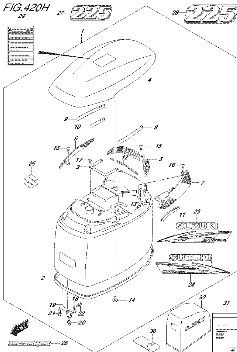
FIG.420H (3-L-4) ENGINE COVER (FOR Y5S) (DF225T E40),(DF225Z E40)
