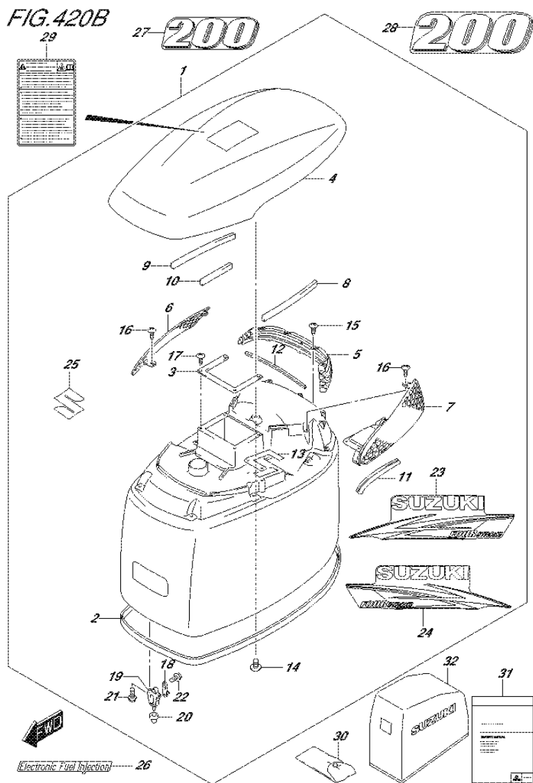
FIG.420B (3-K-6) ENGINE COVER (FOR Y5S) (DF200T E01),(DF200Z E01)
