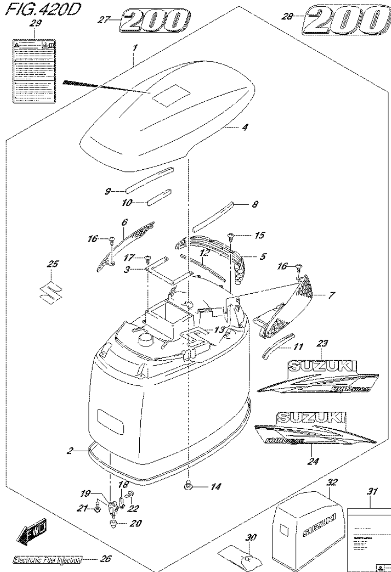
FIG.420D (3-K-9) ENGINE COVER (FOR Y5S) (DF200T E40),(DF200Z E40)
