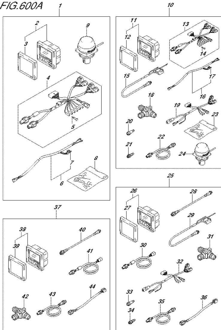
FIG.600A (4-C-8) OPT:MULTI FUNCTION GAUGE
