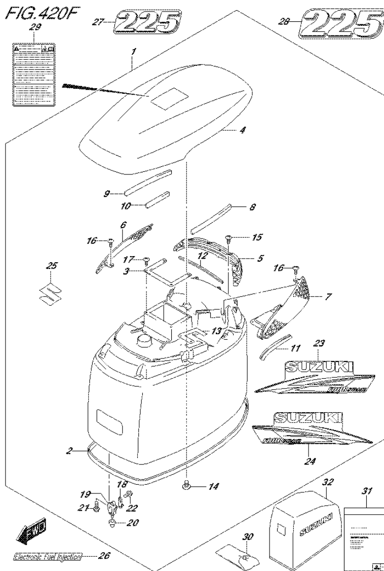
FIG.420F (3-K-14) ENGINE COVER (FOR Y5S) (DF225T E01),(DF225Z E01)
