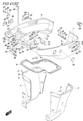
FIG. 410G DSC90 REV. 015, 410G DSE 00862
