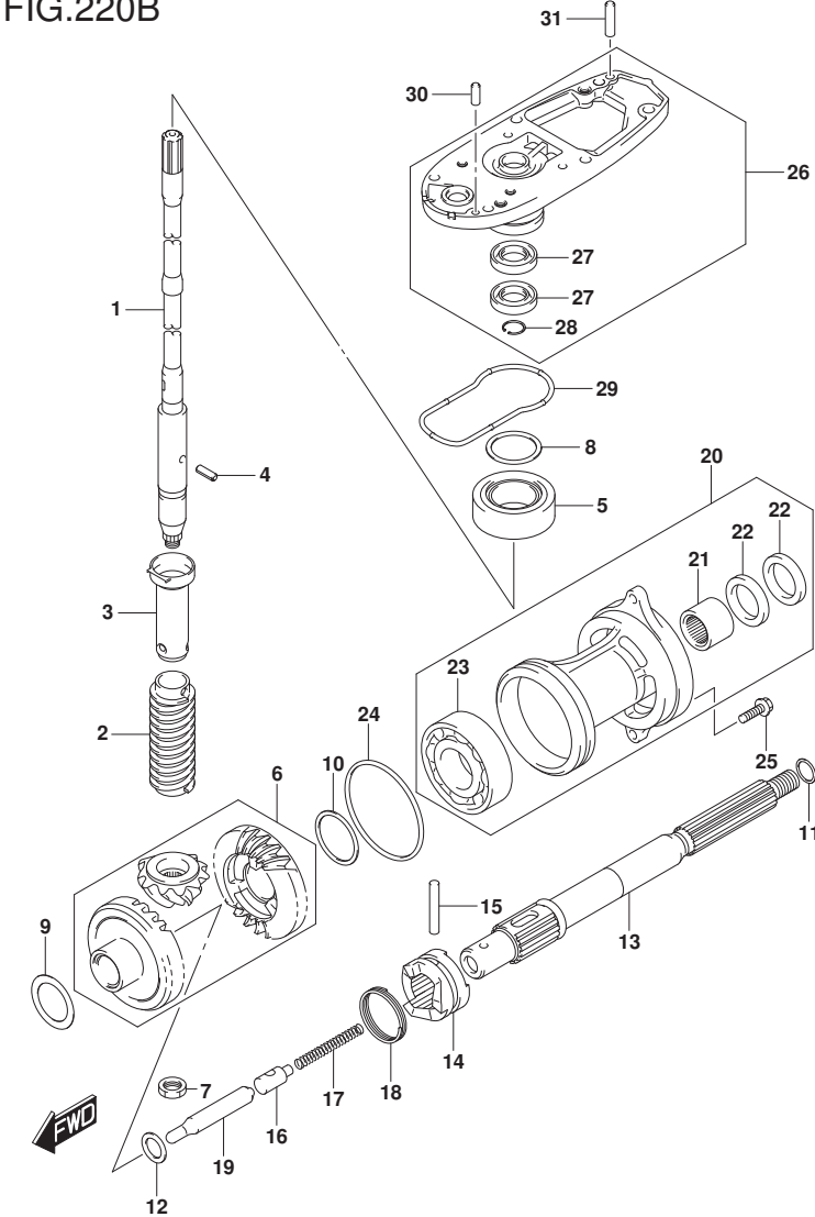
DF60A_E01_019_220B TRANSMISSION
