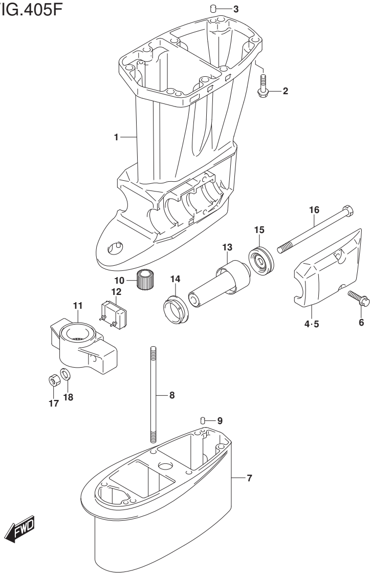
FIG.405F (1-L-3) DRIVE SHAFT HOUSING (DF60ATH E01)(DF60ATH E40)
