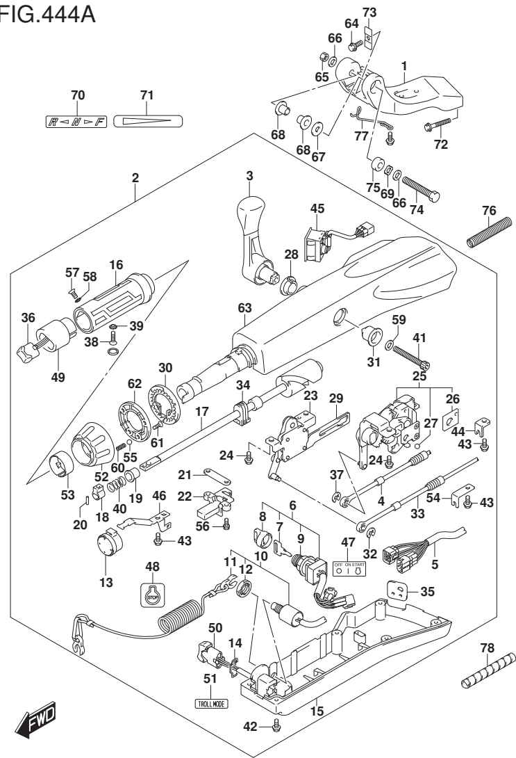
DF60A_E01_019_444A TILLER HANDLE
