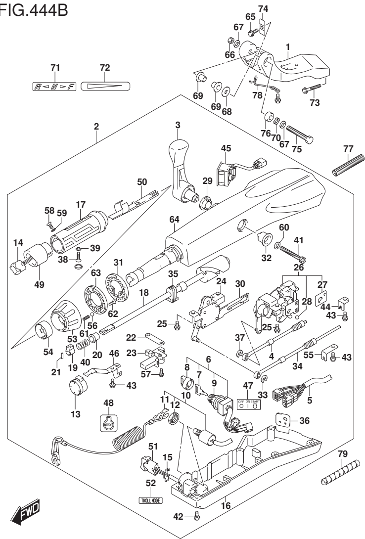
FIG.444B (2-D-6) TILLER HANDLE (DF40ATH)(DF50ATH)
