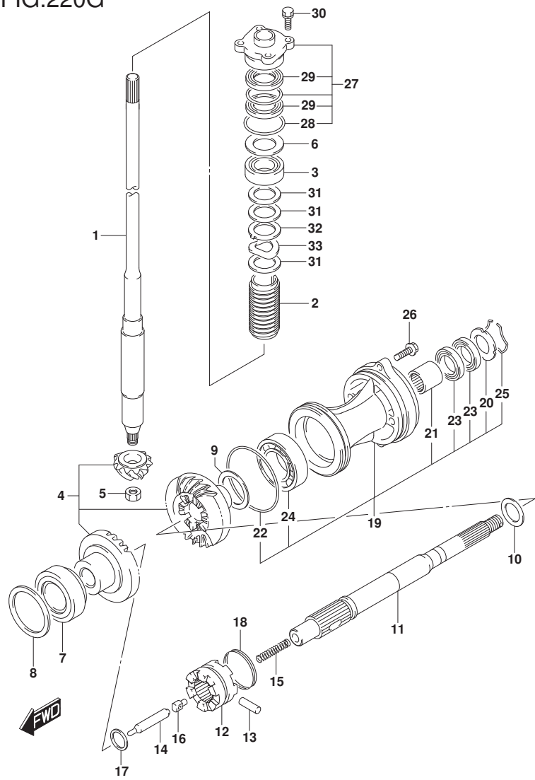
DF60A_E01_019_220G TRANSMISSION
