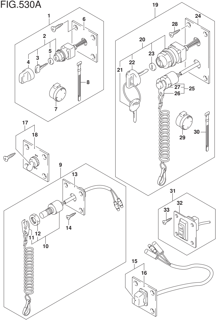
FIG.530A (2-E-15) OPT:SWITCH (DF40A)(DF40AST)(DF50A)(DF60A)(DF50AVT)(DF60AVT)
