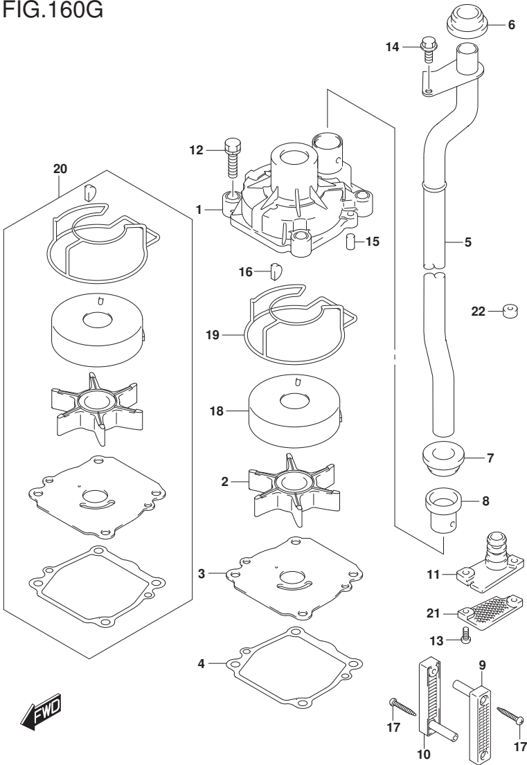
FIG.160G (1-D-7) WATER PUMP (DF60AVT E01)(DF60AVTH E01)
