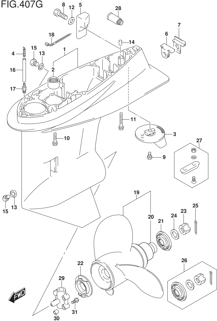
DF60A_E01_019_407G GEAR CASE
