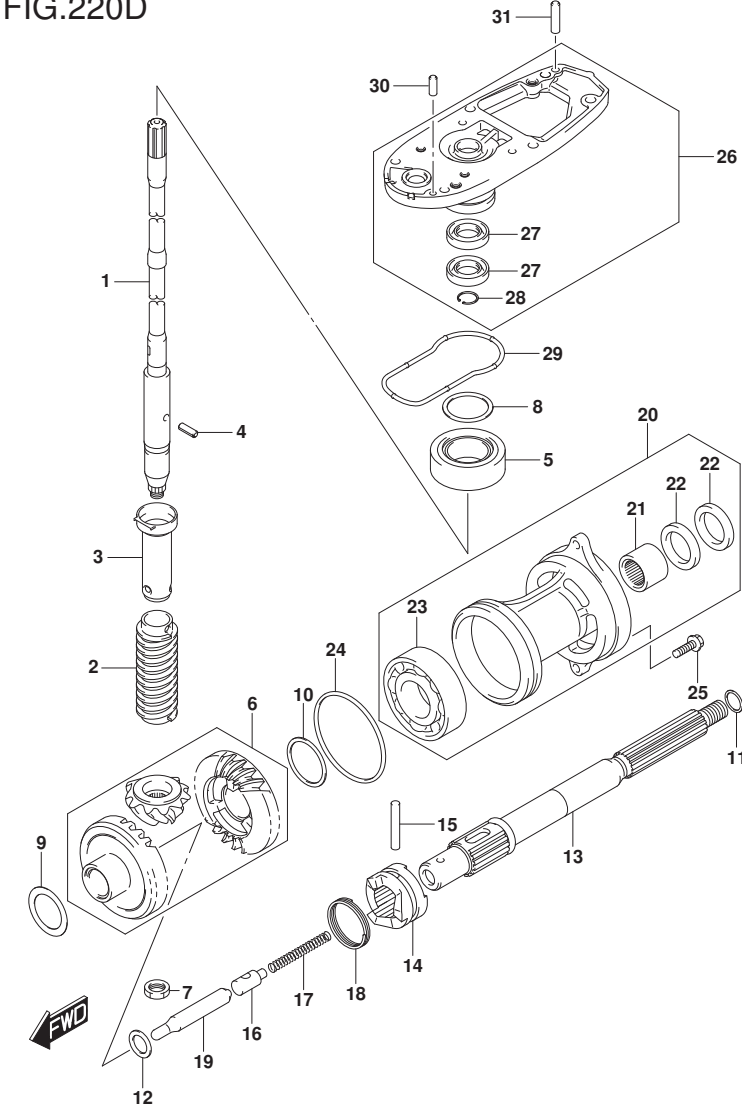
DF60A_E01_019_220D TRANSMISSION
