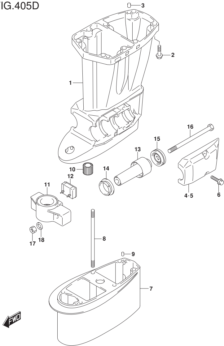
DF60A_E01_019_405D DRIVE SHAFT HOUSING
