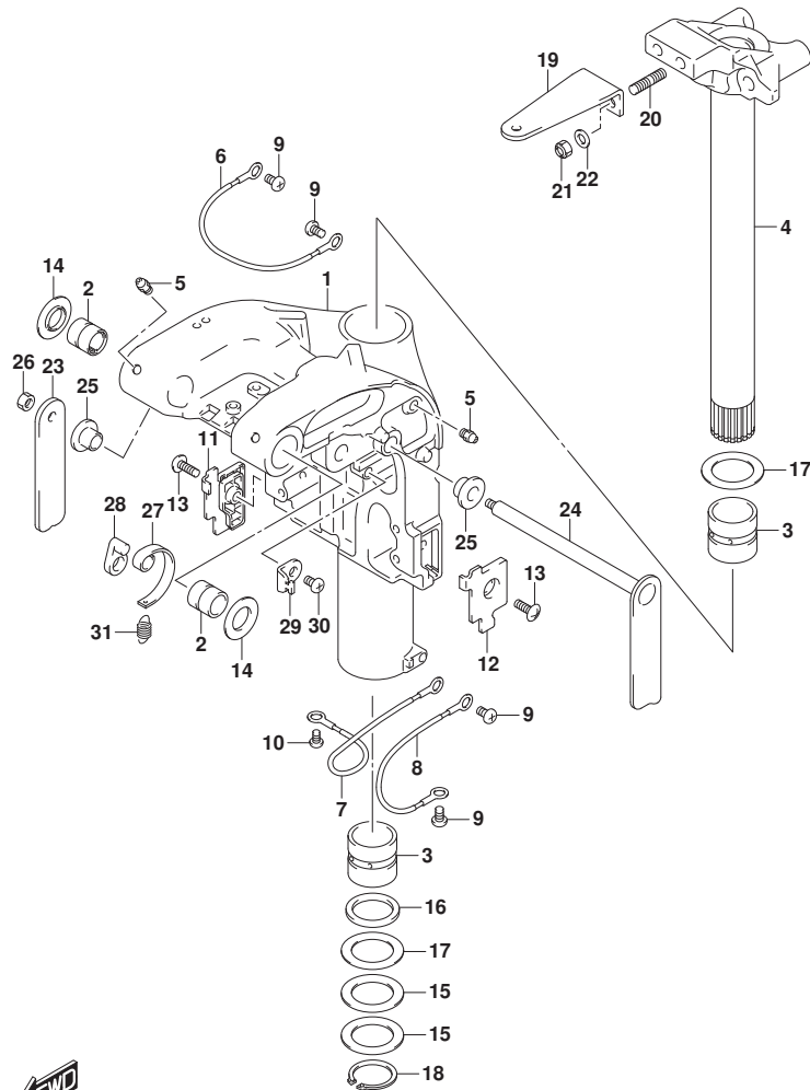
FIG.336D (1-J-4) SWIVEL BRACKET (DF60A E01)
