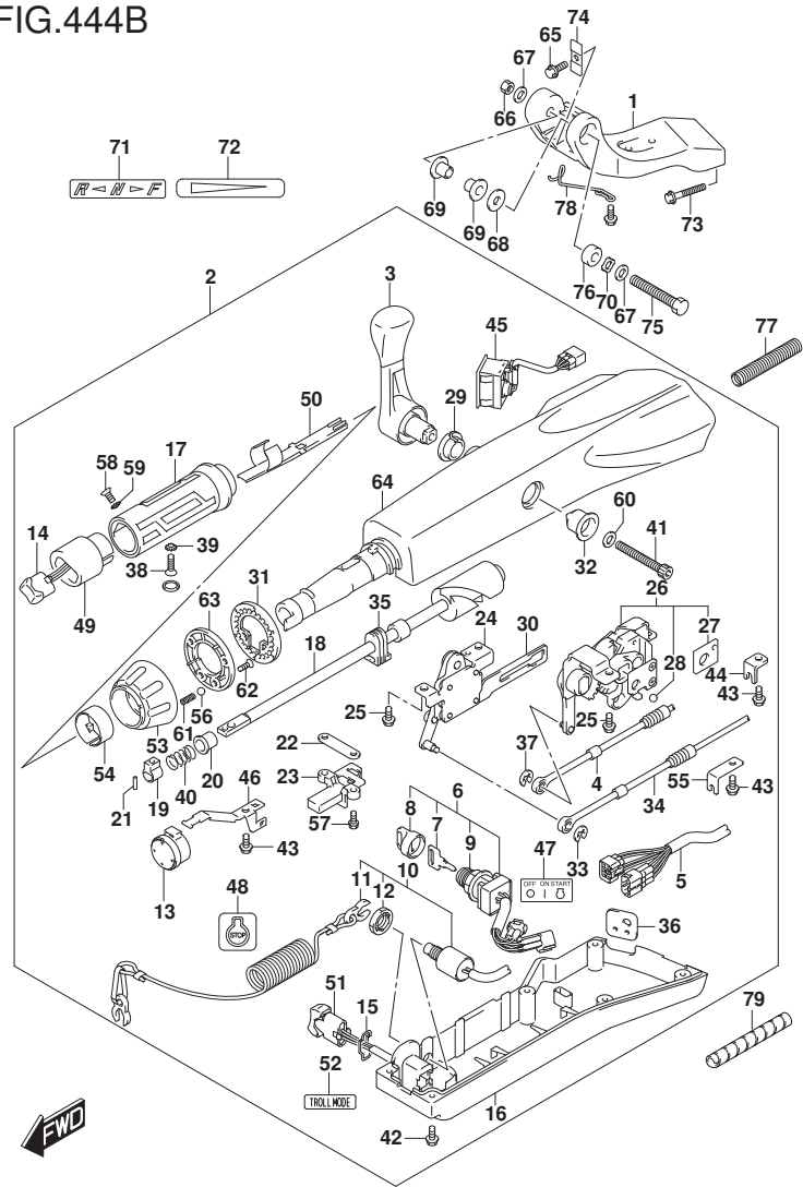
DF60A_E01_019_444B TILLER HANDLE
