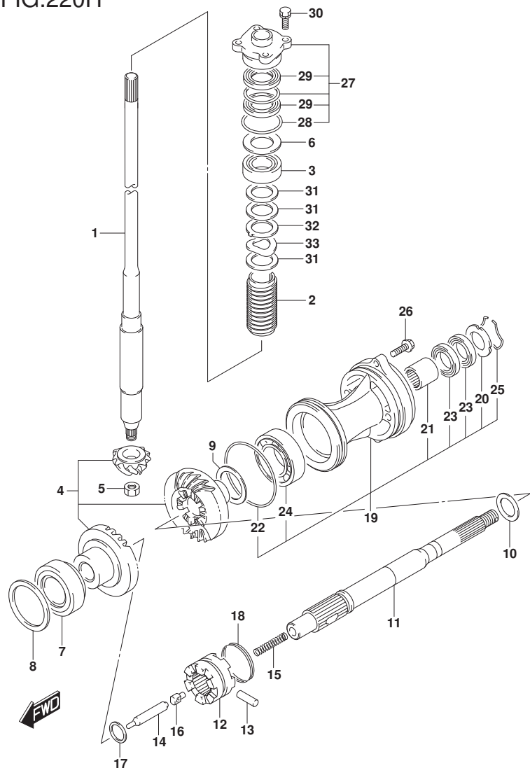
DF60A_E01_019_220H TRANSMISSION
