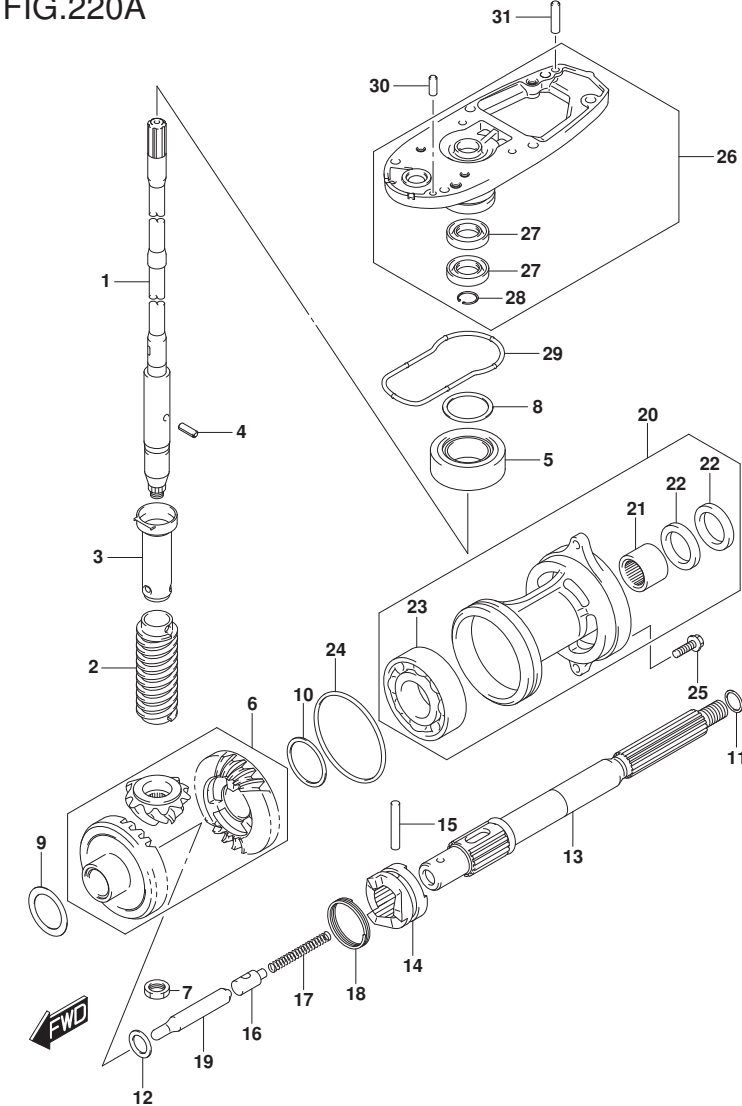
DF60A_E01_019_220A TRANSMISSION
