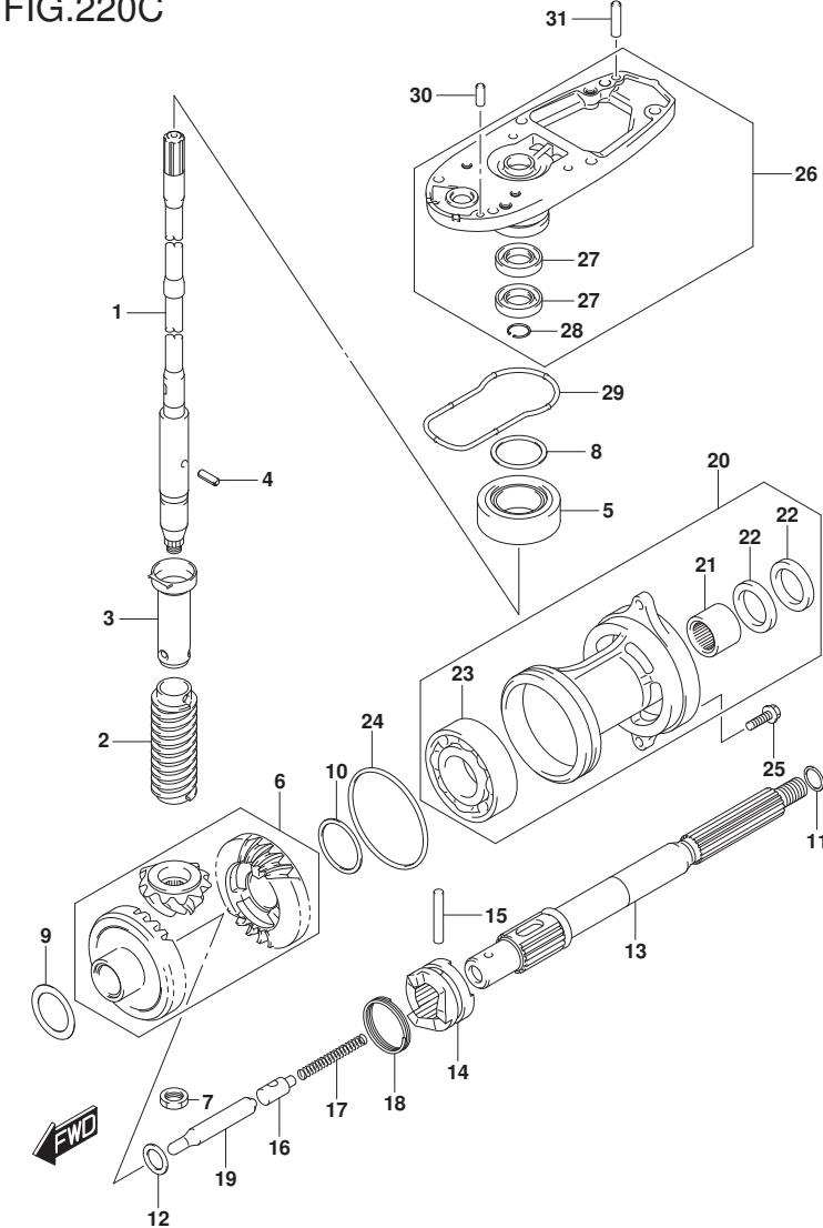
DF60A_E01_019_220C TRANSMISSION
