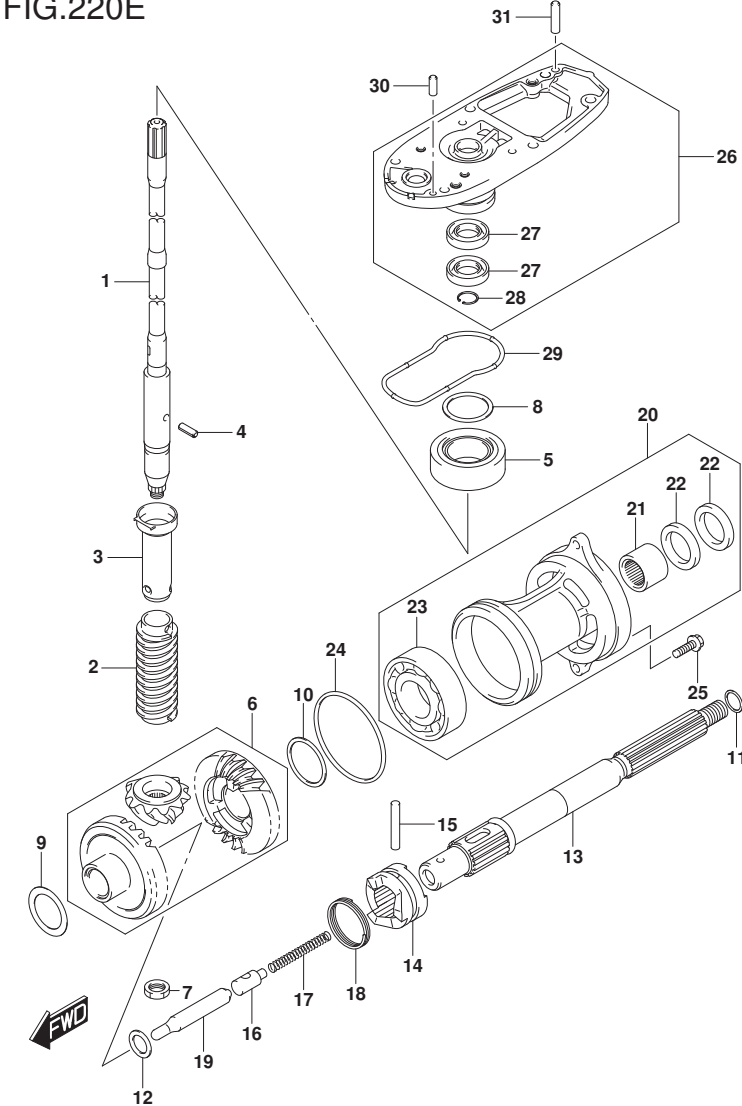
DF60A_E01_019_220E TRANSMISSION
