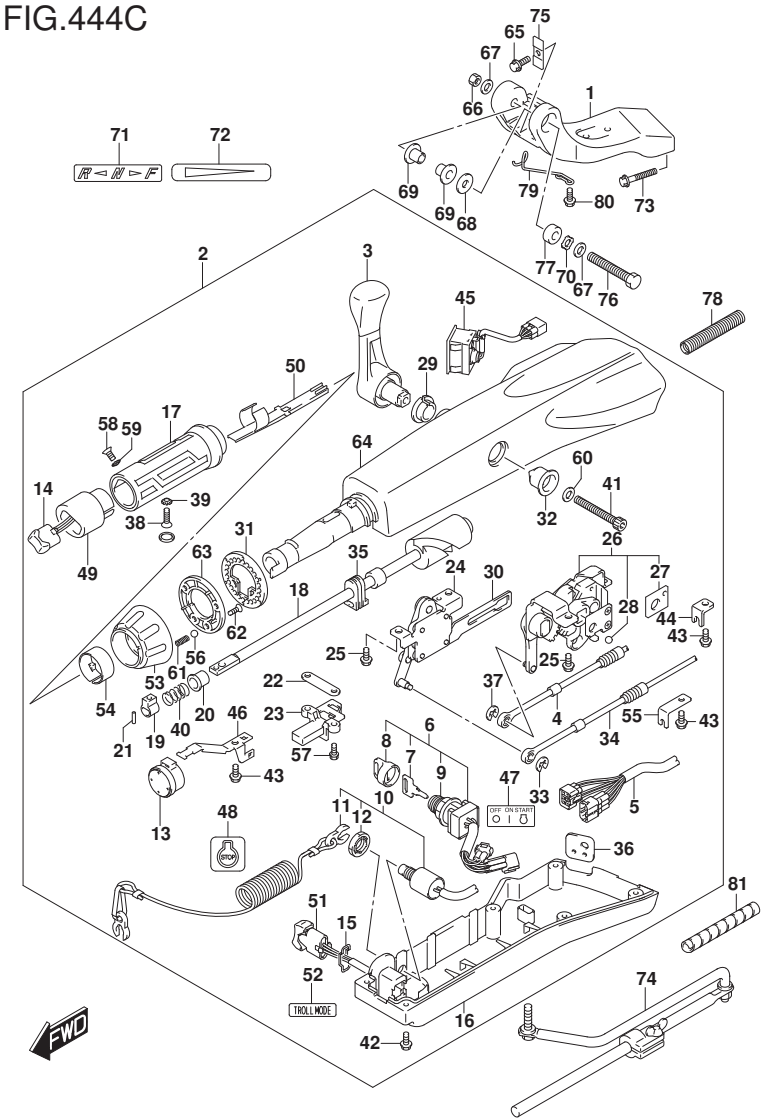
FIG.444C (2-D-10) TILLER HANDLE (DF60ATH)(DF50AVTH)(DF60AVTH)
