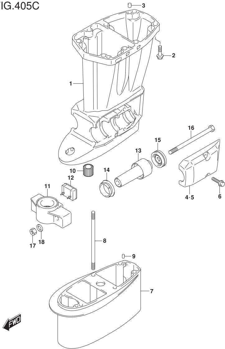
FIG.405C (1-K-14) DRIVE SHAFT HOUSING (DF60A E01)
