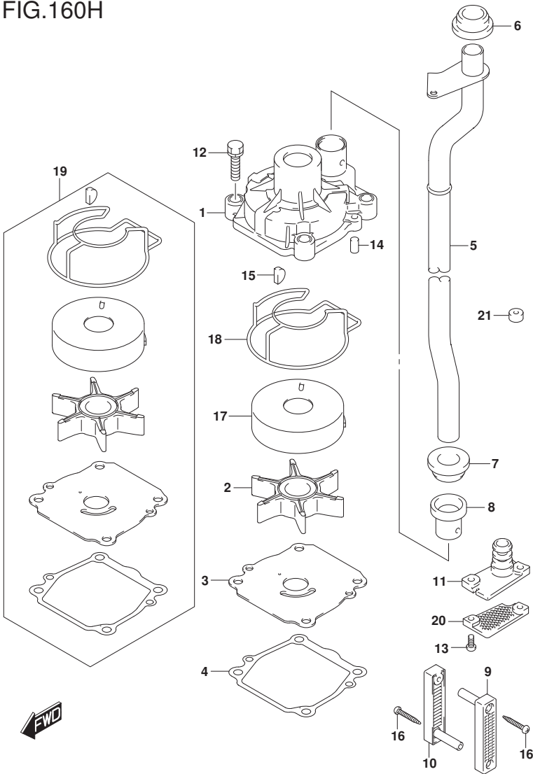
FIG.160H (1-D-8) WATER PUMP (DF60AVT E40)(DF60AVTH E40)
