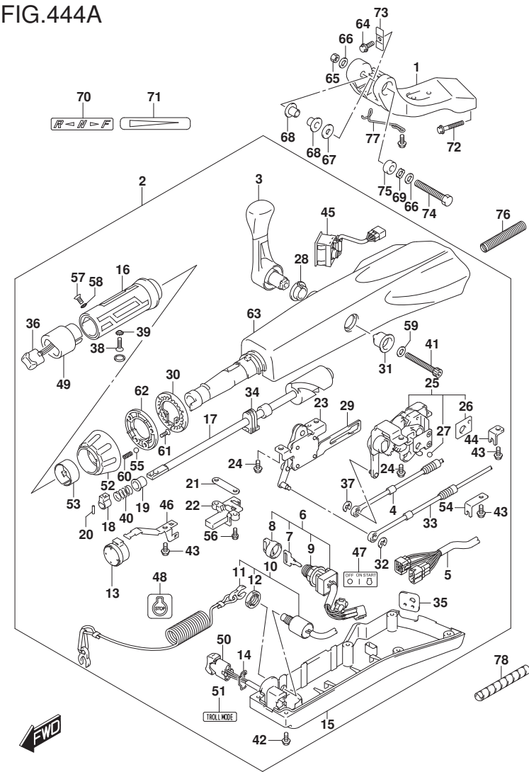
FIG.444A (2-D-2) TILLER HANDLE (DF40AQH)(DF60AQH)
