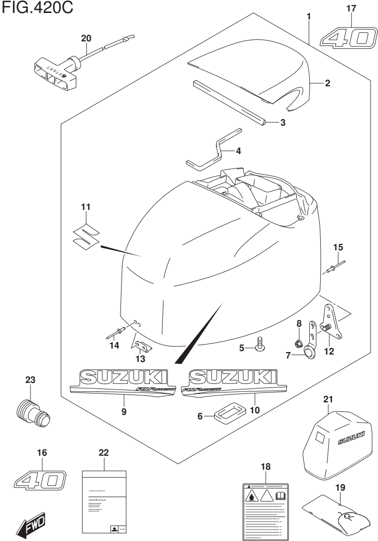
FIG.420C (2-C-4) ENGINE COVER (DF40AST E34)
