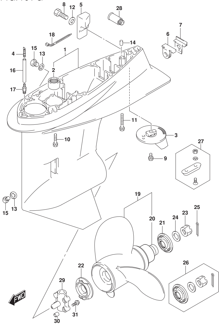
DF60A_E01_020_407G GEAR CASE
