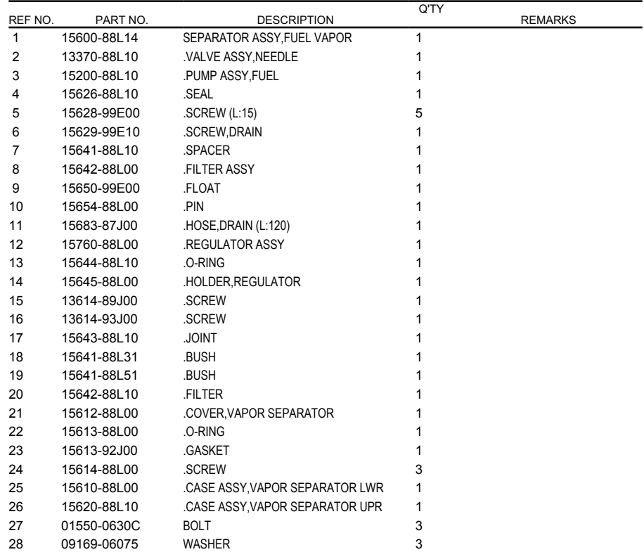
FIG.143B (1-C-10) FUEL VAPOR SEPARATOR (E40)
