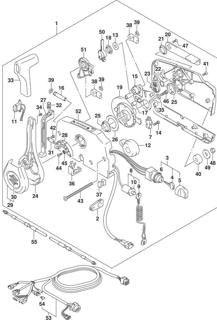
DF60A_E01_020_508A OPT:REMOTE CONTROL
