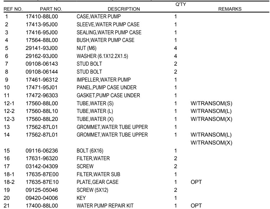
FIG.160C (1-D-3) WATER PUMP (DF60A:E01)
