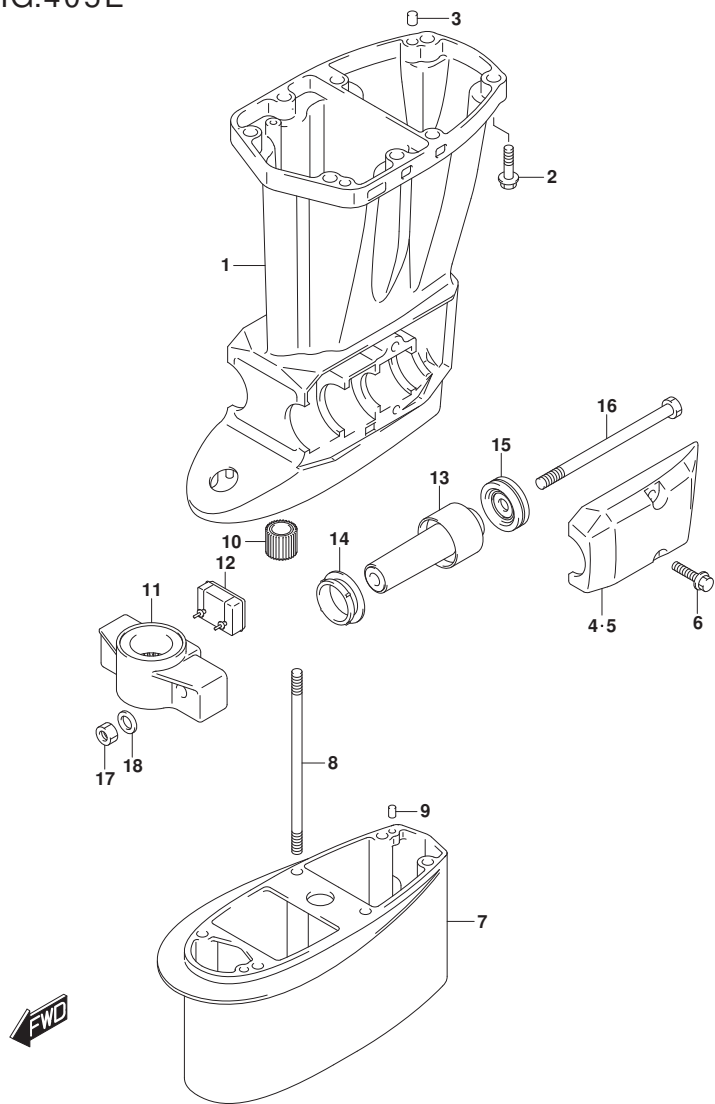
DF60A_E01_020_405E DRIVE SHAFTHOUSING
