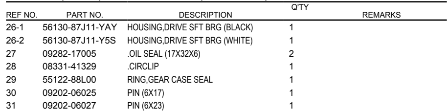
FIG.220D (1-F-13) TRANSMISSION (DF60A:E01)
