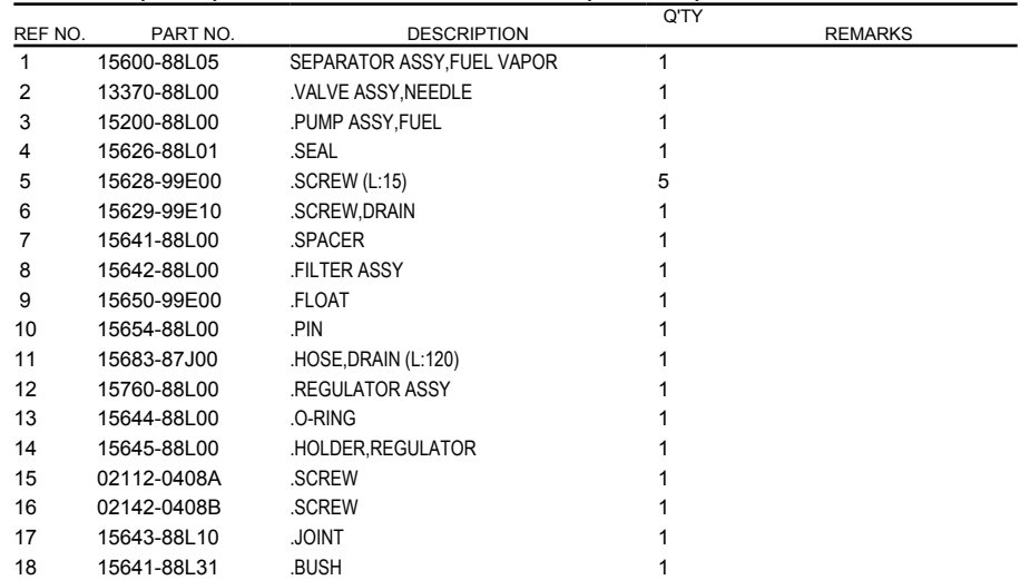
FIG.143A (1-C-7) FUEL VAPOR SEPARATOR (E01,E34)
