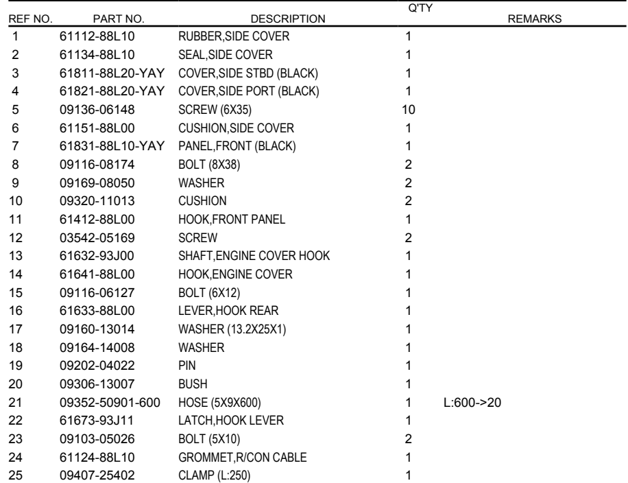
FIG.410B (1-N-8) SIDE COVER (DF40AQH:E01,DF40ATH:E01,DF50ATH:E01)
