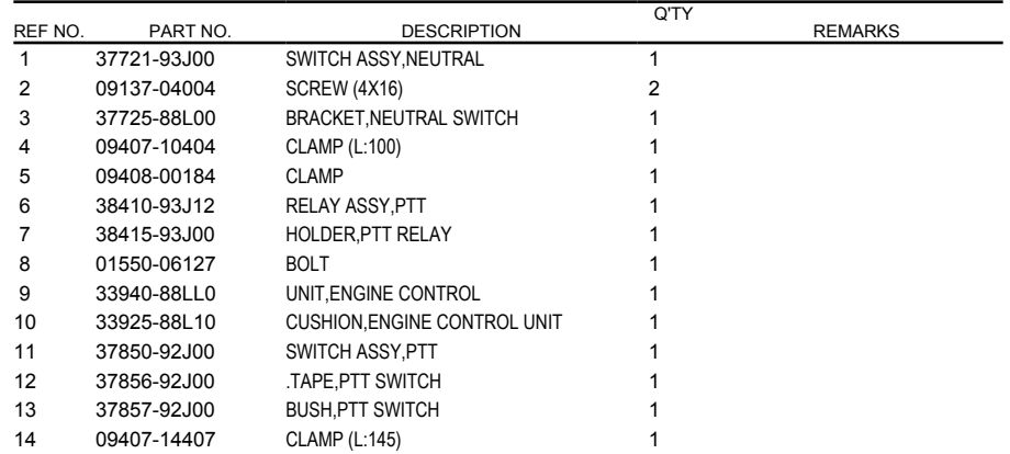
FIG.326D (1-I-5) PTT SWITCH/ENGINE CONTROL UNIT (DF50A:E01,DF50ATH:E01)
