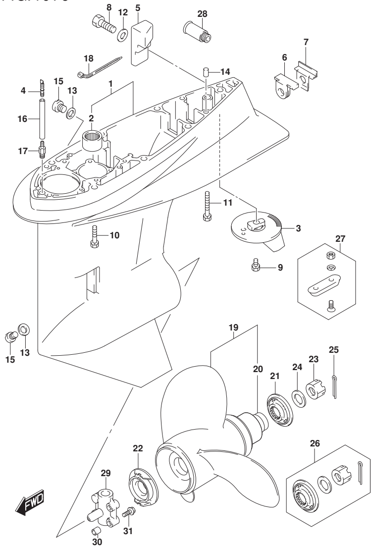
DF60A_E01_020_407J GEAR CASE
