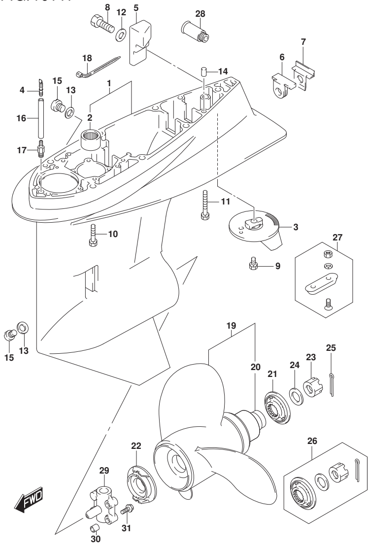
DF60A_E01_020_407H GEAR CASE
