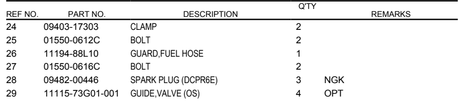
FIG.111B (1-B-5) CYLINDER HEAD (DF40AST,DF60A,DF60ATH)
