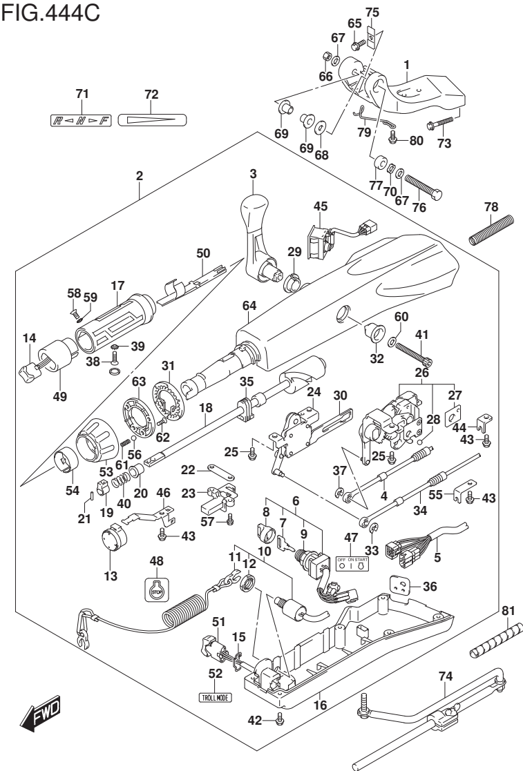
DF60A_E01_018_444C TILLER HANDLE
