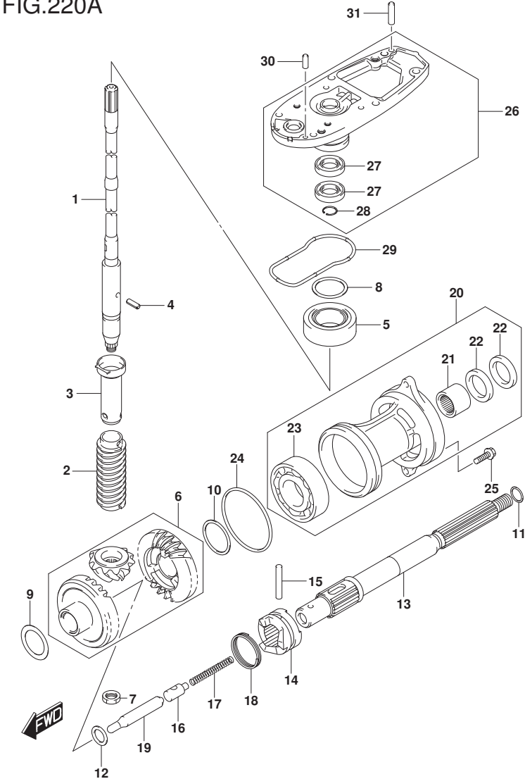
DF60A_E01_018_220A TRANSMISSION
