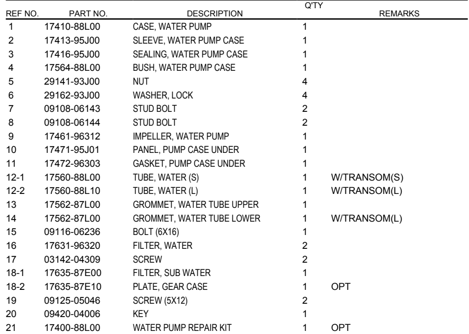
FIG.160A (1-C-14) WATER PUMP (DF40A E01)(DF40AST E34)(DF50A E01)
