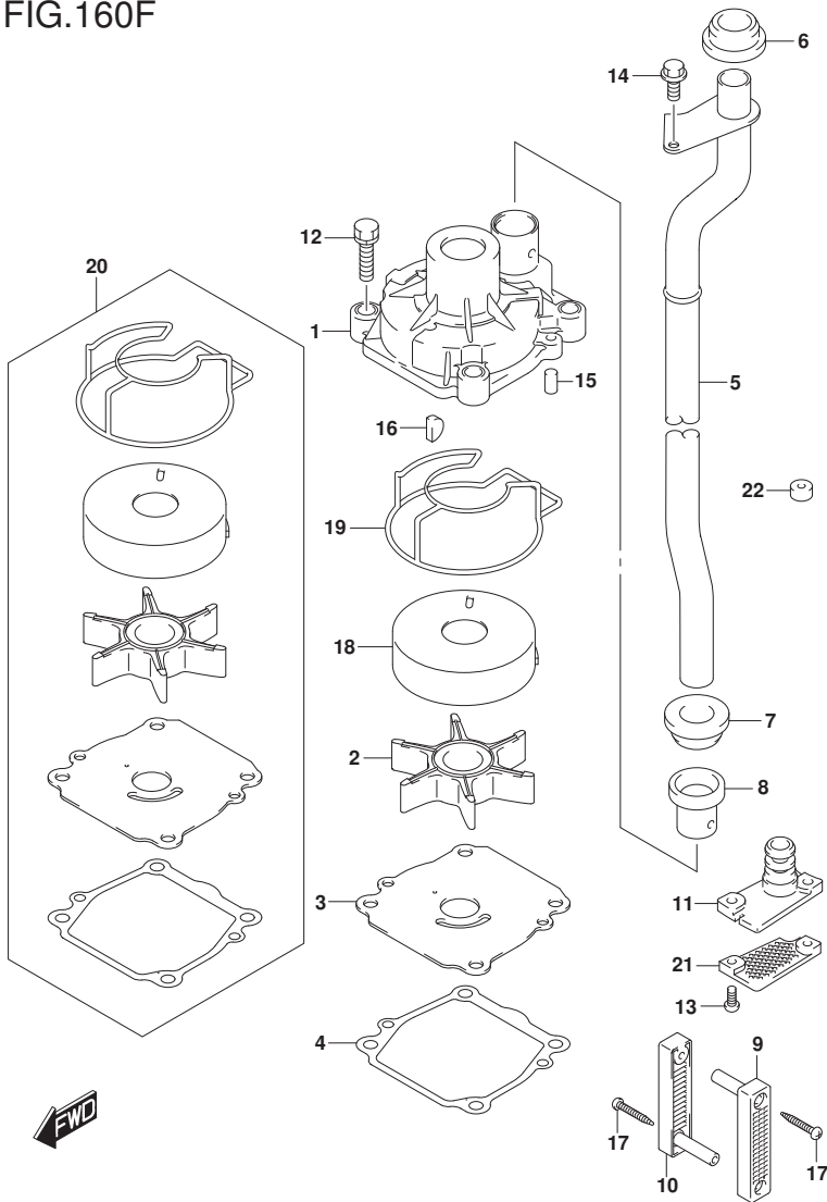
FIG.160F (1-D-5) WATER PUMP (DF50AVT E01)(DF50AVTH E01)
