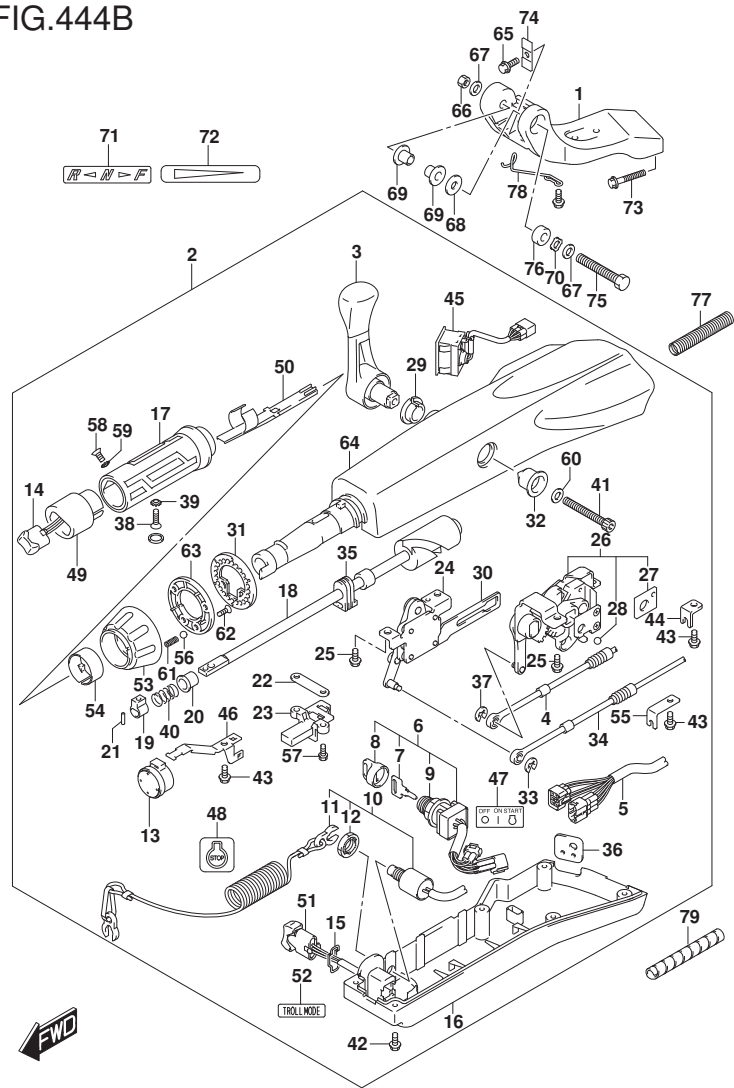
FIG.444B (2-D-6) TILLER HANDLE (DF40ATH)(DF50ATH)
