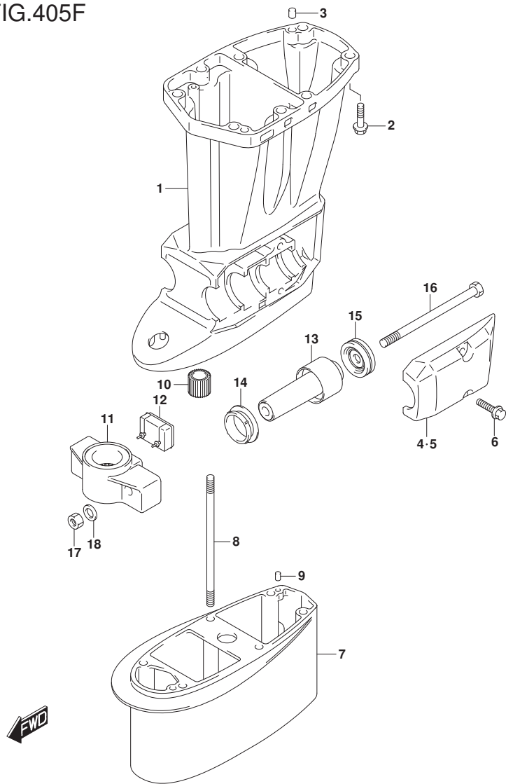
DF60A_E01_018_405F DRIVE SHAFT HOUSING
