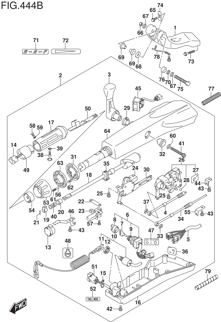
DF60A_E01_018_444B TILLER HANDLE
