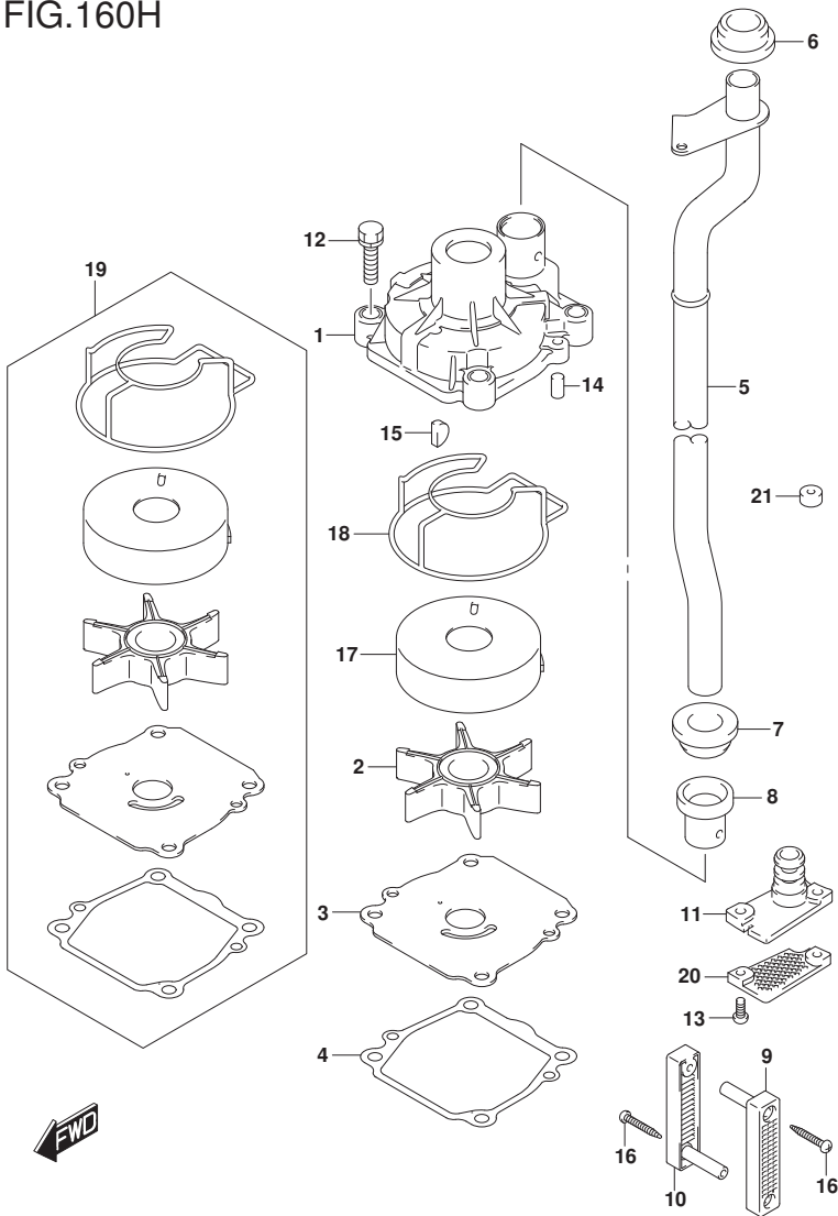
FIG.160H (1-D-7) WATER PUMP (DF60AVT E40)(DF60AVTH E40)
