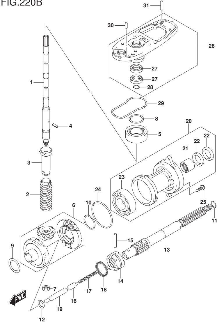
DF60A_E01_018_220B TRANSMISSION
