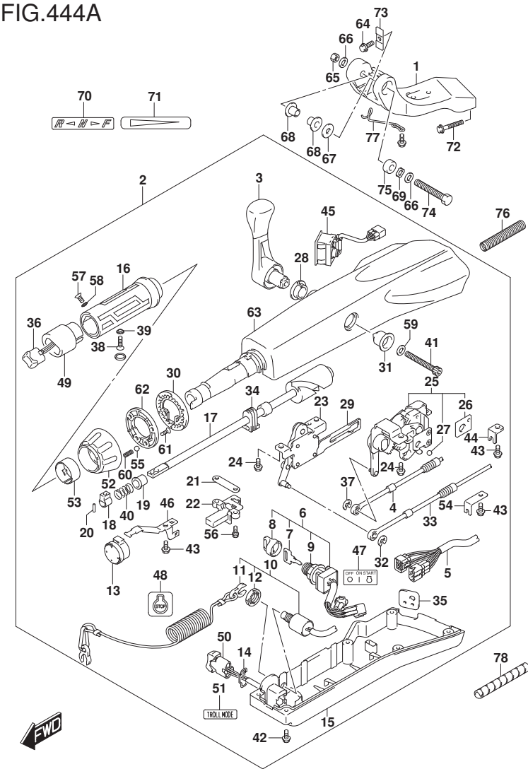
FIG.444A (2-D-4) TILLER HANDLE (DF40AQH)(DF60AQH)
