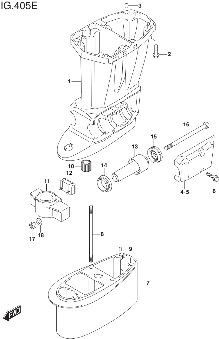
FIG.405E (1-L-4) DRIVE SHAFT HOUSING (DF60ATH E01)(DF60ATH E40)
