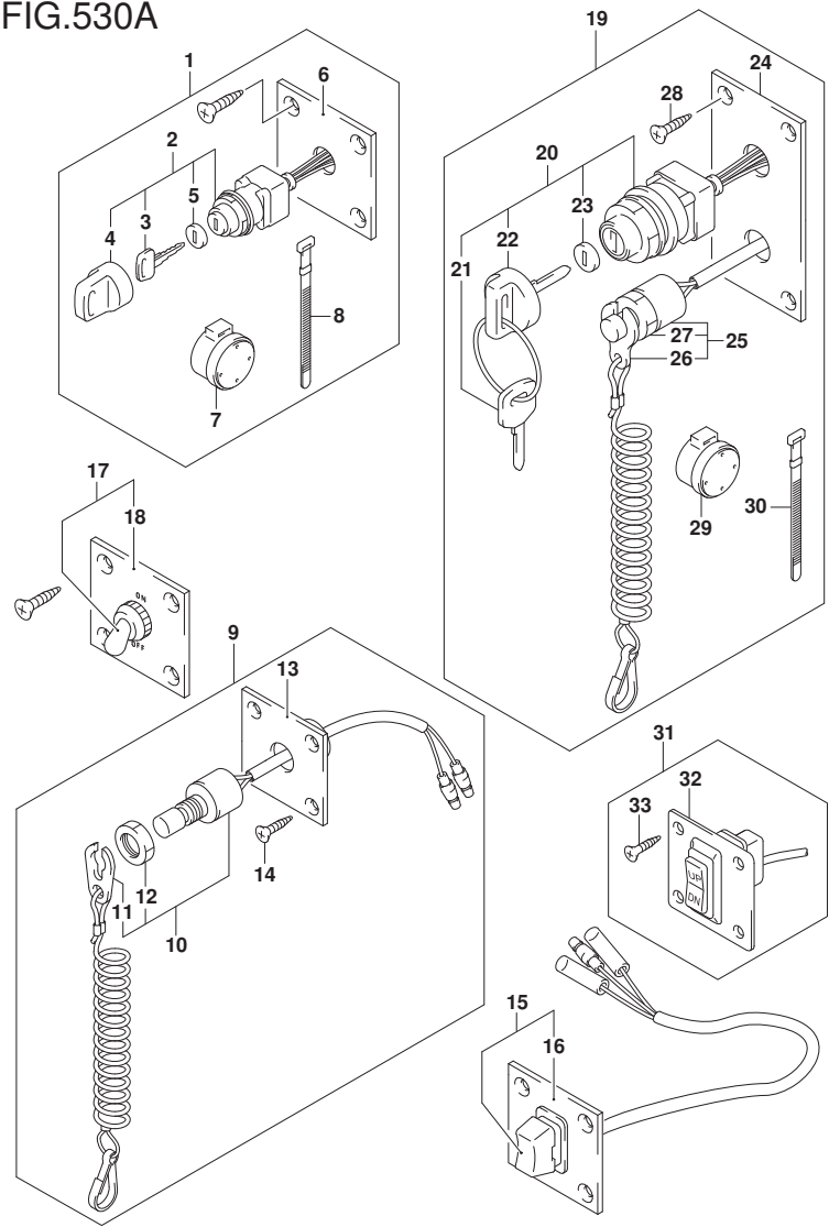
FIG.530A (2-F-3) OPT:SWITCH (DF40A)(DF40AST)(DF50A)(DF60A)(DF50AVT)(DF60AVT)
