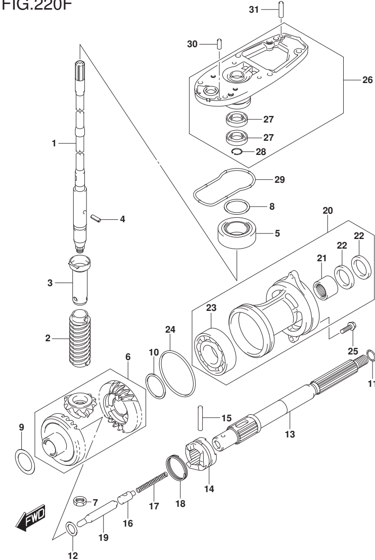
DF60A_E01_018_220F TRANSMISSION
