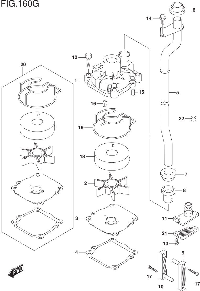
FIG.160G (1-D-6) WATER PUMP (DF60AVT E01)(DF60AVTH E01)
