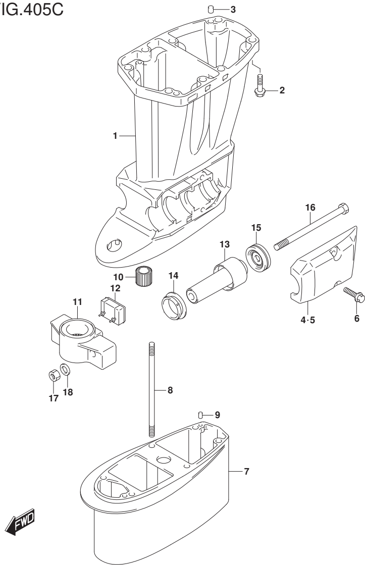
FIG.405C (1-K-15) DRIVE SHAFT HOUSING (DF60A E01)
