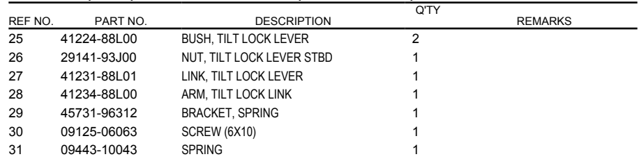
FIG.336D (1-J-7) SWIVEL BRACKET (DF40AST E34)
