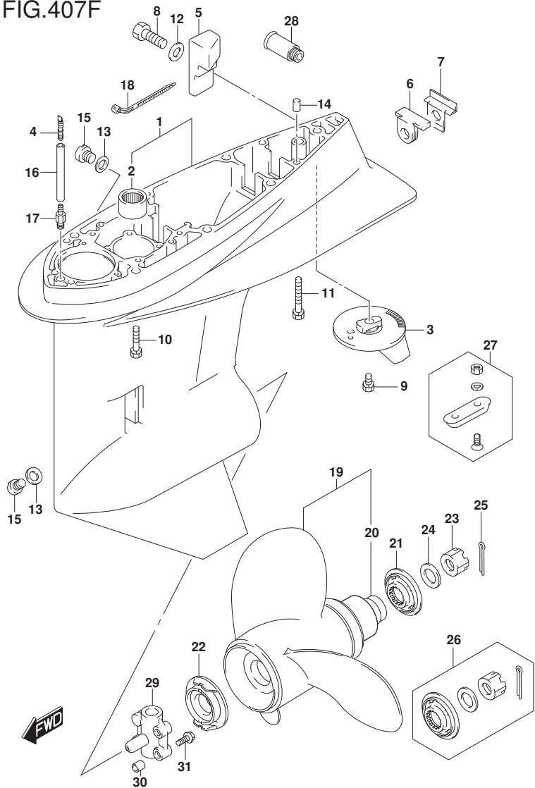
DF60A_E01_018_407F GEAR CASE
