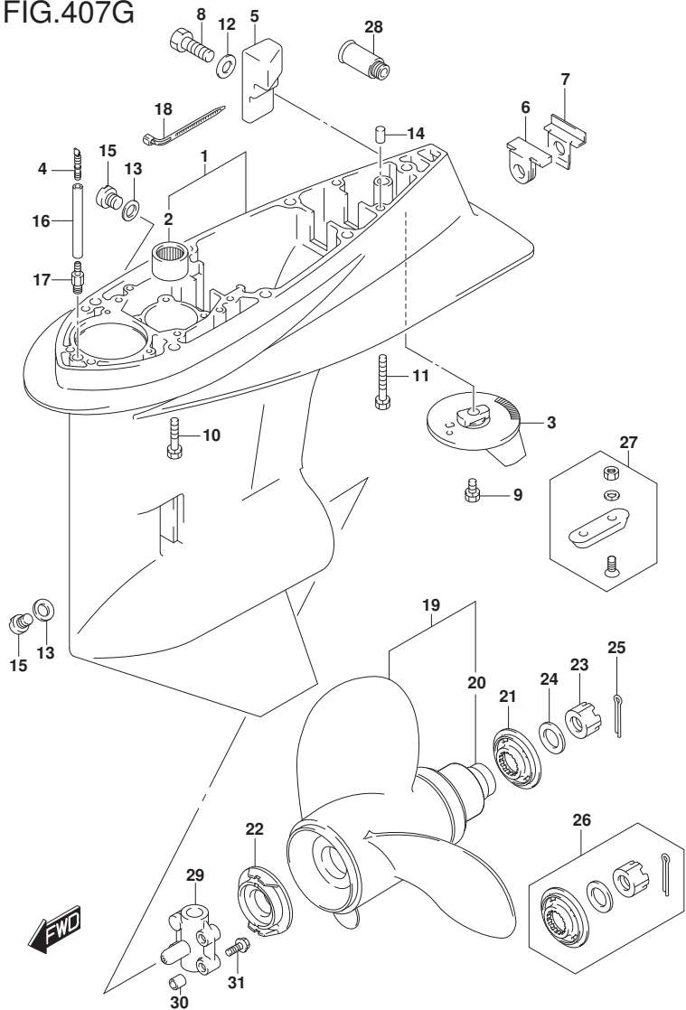
DF60A_E01_018_407G GEAR CASE
