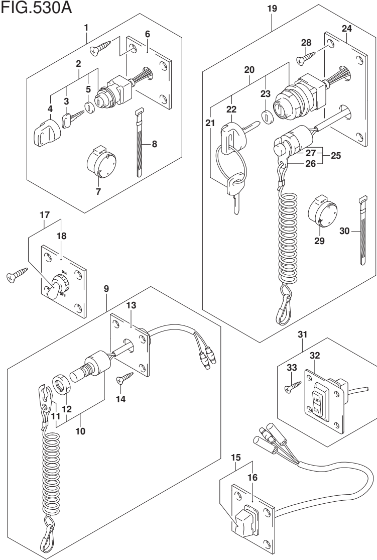
FIG.530A (2-F-2) OPT:SWITCH (DF40A)(DF40AST)(DF50A)(DF60A)(DF50AVT)(DF60AVT)
