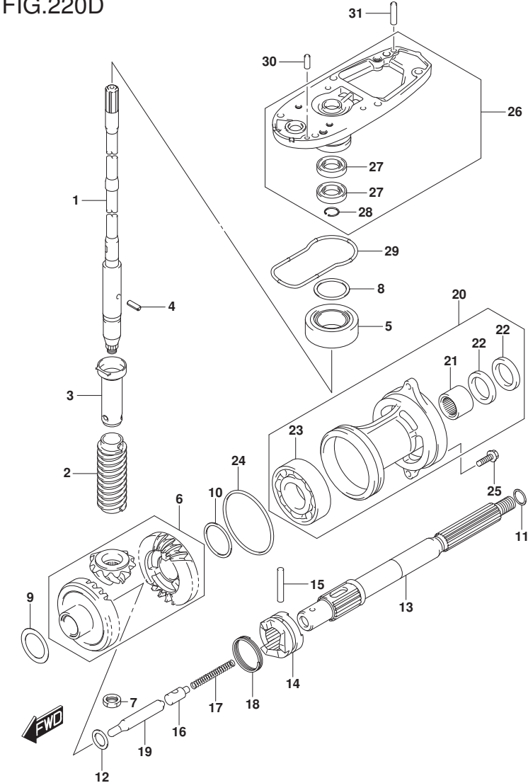
DF60A_E01_018_220D TRANSMISSION
