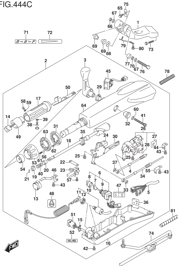
FIG.444C (2-D-11) TILLER HANDLE (DF60ATH)(DF50AVTH)(DF60AVTH)
