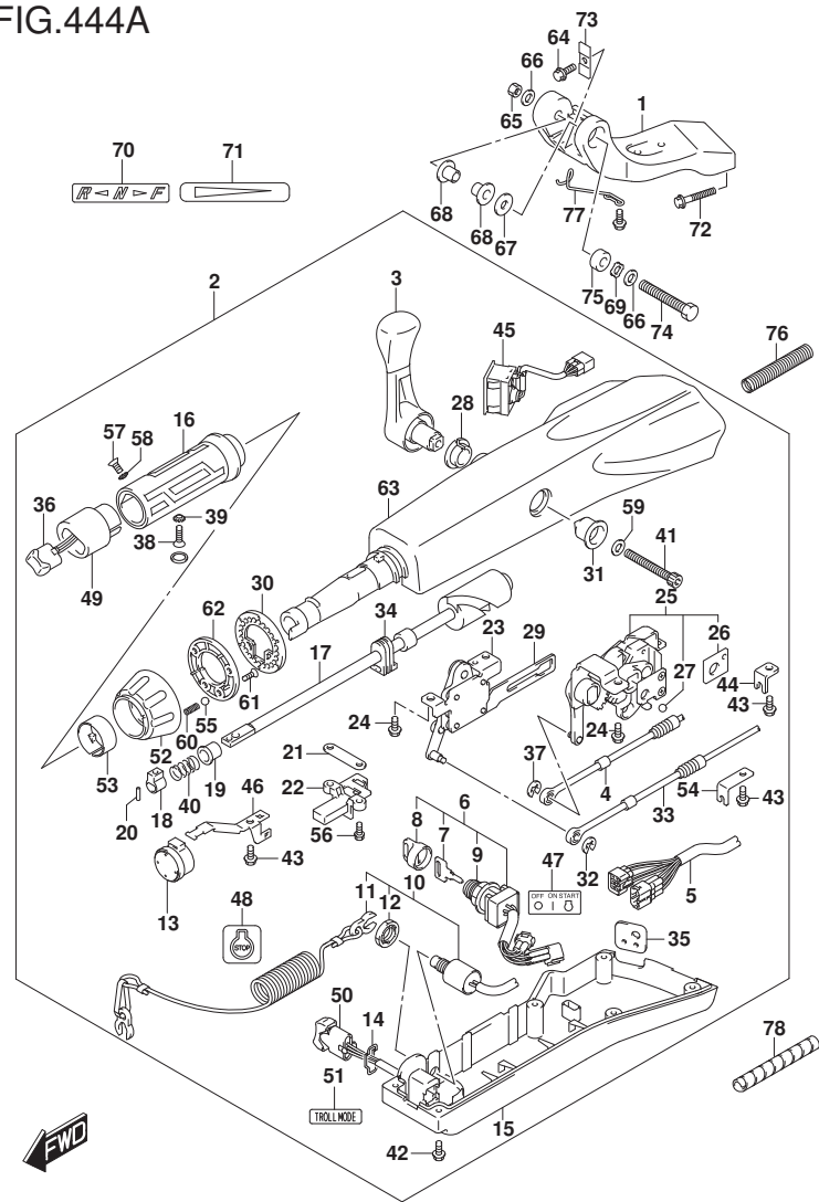
FIG.444A (2-C-15) TILLER HANDLE (DF40AQH)(DF60AQH)
