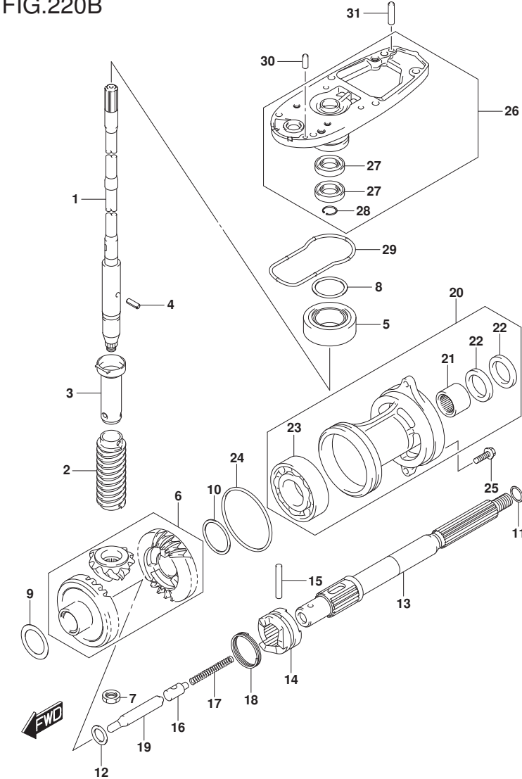
DF60A_E01_018_220B TRANSMISSION
