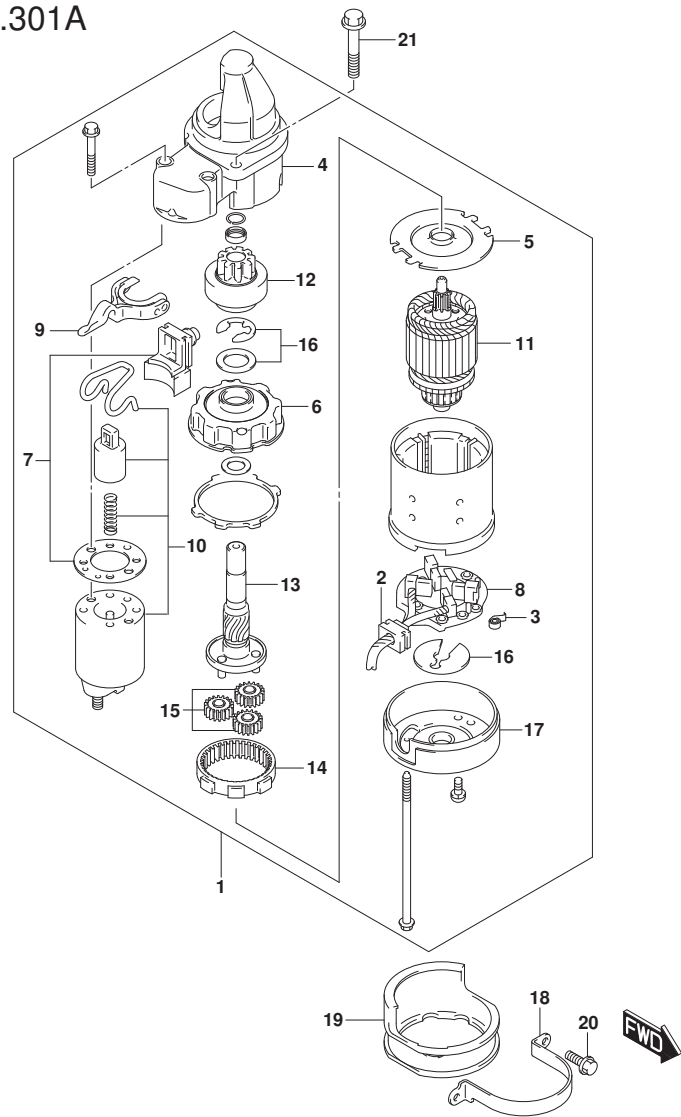
FIG.301A (1-G-12) STARTING MOTOR
