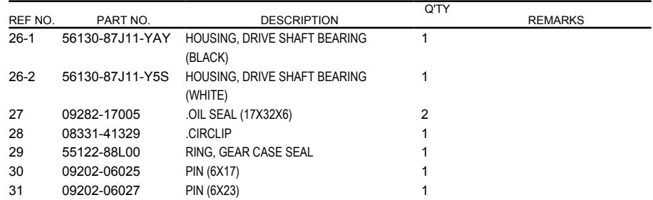
FIG.220A (1-F-7) TRANSMISSION (DF40A E01)(DF50A E01)
