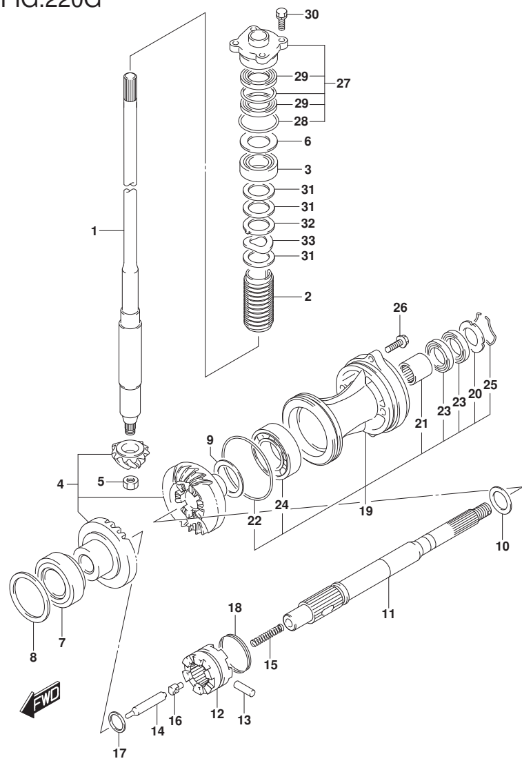
DF60A_E01_018_220G TRANSMISSION
