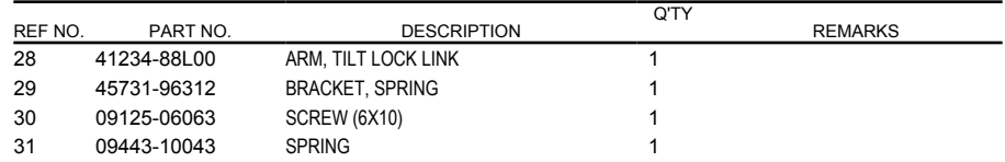
FIG.336K (1-K-2) SWIVEL BRACKET (DF60AVT E01)(DF60AVT E40)
