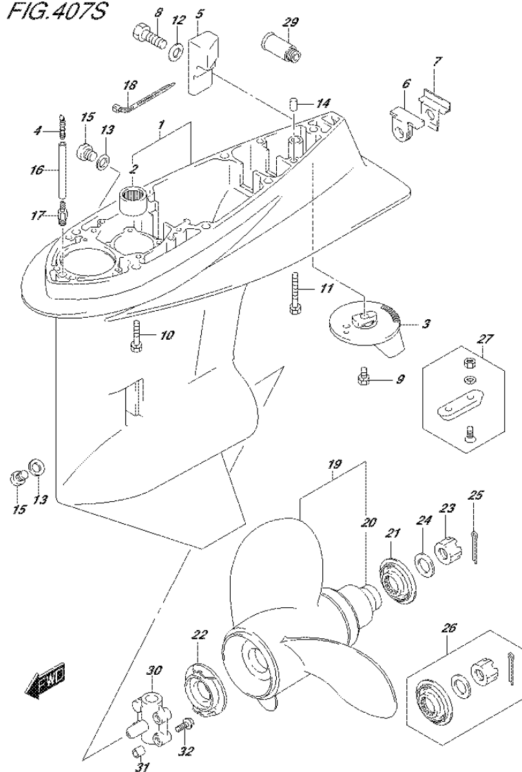
FIG.407S (3-K-4) GEAR CASE (DF60AVT E40)
