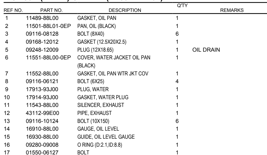
FIG.180N (2-B-11) OIL PAN (DF50AVT E01)
