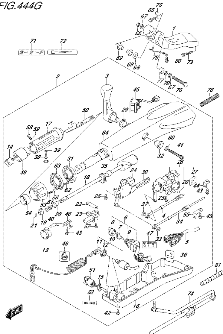
FIG.444G (4-E-8) TILLER HANDLE (DF60ATH E40)
