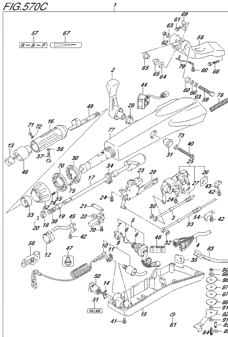
FIG.570C (5-D-6) OPT:TILLER HANDLE (DF50A E01)
