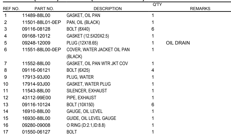
FIG.180T (2-B-15) OIL PAN (DF60AVTH E01)
