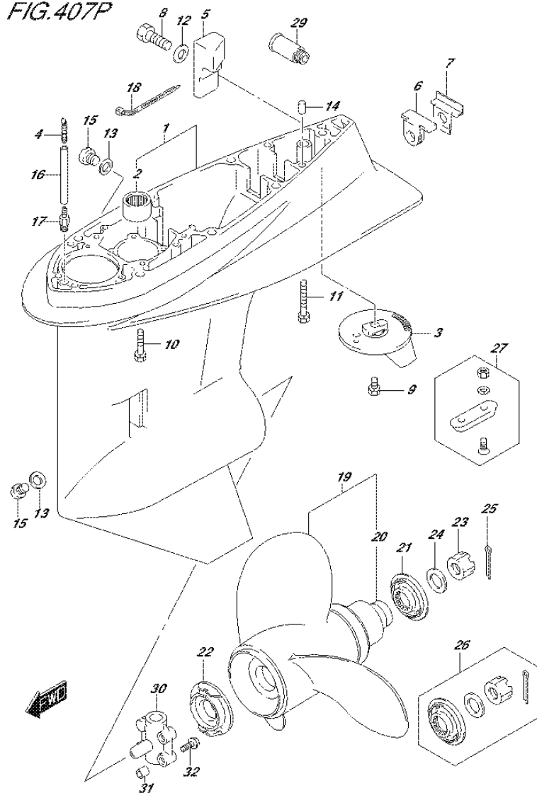
FIG.407P (3-J-14) GEAR CASE (DF50AVTH E01)
