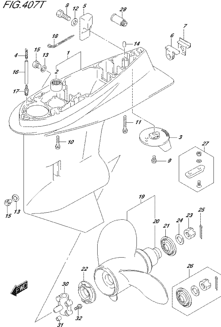
FIG.407T (3-K-6) GEAR CASE (DF60AVTH E01)
