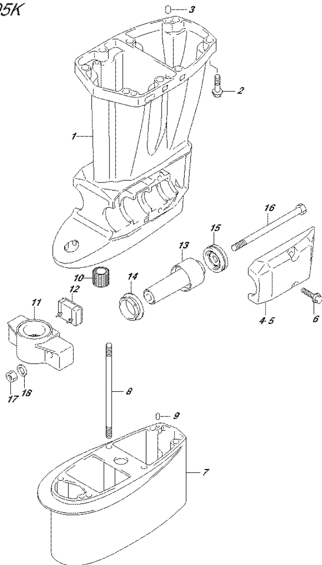
FIG.405K (3-H-6) DRIVE SHAFT HOUSING (DF60AQH E40)
