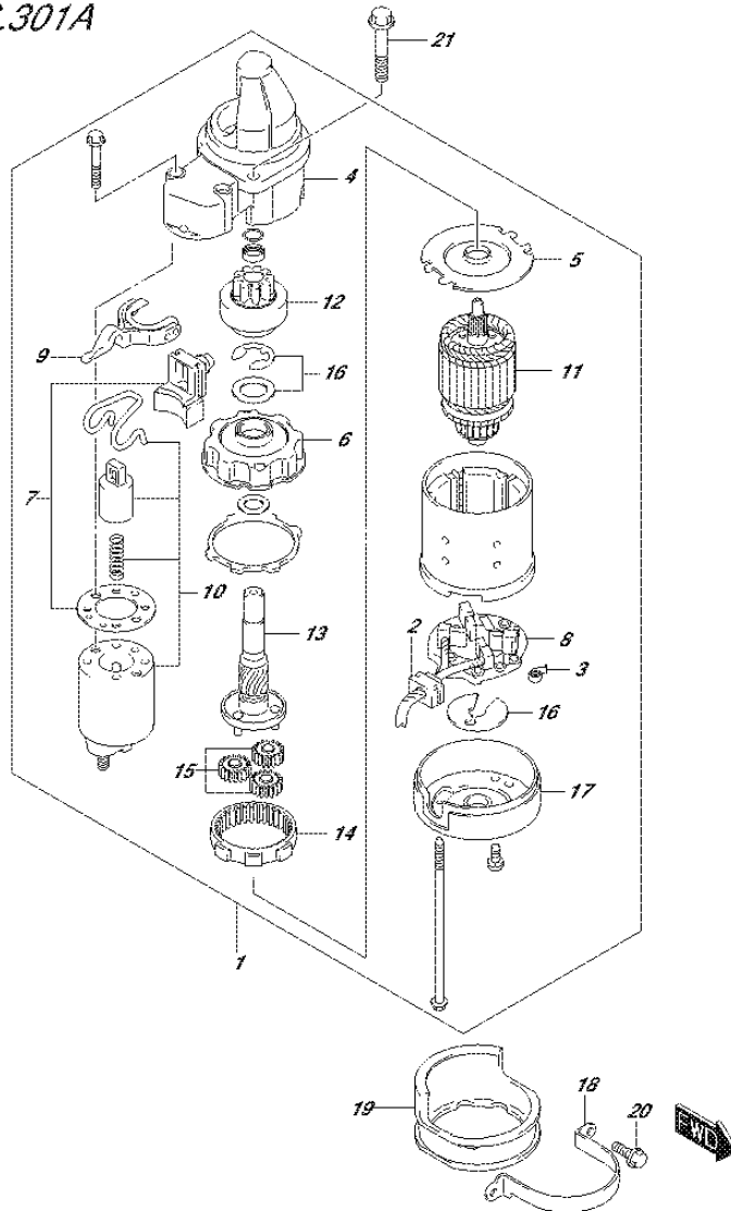
FIG.301A (2-H-5) STARTING MOTOR
