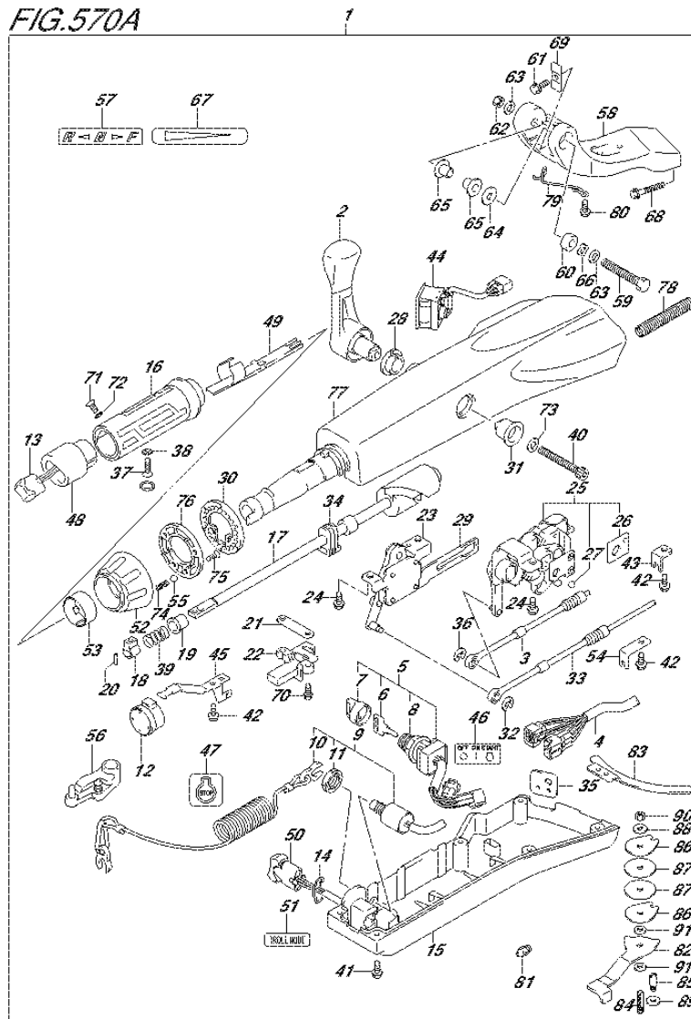
FIG.570A (5-C-13) OPT:TILLER HANDLE (DF40A E01)
