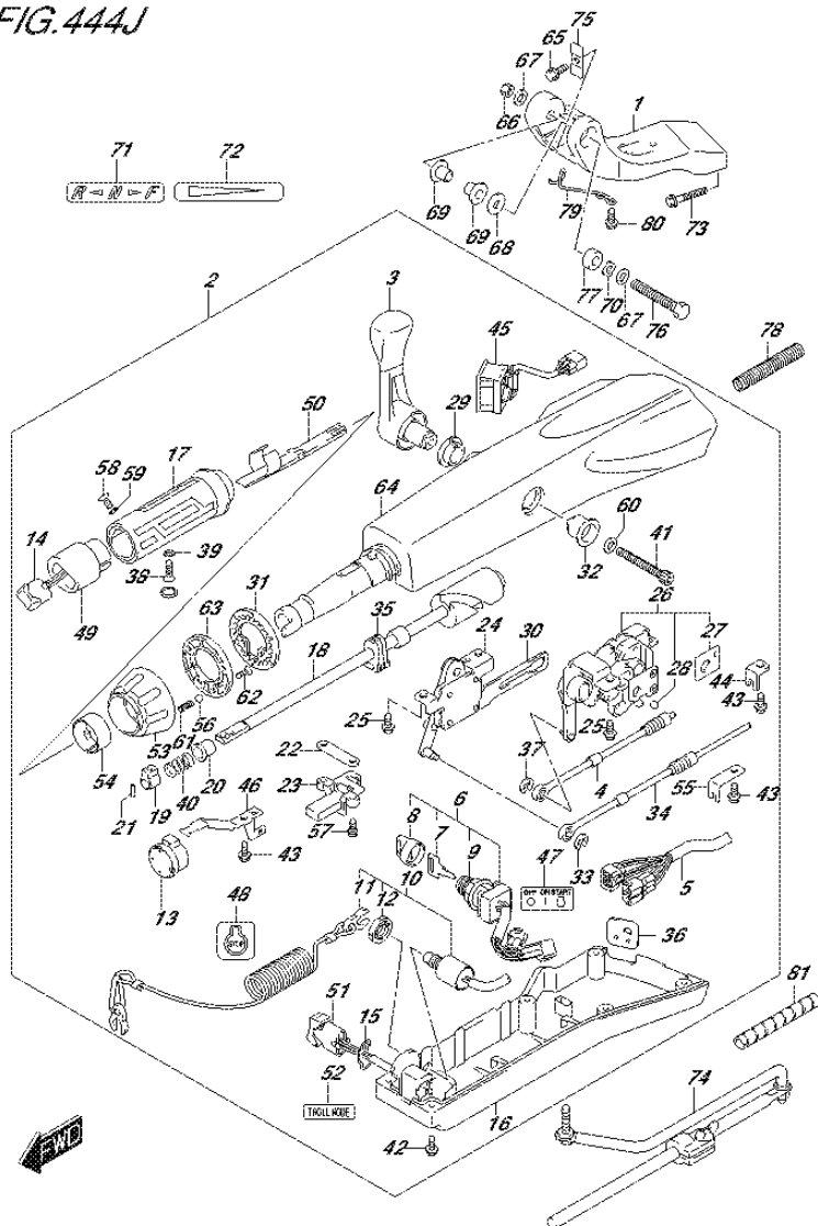
FIG.444J (4-E-14) TILLER HANDLE (DF60AVTH E01)
