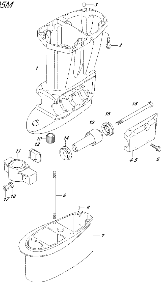
FIG.405M (3-H-8) DRIVE SHAFT HOUSING (DF60ATH E40)
