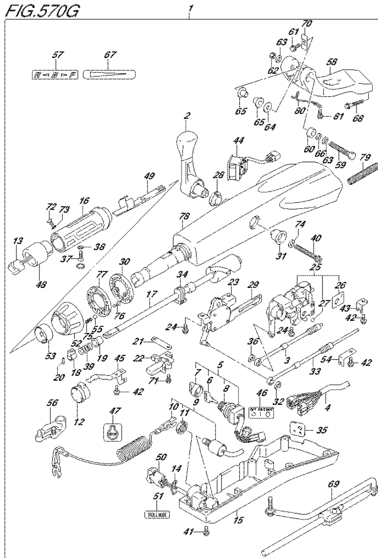
FIG.570G (5-E-4) OPT:TILLER HANDLE (DF60AVT E01)
