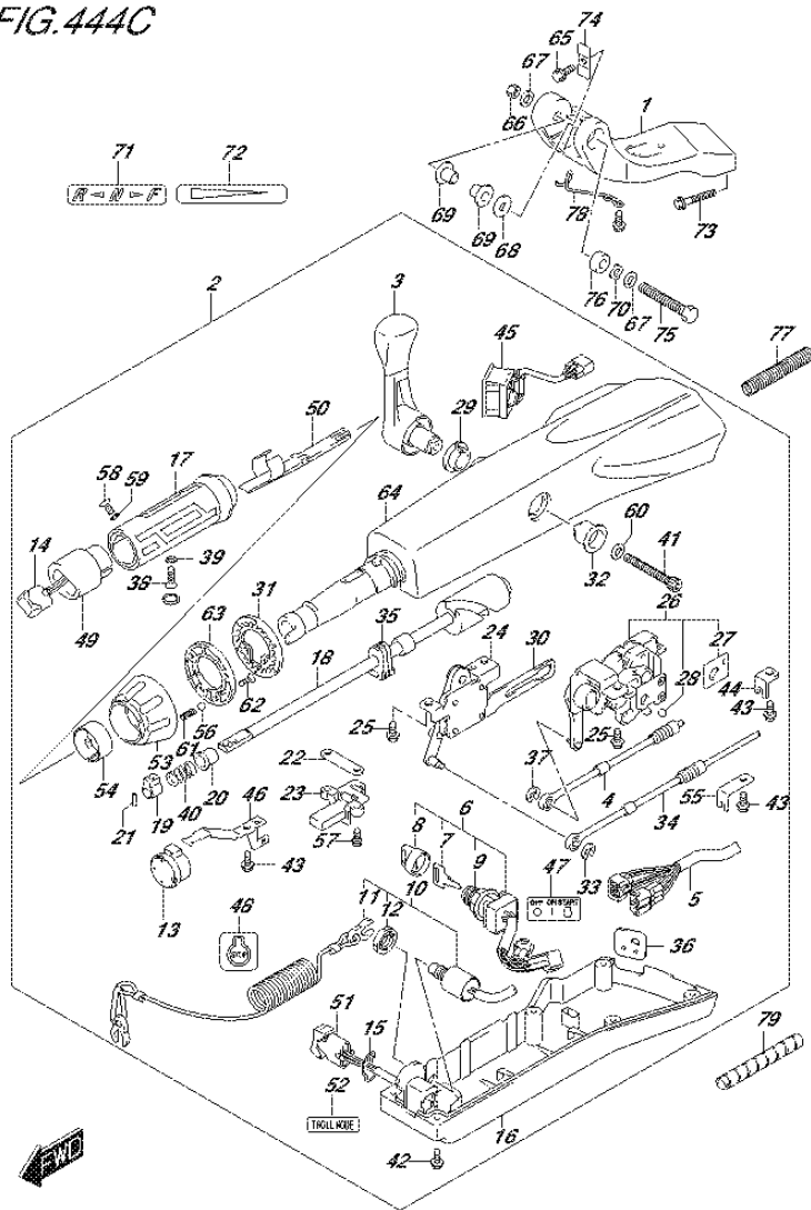
FIG.444C (4-D-8) TILLER HANDLE (DF50ATH E01)
