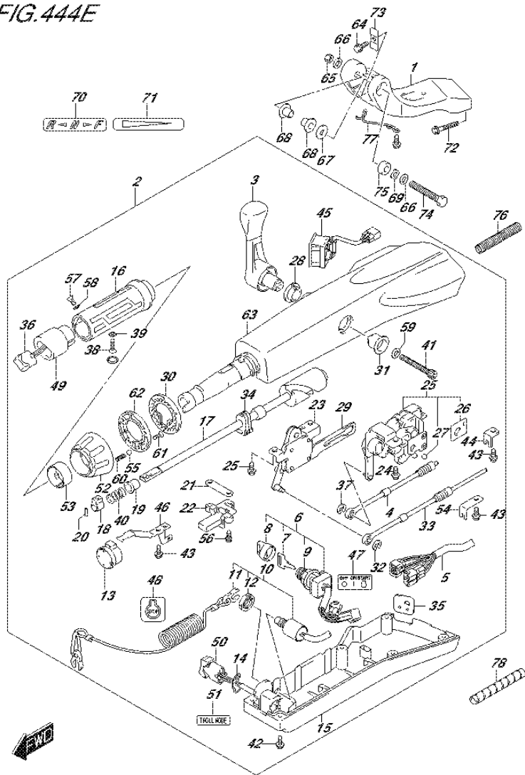
FIG.444E (4-E-2) TILLER HANDLE (DF60AQH E40)
