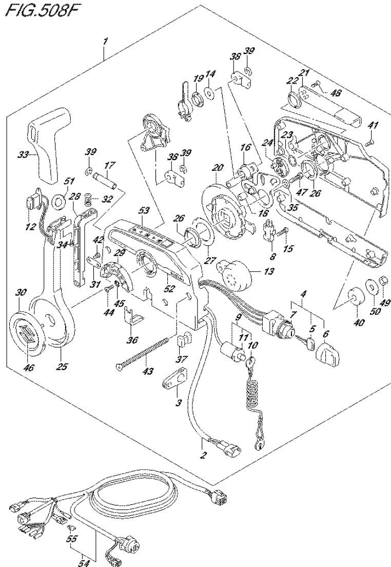
FIG.508F (3-C-6) OPT:REMOTE CONTROL (DF90A E40)
