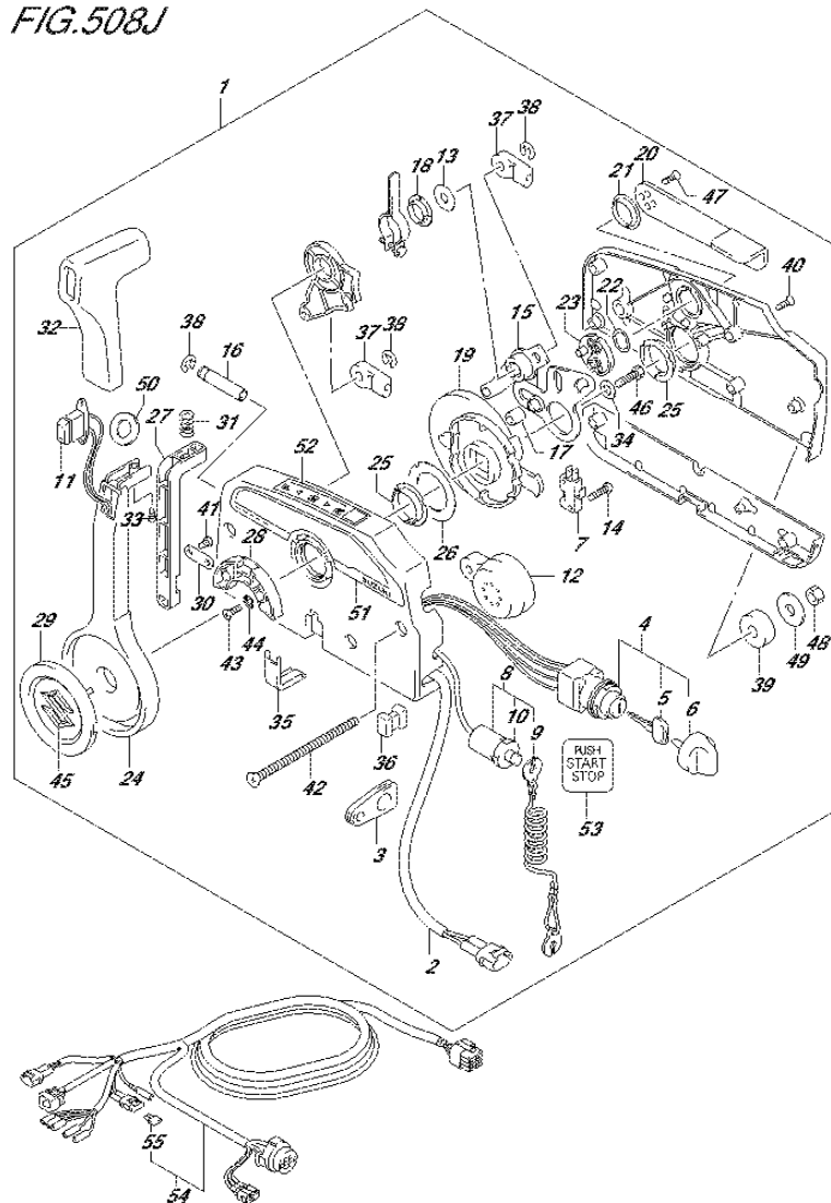
FIG.508J (3-C-12) OPT:REMOTE CONTROL (W/KEY LESS START) (DF90A E01)
