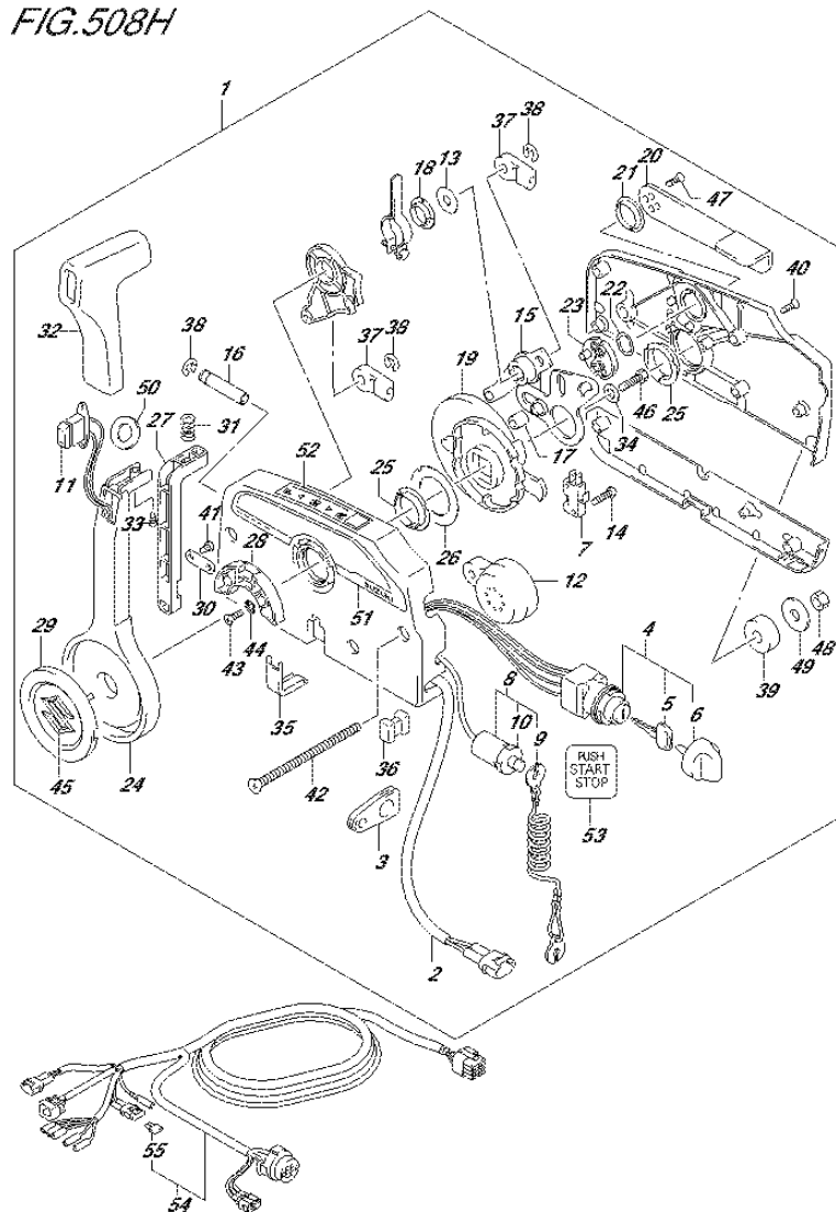
FIG.508H (3-C-10) OPT:REMOTE CONTROL (W/KEY LESS START) (DF80A E01
