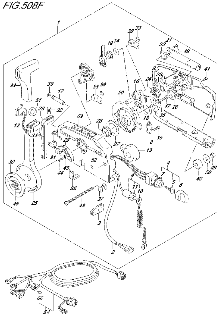
FIG.508F (3-C-5) OPT:REMOTE CONTROL (DF90A E40)
