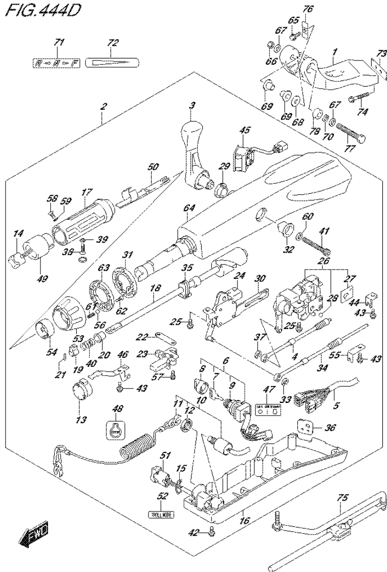
FIG.444D (2-J-7) TILLER HANDLE (DF90ATH E40)
