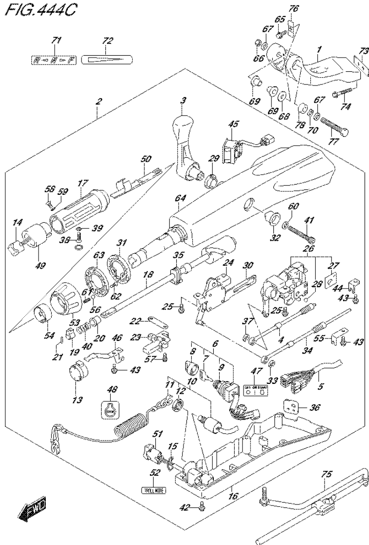
FIG.444C (2-J-4) TILLER HANDLE (DF90ATH E01)
