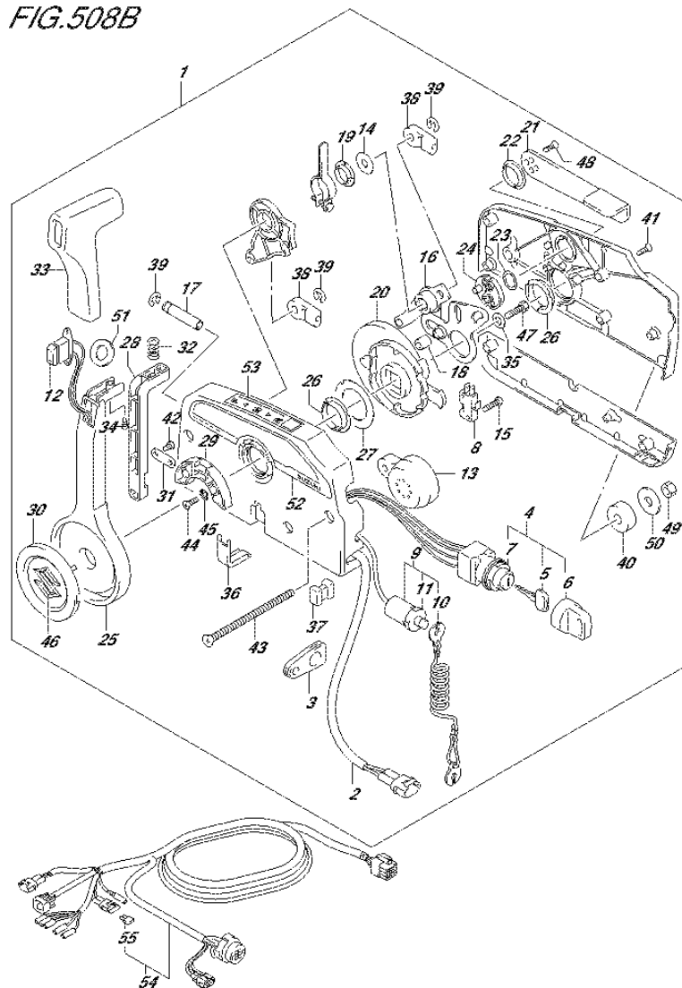
FIG.508B (3-B-12) OPT:REMOTE CONTROL (N/KEY LESS START) (DF80A E01)
