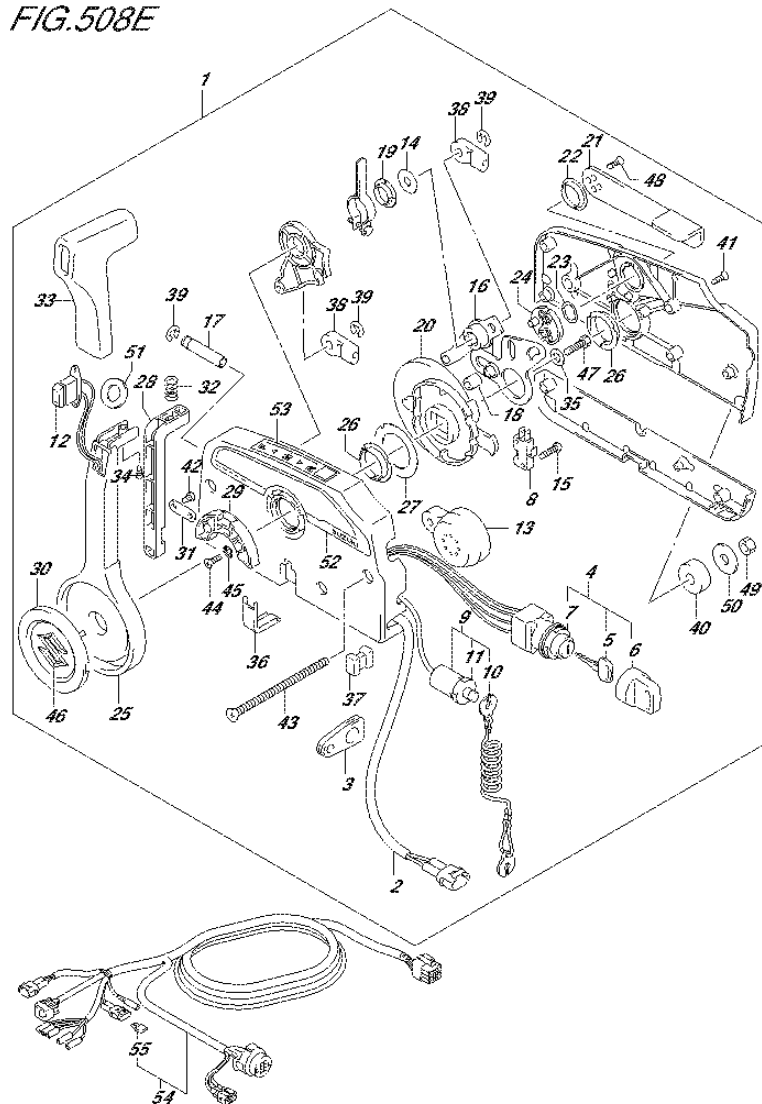
FIG.508E (3-C-3) OPT:REMOTE CONTROL (DF80A E40)
