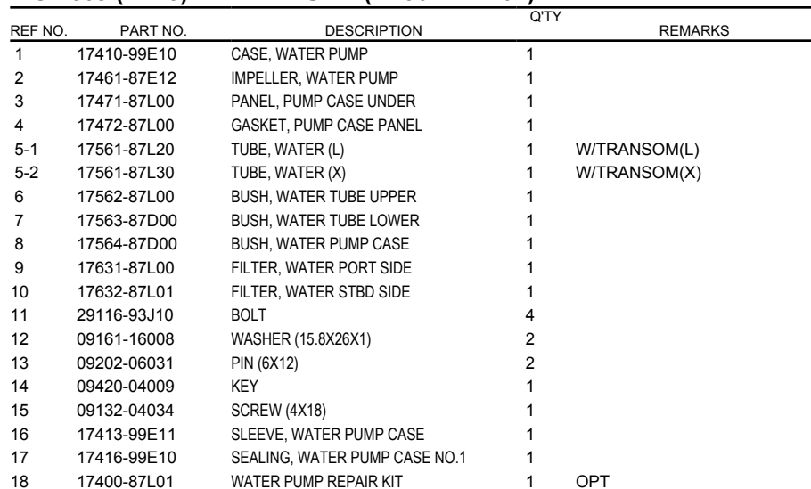
FIG.160J (1-F-3) WATER PUMP (DF90ATH E01)
