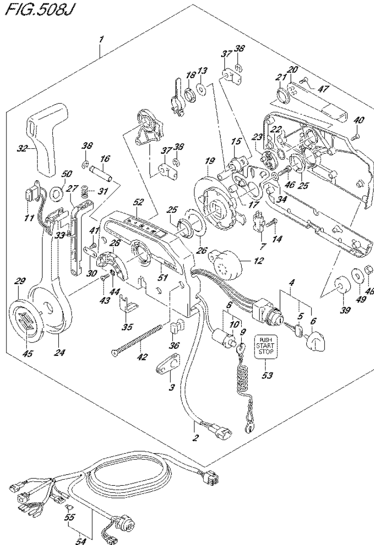
FIG.508J (3-C-11) OPT:REMOTE CONTROL (W/KEY LESS START) (DF90A E01)
