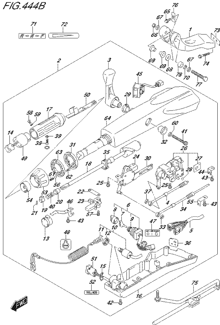
FIG.444B (2-I-15) TILLER HANDLE (DF70ATH E40)
