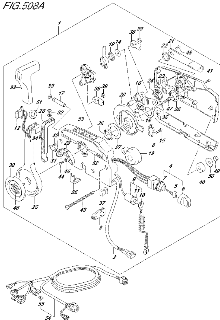
FIG.508A (3-B-9) OPT:REMOTE CONTROL (N/KEY LESS START) (DF70A E01)
