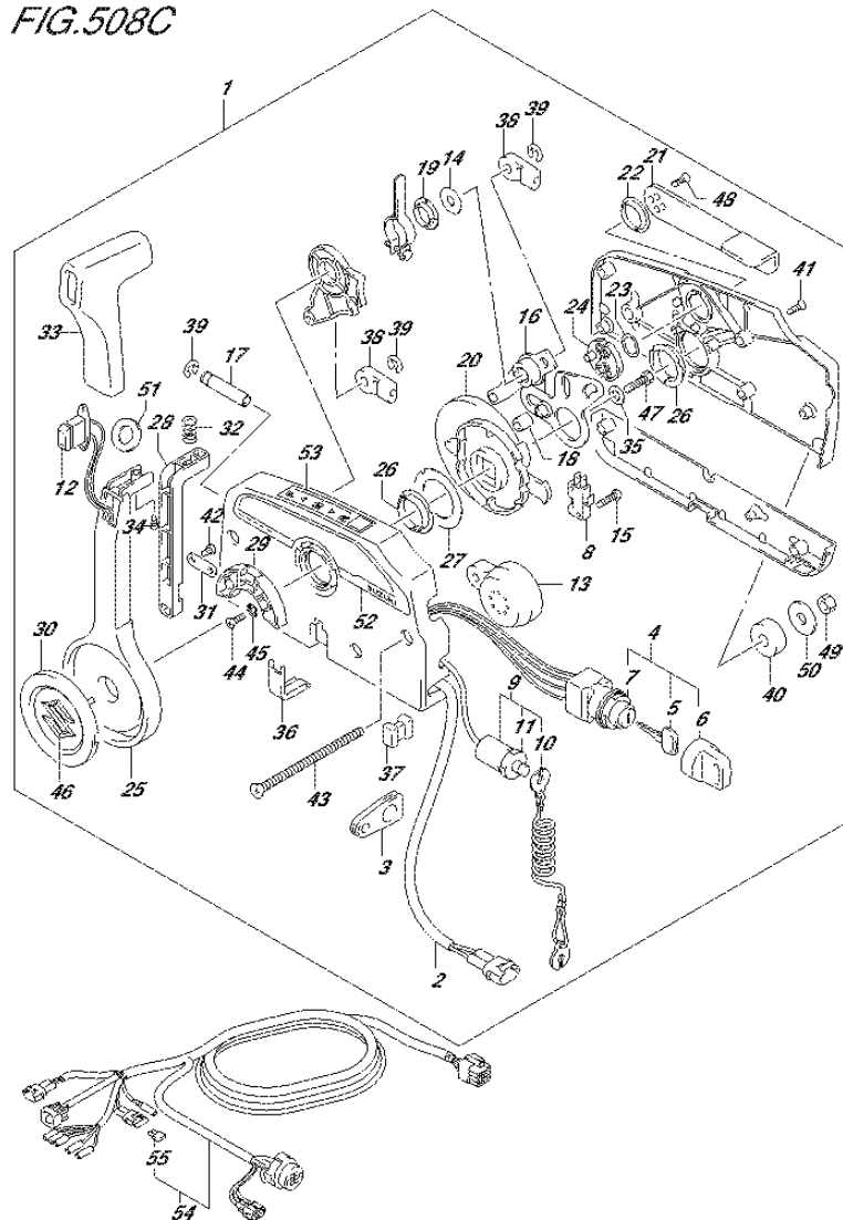
FIG.508C (3-B-13) OPT:REMOTE CONTROL (N/KEY LESS START) (DF90A E01)
