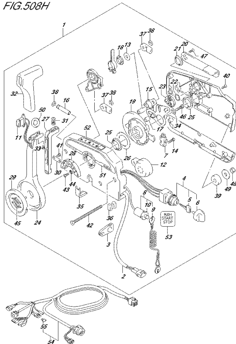
FIG.508H (3-C-9) OPT:REMOTE CONTROL (W/KEY LESS START) (DF80A E01)
