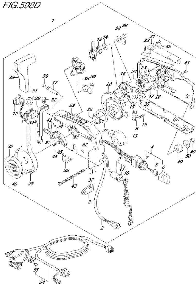
FIG.508D (3-C-2) OPT:REMOTE CONTROL (DF70A E40)
