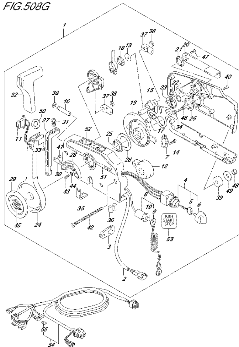
FIG.508G (3-C-7) OPT:REMOTE CONTROL (W/KEY LESS START) (DF70A E01)
