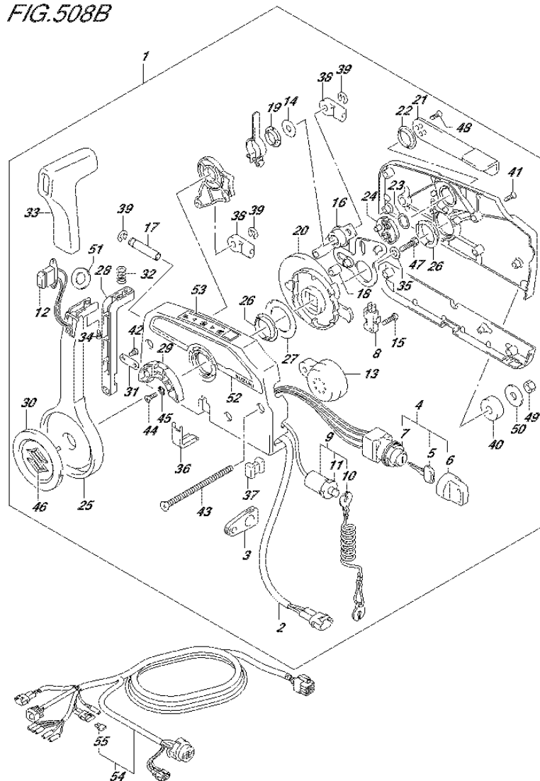
FIG.508B (3-B-11) OPT:REMOTE CONTROL (N/KEY LESS START) (DF80A E01)
