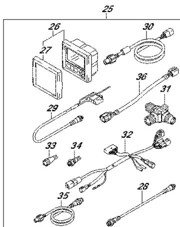
FIG.503A (2-L-2) OPT:METER (2)
