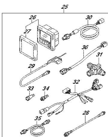
FIG.503A (2-L-3) OPT:METER (2)
