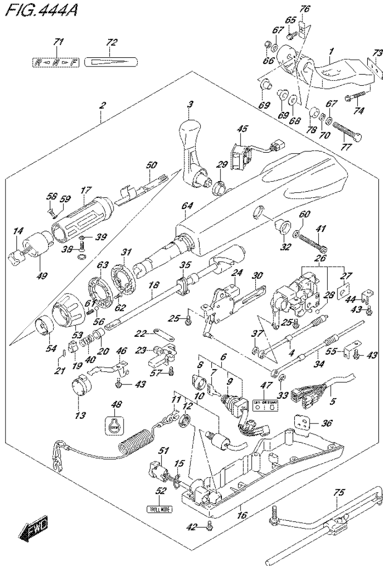
FIG.444A (2-I-6) TILLER HANDLE (DF70ATH E01)
