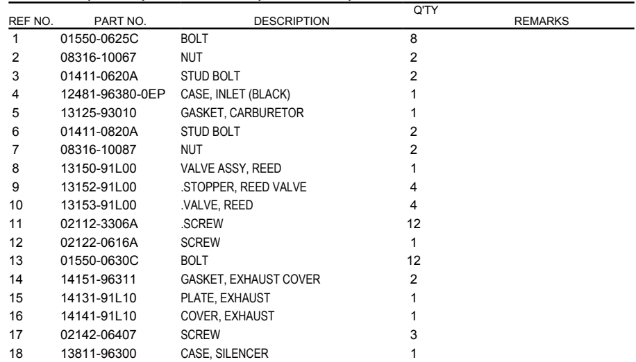
FIG.125C (1-B-10) INLET CASE (DT30R P40)
