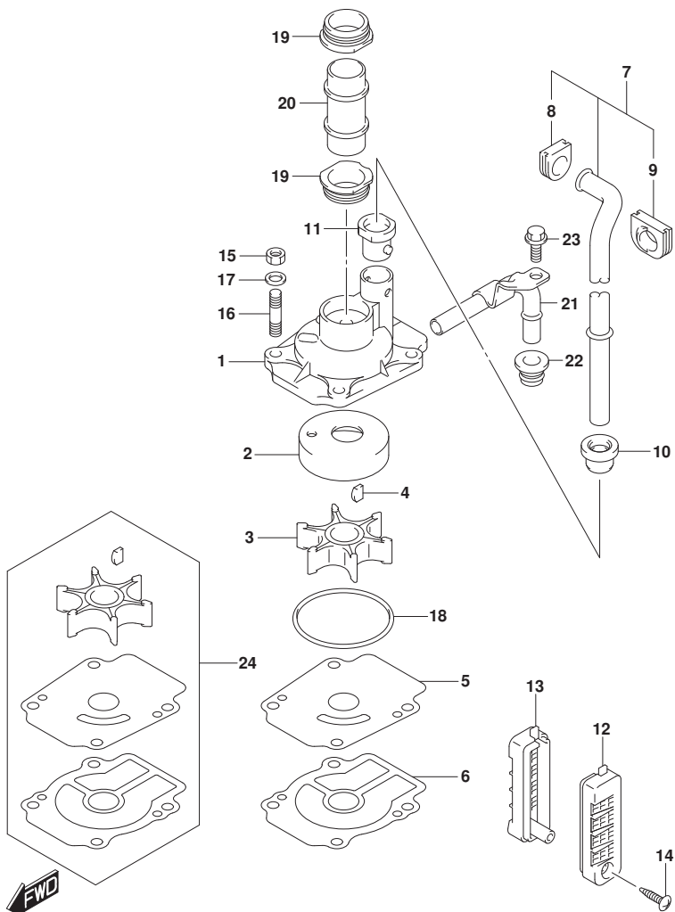
DT25_30_P40_017_160A WATER PUMP
