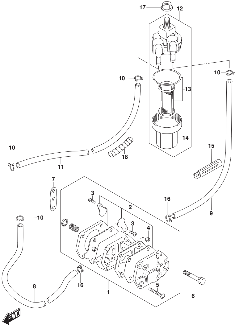
DT25_30_P40_017_146C FUEL PUMP
