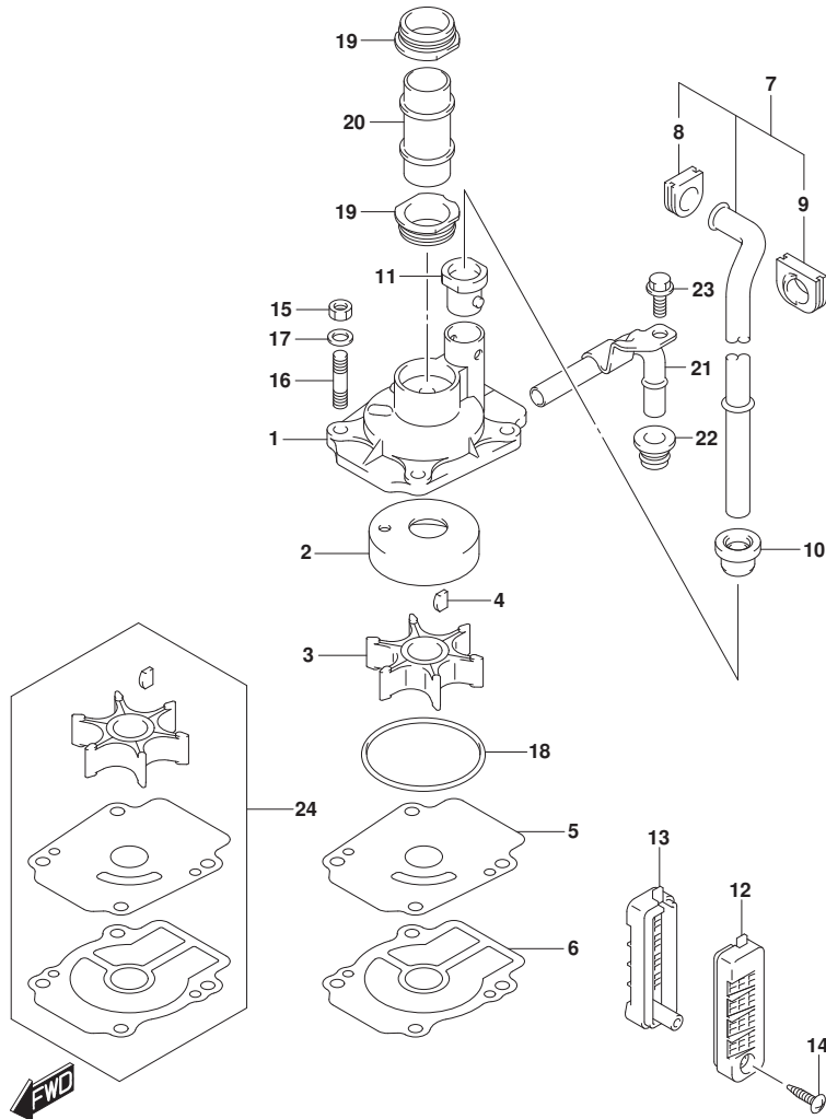
DT25_30_P40_017_160C WATER PUMP
