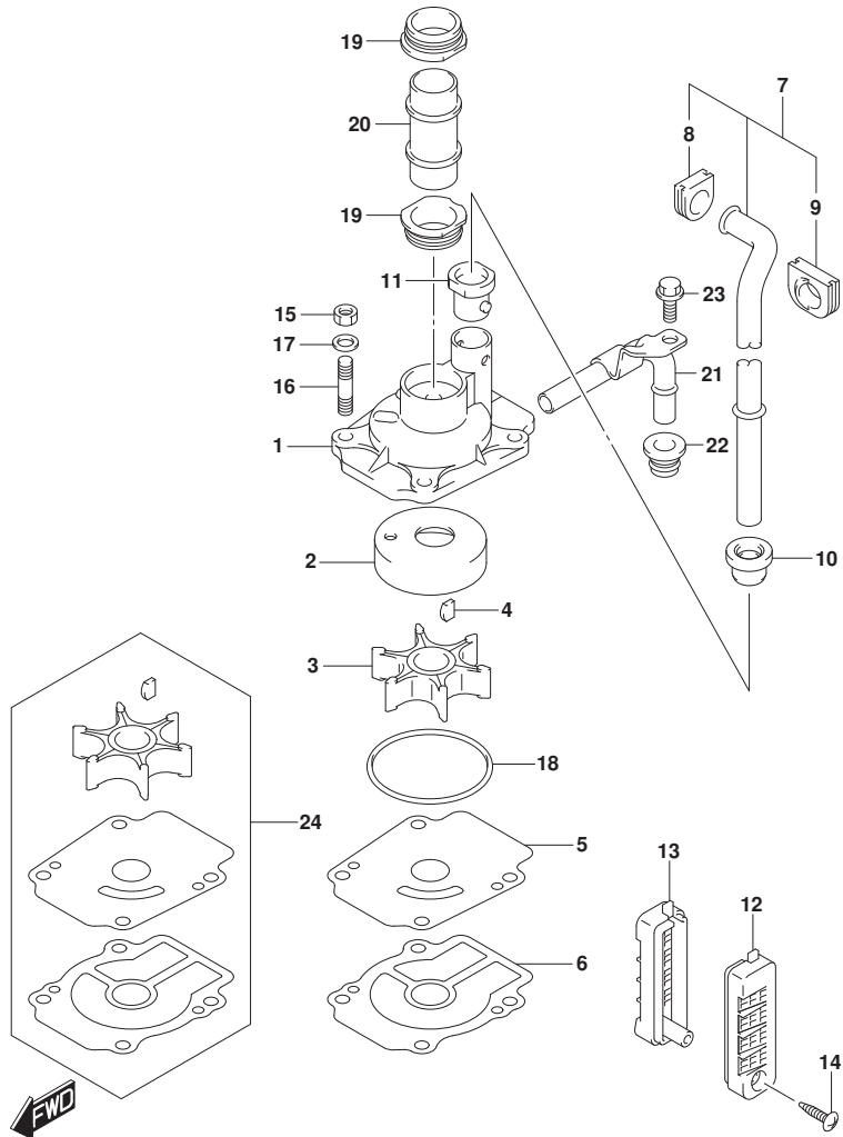
DT25_30_P40_017_160E WATER PUMP
