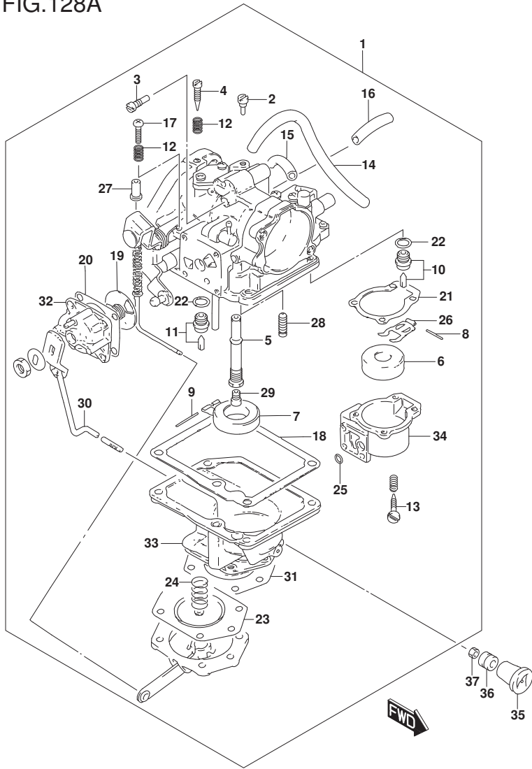
DT25_30_P40_017_128A CARBURETOR
