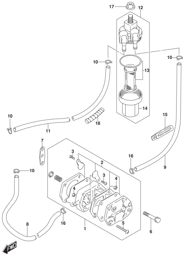
DT25_30_P40_017_146B FUEL PUMP
