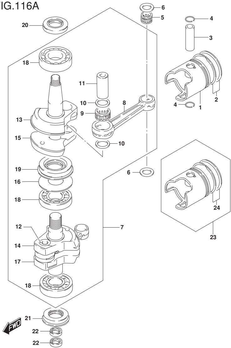
FIG.116A (1-B-4) CRANKSHAFT (DT25K)
