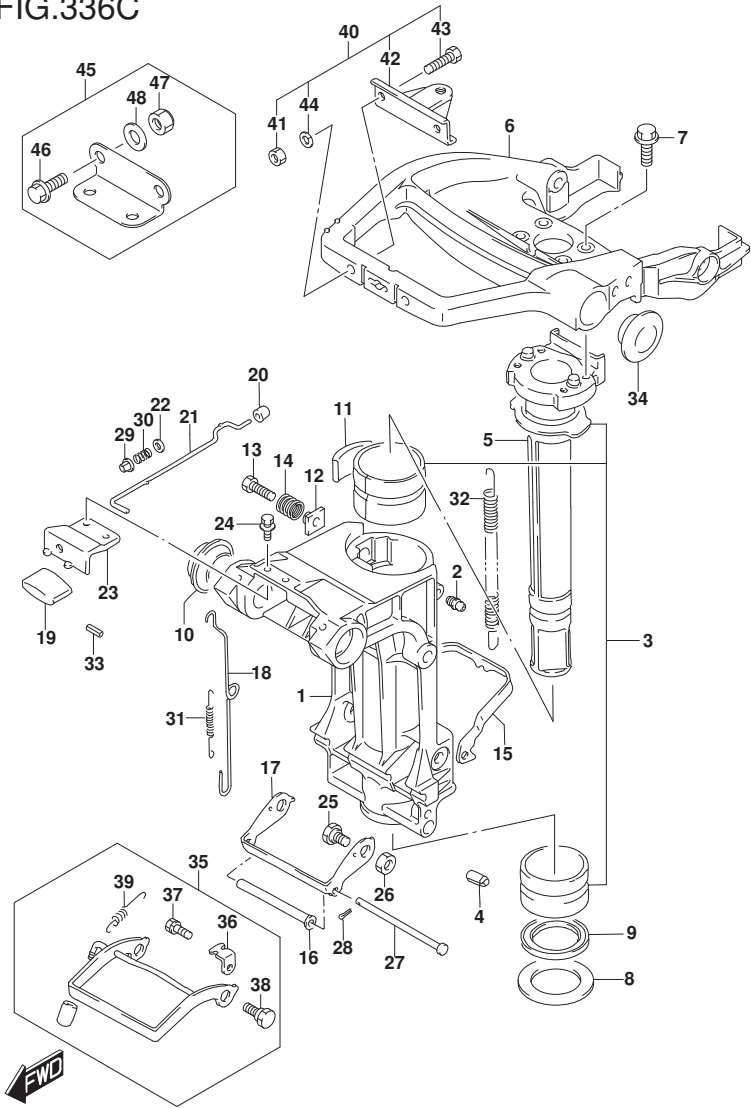
DT25_30_P40_019_336C SWIVEL BRACKET
