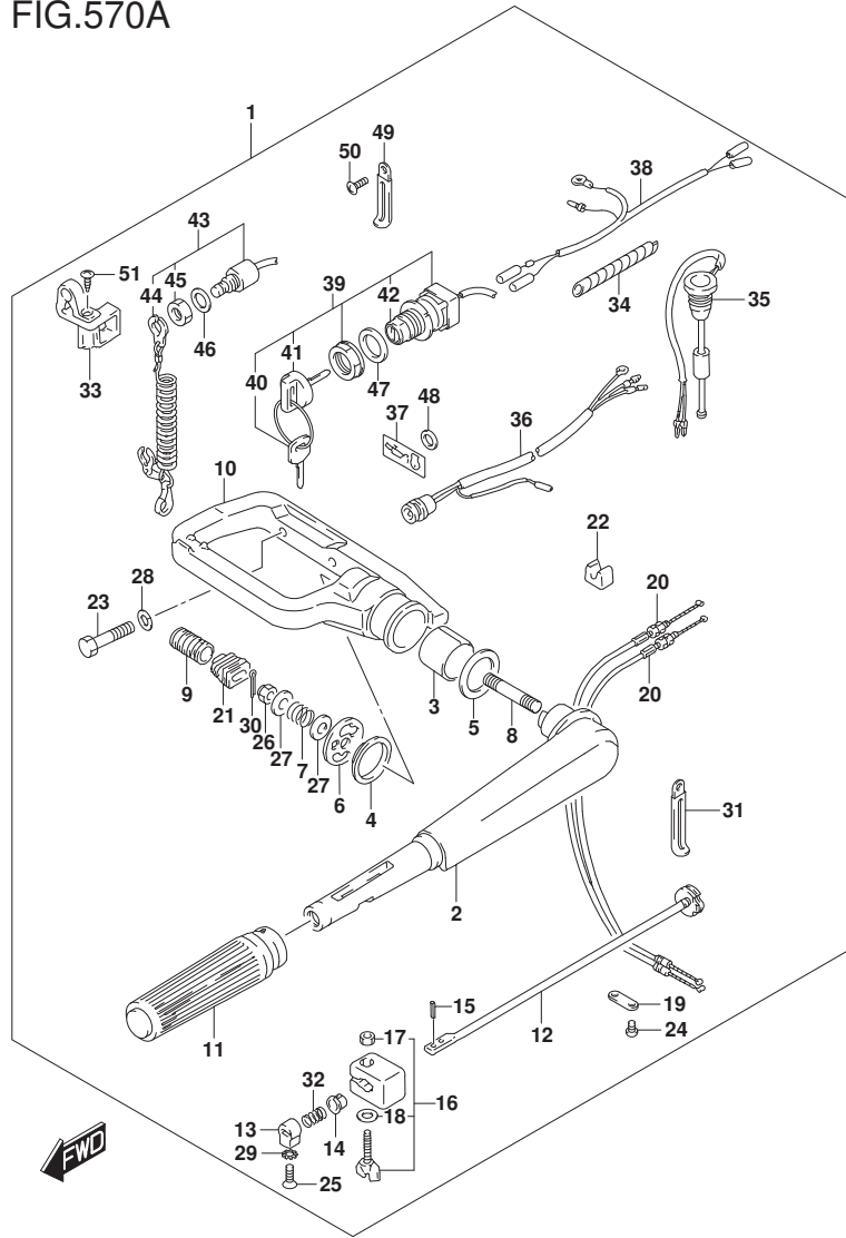
FIG.570A (1-G-13) OPT:TILLER HANDLE (DT40WR)
