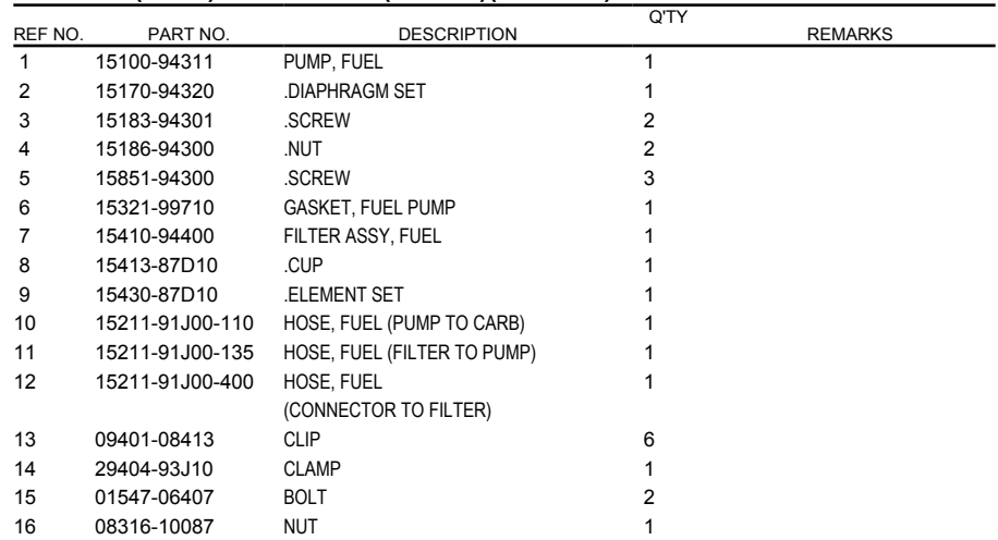
FIG.146A (1-C-4) FUEL PUMP (DT40W)(DT40WR)
