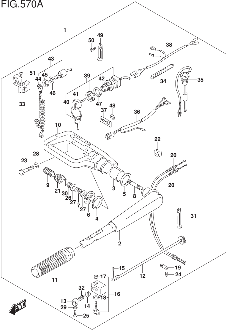
DT40W_P40_019_570A OPT:TILLER HANDLE
