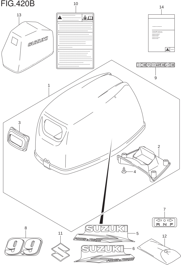
FIG.420B (1-H-12) ENGINE COVER (DT9.9AK P40)
