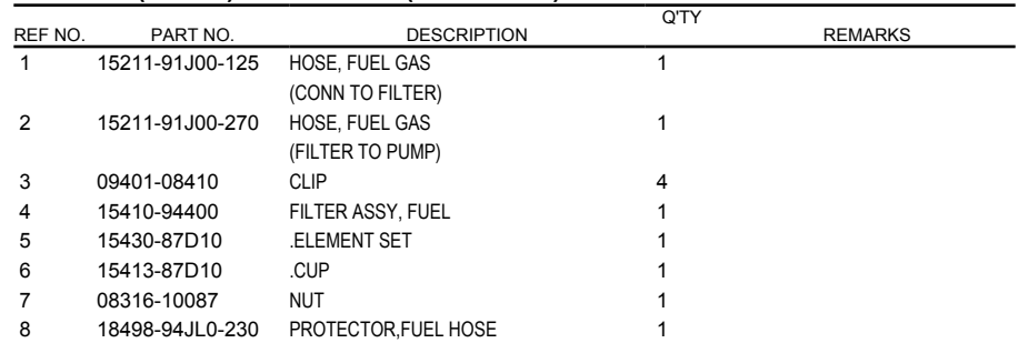
FIG.146D (1-C-13) FUEL PUMP (DT15A P40)
