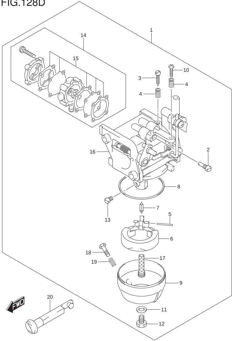
DT9.9A_15A_P40_014_128D CARBURETOR
