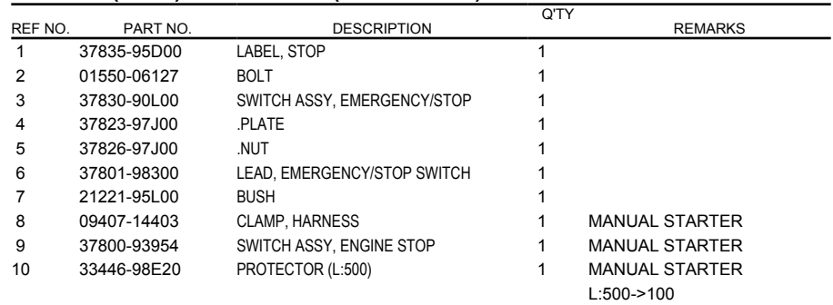
FIG.319B (1-G-2) ELECTRICAL (DT9.9AK P40)
