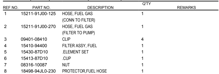
FIG.146A (1-C-10) FUEL PUMP (DT9.9A P40)
