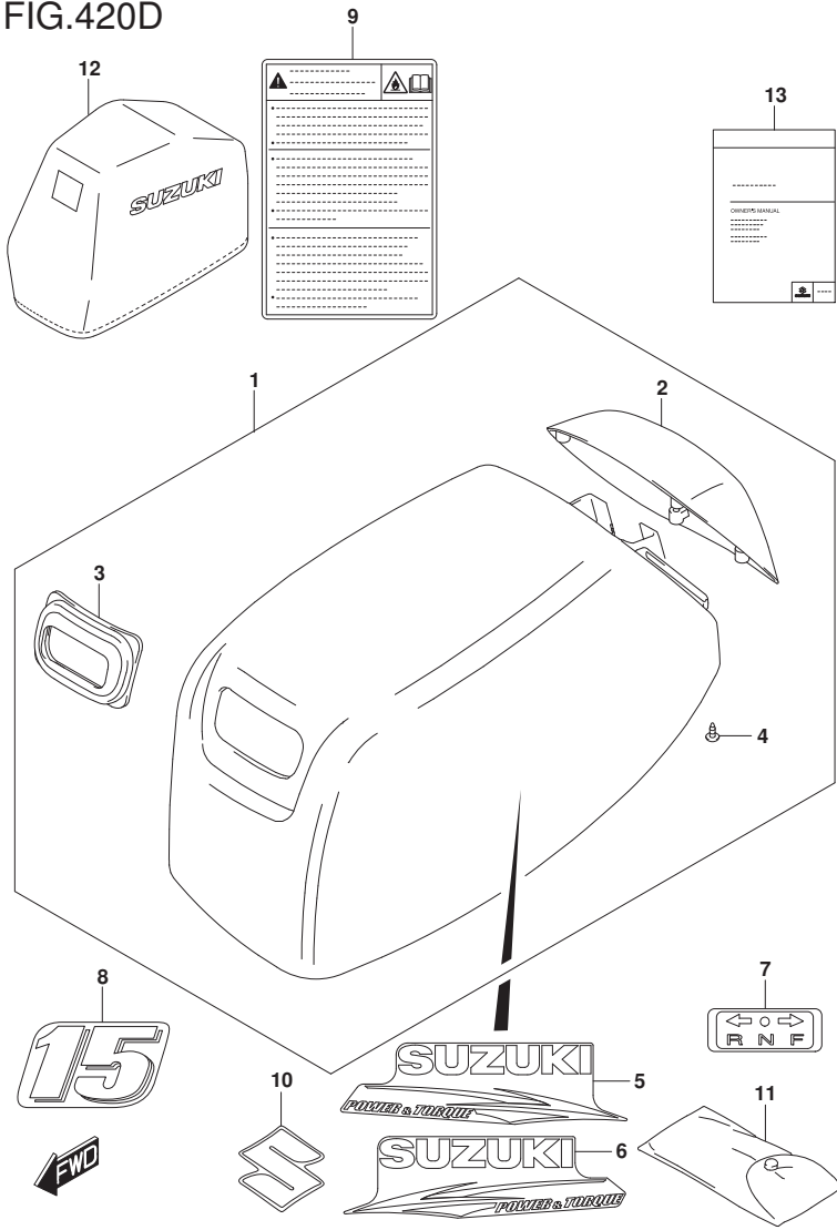
FIG.420D (1-G-5) ENGINE COVER (DT15A P36)(DT15A P81)
