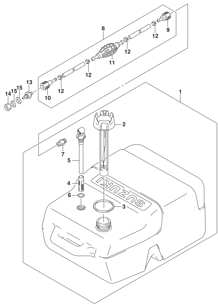
DT9.9A_15A_P40_018_432B FUEL TANK
