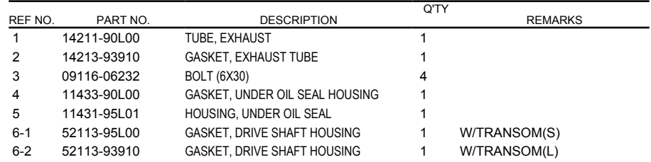
FIG.141B (1-C-4) EXHAUST TUBE (DT9.9A P40)(DT15A P40)
