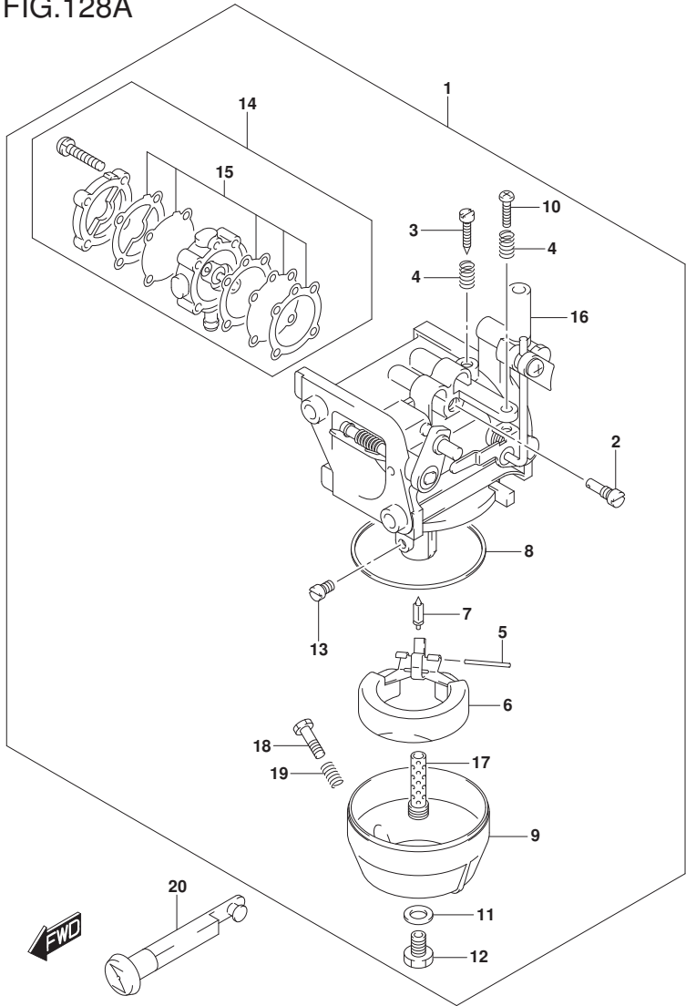
DT9.9A_15A_P40_018_128A CARBURETOR
