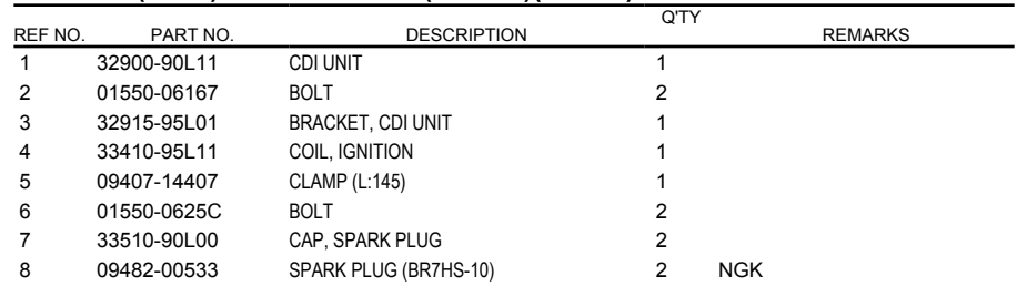
FIG.307A (1-E-4) IGNITION COIL (DT9.9A)(DT15A)
