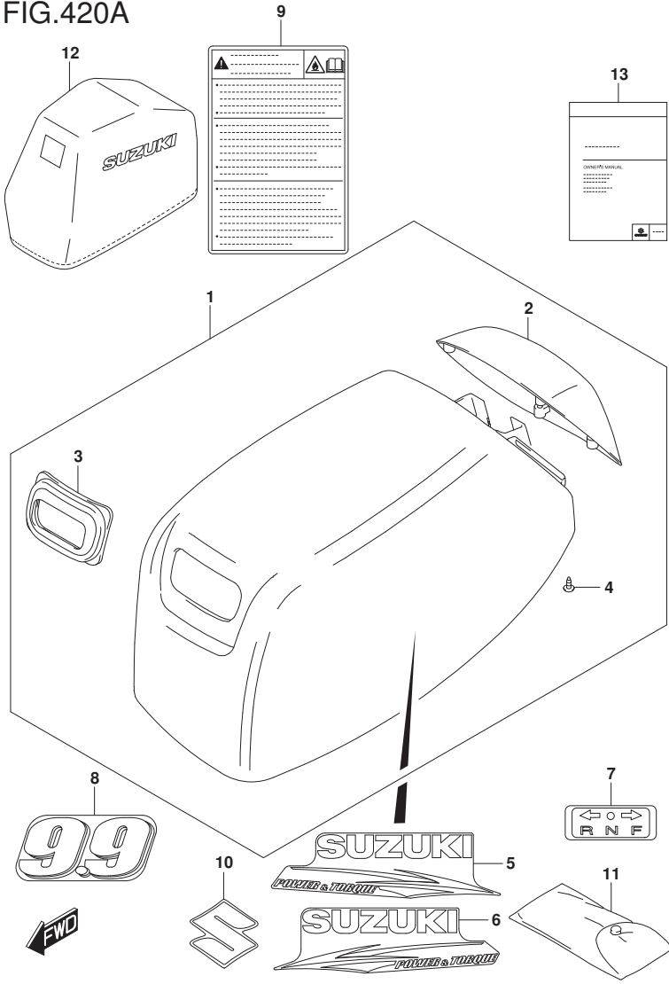
FIG.420A (1-G-2) ENGINE COVER (DT9.9A P36)(DT9.9A P81)
