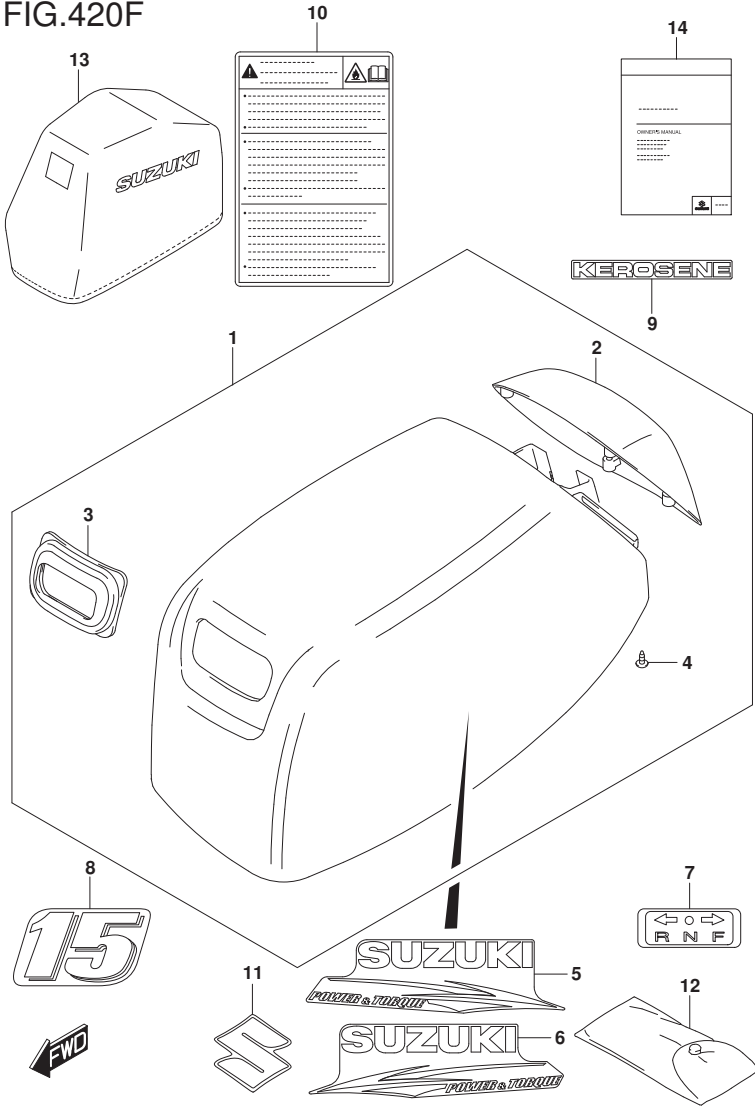
FIG.420F (1-G-7) ENGINE COVER (DT15AK)
