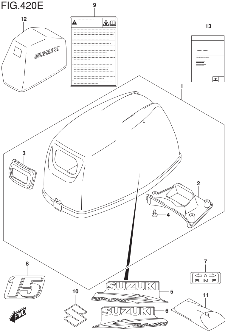
FIG.420E (1-G-6) ENGINE COVER (DT15A P40)
