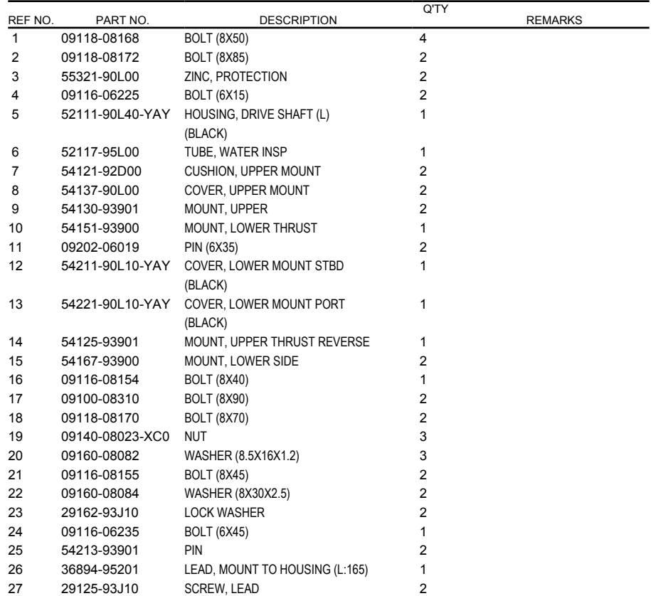
FIG.405B (1-F-5) DRIVE SHAFT HOUSING (DT9.9AK P40)
